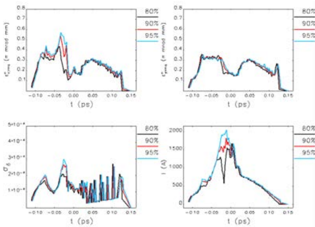
Figure 3.22: Electron beam slice analysis at the entrance of the undulator (Full RF case): x-y transverse emittance (top) and energy spread (bottom left), together with the current profile (bottom right), obtained by selecting different fractions of the beam core according to the core-emittance criterion [25].
