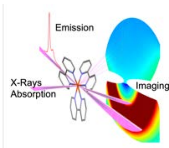
Figure 2.2: Schematics of some complementary X-ray-based techniques, such as spectroscopy and imaging, that could be employed at the new EuPRAXIA@SPARC_LAB. By probing in the ultrafast time domain, these methods enable us to capture the evolving electronic and structural dynamics of molecular systems, solutions, solids, and biosystems, thus providing deeper insights into the nature of dynamical matter. Image adapted from [25].
