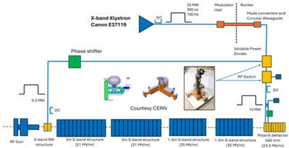
Figure 5.16: Layout for the X-band power distribution taking into account the X-band linearizer and the PolariX Transverse Deflecting Structure [11].
