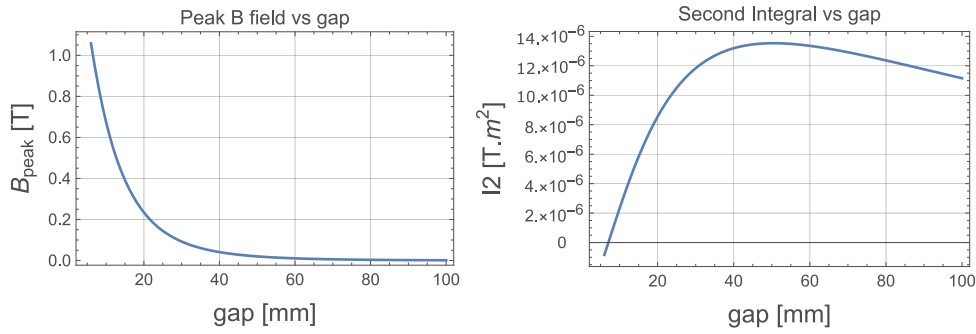
Figure 8.38: Variation of the peak B field and of the second integral with changing phase shifter gap. We do not report the variation of the first integral since it is negligible. Variation of the second integral is anyway within tolerances.
