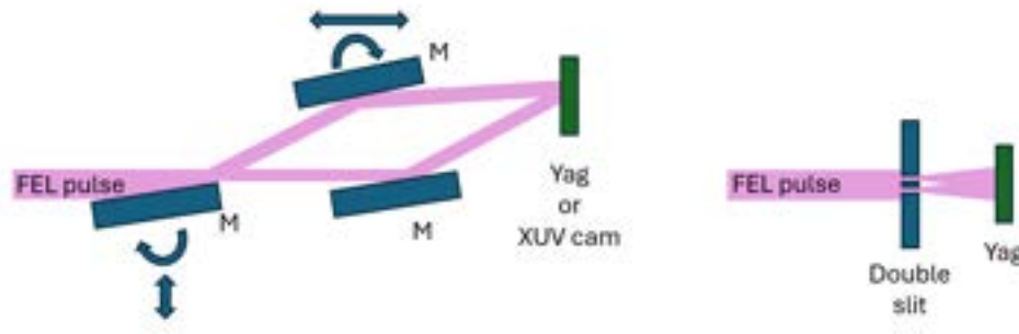
Figure 9.17: Schematic of the two different coherence measurement setups. The FEL pulse is split using a Ni-coated mirror pair for temporal coherence measurement (left), and directed through a variable double-slit apparatus for spatial coherence assessment (right). The recombined or diffracted beams are recorded on XUV-sensitive detectors downstream.
