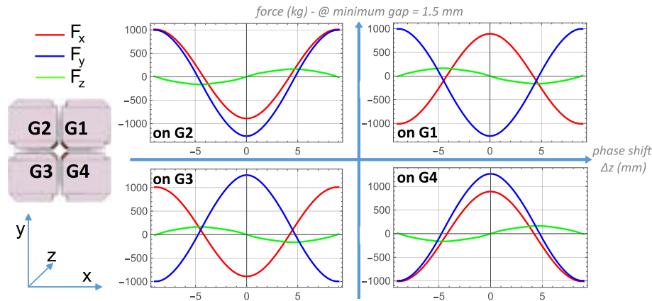
Figure 8.27: Integrated magnetic forces acting on the four undulator girders supporting the magnet arrays (G1, G2, G3, G4). Forces are of the order of 1 ton.
