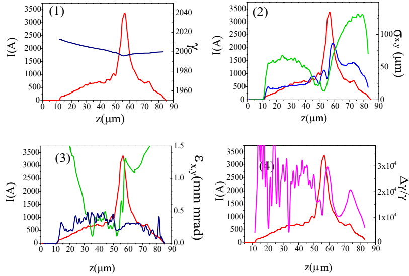
Figure 3.23: Electron beam parameters in the undulator (Full RF case): Beam current (red curve) on the left axis in all the figures as function of z ( \mu\text{m} ) and, on the right vertical axes, (1) Lorentz factor (blue curve), (2) x and y rms dimension (green and light blue, respectively), (3) x and y normalized emittance (green and light blue, respectively), and (4) relative energy spread (magenta).
