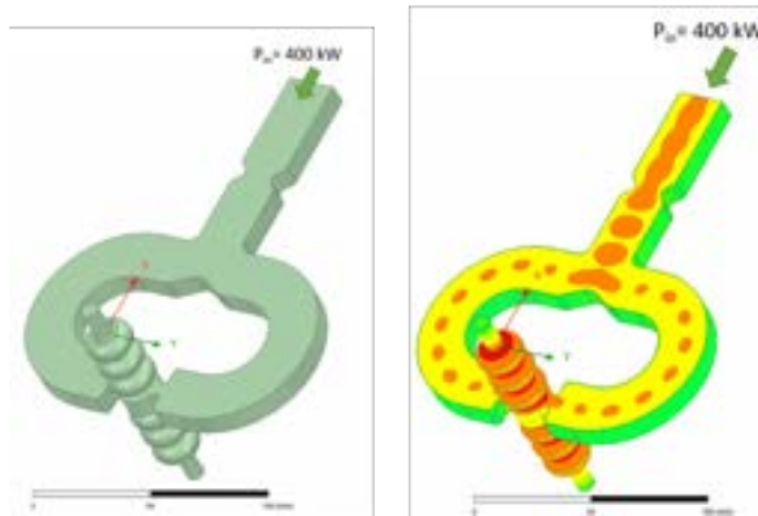
Figure 5.10: Full structure: RF power splitter and X-band cavity. Rendering, left; surface electric field distribution, right.
