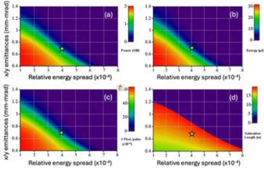
Figure 8.6: As in Fig. 8.5, the four panels represent the dependence of the peak power (a), the pulse energy (b), the number of photons per pulse (c) and the saturation length (d) as functions of both the beam emittances and the energy spread, but with the undulator in linear polarization mode. The yellow star symbol indicate the working point simulated in the beam physics chapter, Tab. 3.1. Note that the simulated working point presents a substantially higher peak current with respect to the conservative value used in this example (3.3-3.4 kA vs 1.5 kA).
