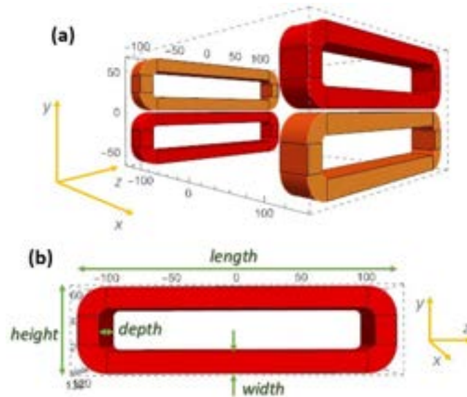
Figure 8.25: (a) Single block of the correction coils system. The horizontal distance from the undulator axis ( x = 0 ) takes reasonably into account the size of the magnets' holders. (b) Scheme and dimensions of the single coil.
