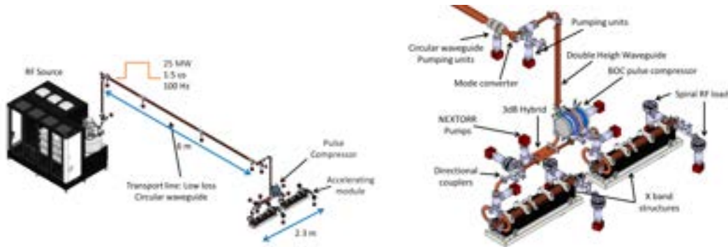
Figure 6.2: X-band RF module mechanical layout.
