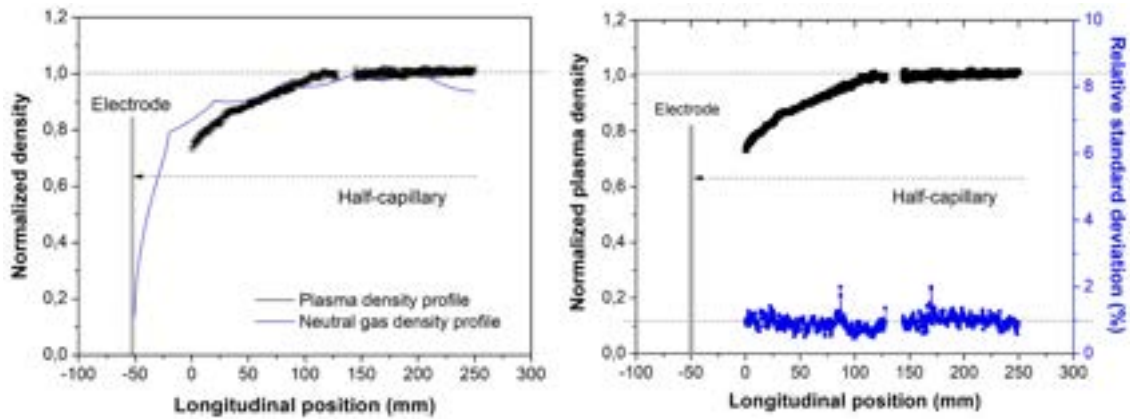
Figure 7.7: Characterization of a 60 cm-long capillary equipped with inlets having an increasing diameter toward the ends. a) Comparison of the longitudinal plasma profile measured using the Stark broadening technique with simulations of the N_2 gas distribution (blue curve in Figure 7.4). b) Longitudinal plasma density and relative standard deviation.
