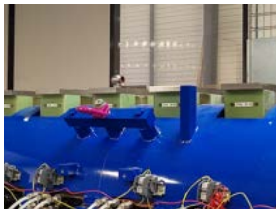
Figure 17.8: The solenoid with the iron shield during the coils alignment
