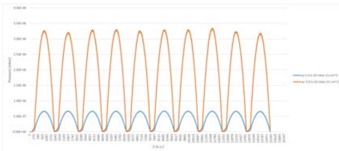
Figure 16.19: Undulators: Simulated pressure distribution along undulator series
