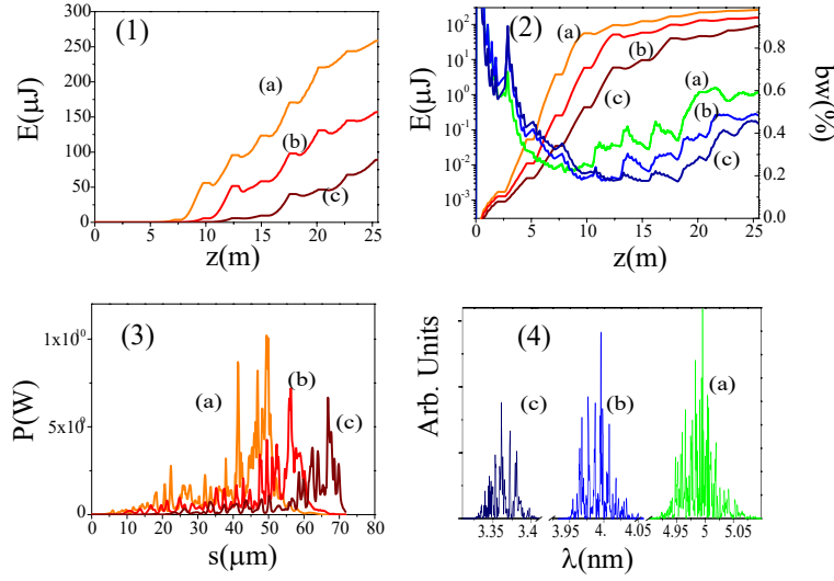
Figure 3.24: FEL simulation results (Full RF case). Case (a) K_{rms} = 1.1 , corresponding to \lambda_r = 4.95 nm, (b) K_{rms} = 0.878 , corresponding to \lambda_r = 4.0 nm and (c) K_{rms} = 0.7 , corresponding to \lambda_r = 3.37 nm. Figure (1): pulse energy growth in linear scale. Figure (2): pulse energy growth in logarithmic scale and bandwidth in %. Figure (3): power distributions at 25 m, ( s = z - 25 m). Figure (4): spectral distributions at 25 m.
