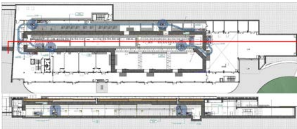
Figure 18.12: Layout and section view for equipment accessibility during maintenance stops.
