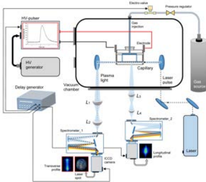
Figure 7.20: Experimental setup installed in the Plasma_lab of the INFN-LNF, used to implement the Stark broadening technique to characterize the gas-filled discharge capillaries.
