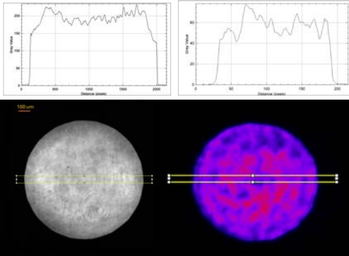
Figure 12.6: Measured transverse profile of the laser beam (IR left, UV right).
