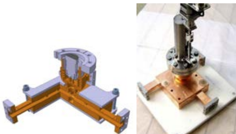
Figure 13.6: Mechanical design and realization of the variable RF power divider.
