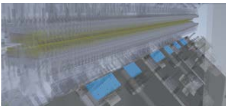
Figure 8.54: Representation of the undulator frame where the areas holding the vacuum chamber are highlighted in blue.
