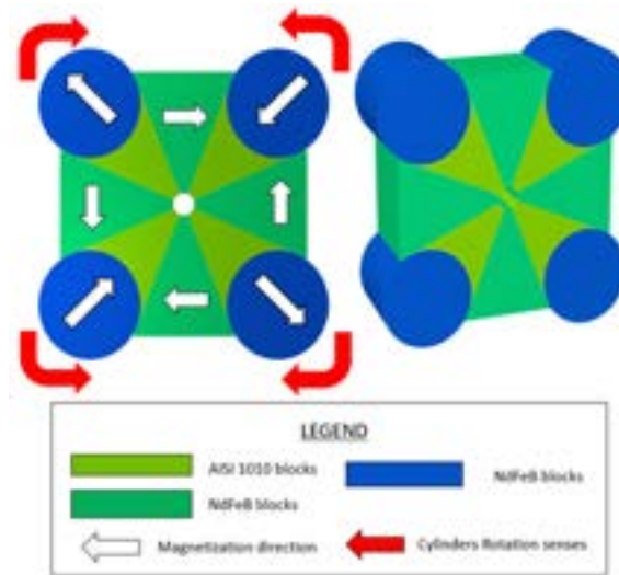
Figure 17.17: 3D front (left) and general (right) views of the TPMQ compact design for the short quadrupole downstream the plasma capillary. Blocks material, magnetization direction and cylinders rotation senses are depicted with colors and symbols of the legend.
