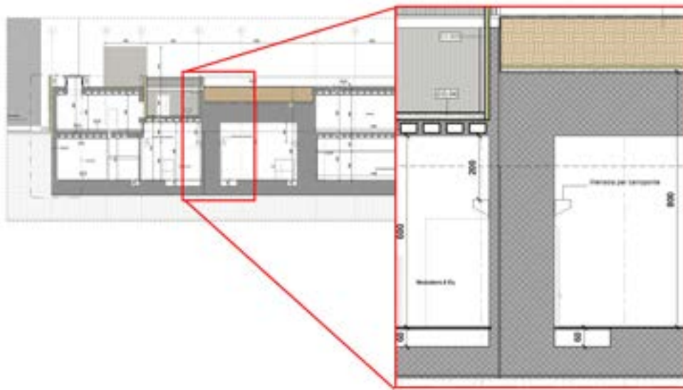
Figure 18.11: EuPRAXIA@SPARC_LAB Building cross section.
