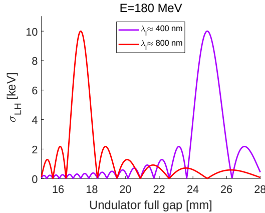
Figure 3.27: Slice energy spread induced by the LH vs undulator full gap (target \sigma_{LH} = 10 keV), for the two possible laser wavelengths, in the case of an electron beam energy of 180 MeV.
