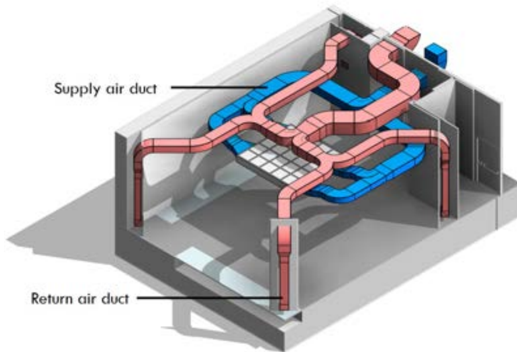
Figure 18.23: CleanRoom ventilation system.
