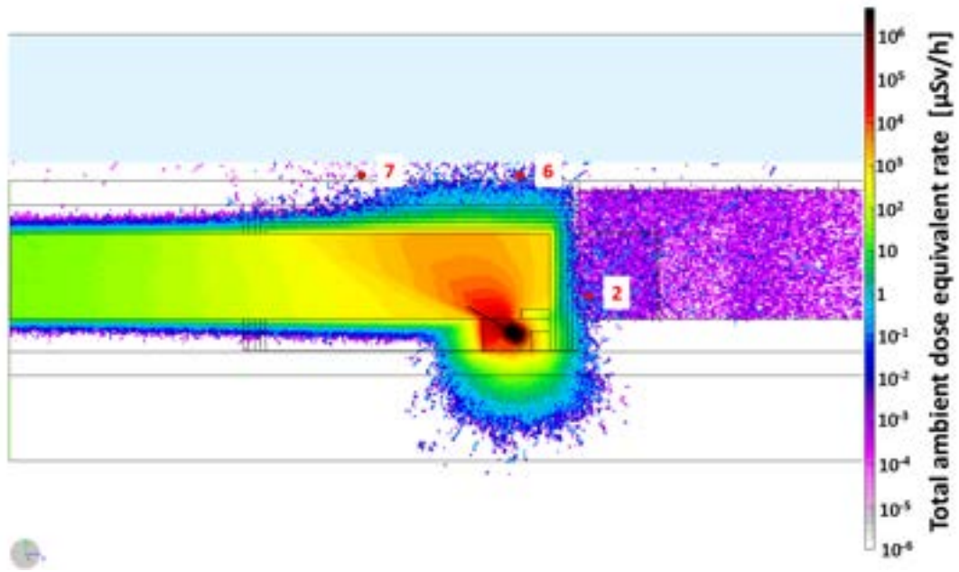
Figure 19.23: H^*(10) - FEL beam dump - without plasma acceleration - yz plane.
