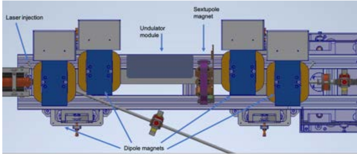
Figure 5.17: Layout of the Laser Heater section.
