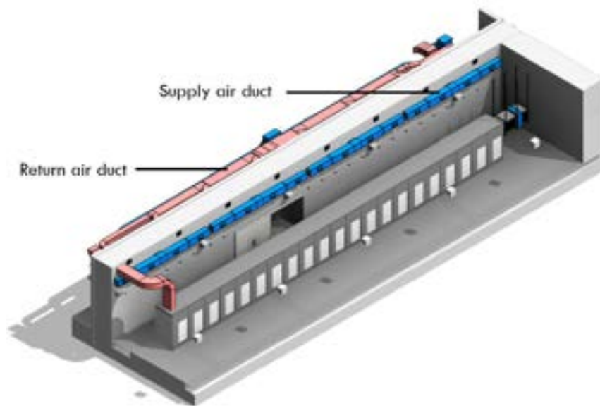
Figure 18.20: Undulators Hall ventilation system.
