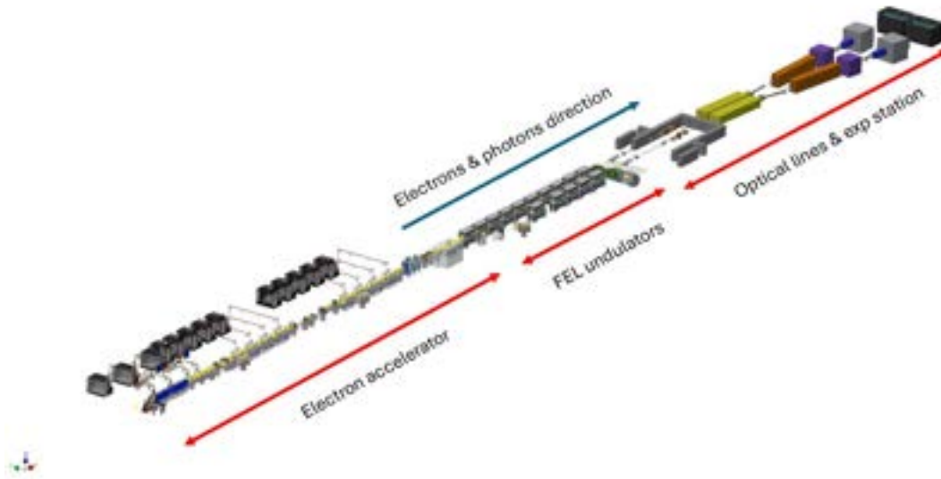
Figure 1.7: Layout of the accelerator and beamlines
