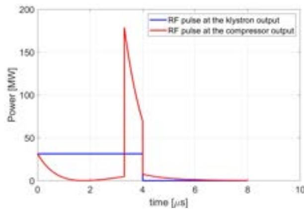
Figure 13.2: Computed RF pulses at the SLED input and output for the 3 m S-band structures.
