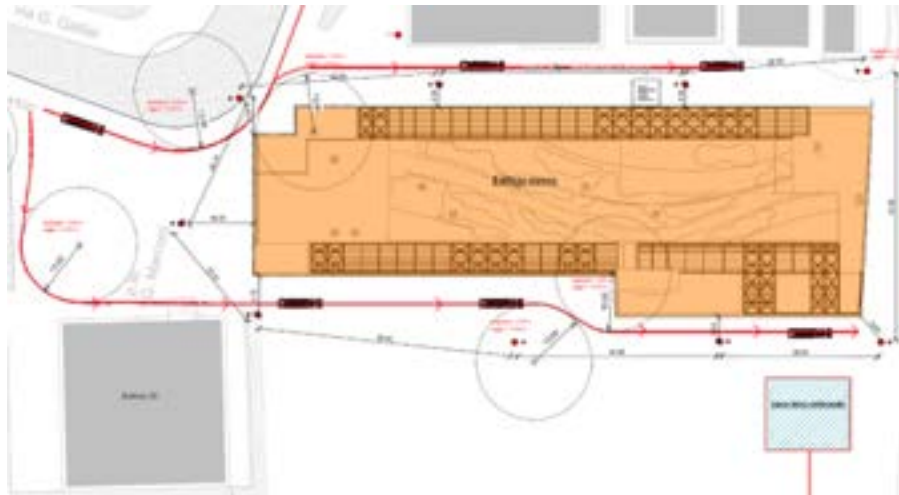
Figure 19.6: Access routes for firefighting vehicles showing single fire pump connection (UNI 70), and pillar-type or underground hydrants (DN70)
