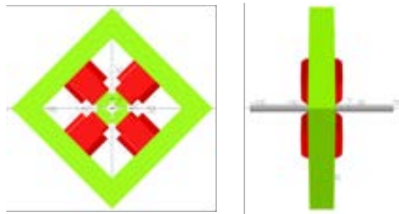
Figure 17.23: The Opera 3D model of the intra-undulators quadrupoles (front and side view).
