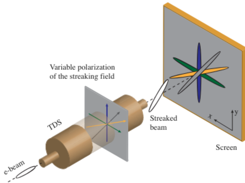
Figure 11.13: Working principle of the PolariX TDS, capable of streaking the beam along different directions by varying the field polarization [25].
