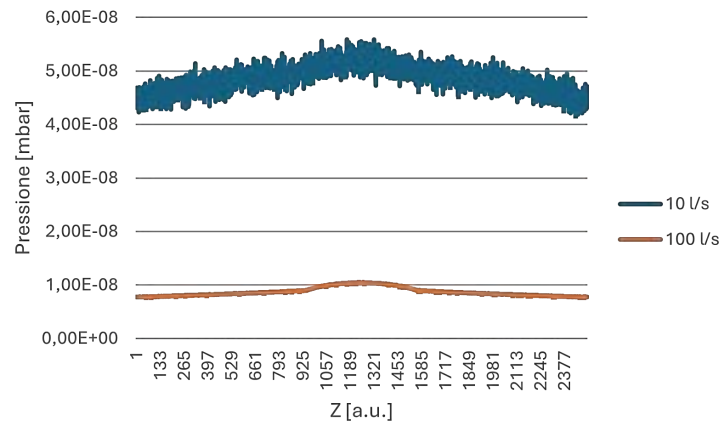
Figure 16.10: Laser Heater Chamber: Pressure Distribution for 10 L/s and 100 L/s
