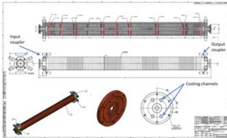
Figure 6.8: Mechanical drawing of the X-band structure.
