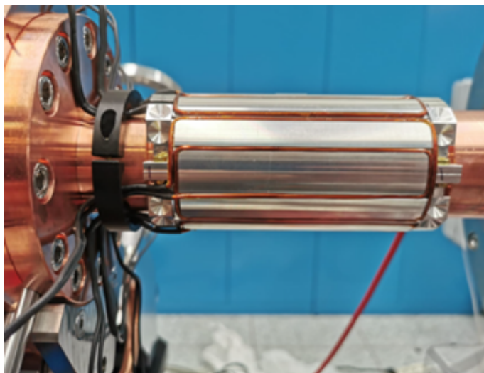
Figure 17.4: Skew quadrupole mounted on the SPARC_LAB gun vacuum chamber
