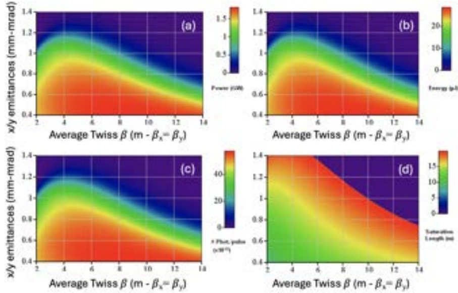
Figure 8.8: As in Fig. 8.7, the four panels represent the dependence of the peak power (a), the pulse energy (b), the number of photons per pulse (c) and the saturation length (d) as functions of the transverse normalised emittances and the average \beta_T , but with the undulator in linear polarisation.
