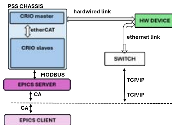
Figure 19.33: PSS Architecture
