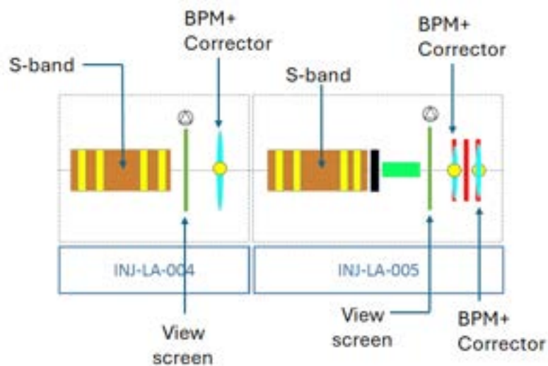
Figure 11.33: Diagnostics positions in the injector area section INJ-LA-004-005.
