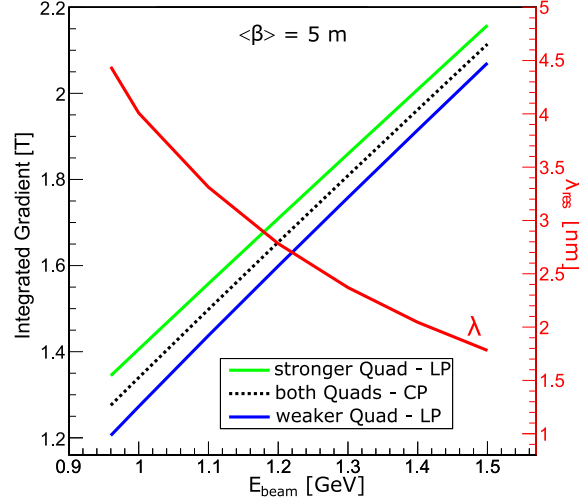
Figure 8.15: Quadrupole Integrated gradient as a function of beam energy with a Twiss \beta = 5\text{ m} , for both LP and CP configurations, superimposed to the achievable wavelength \lambda as a function of the electron beam energy. Calculated for \lambda_u = 18\text{ mm} , K_{rms} = 0.84 .
