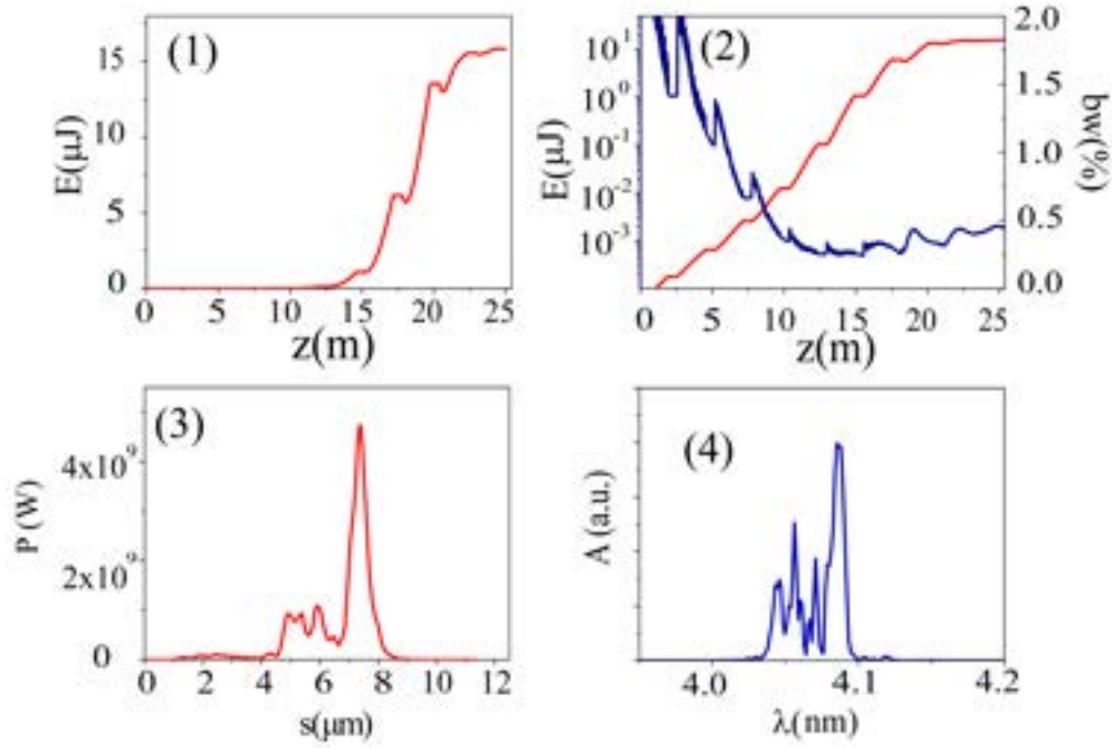
Figure 1.4: Genesis simulation results for PWFA working points with Undulator Tapering, Plot (1): energy growth in linear scale. Plot (2): energy growth in logarithmic scale and bandwidth in %. Plot (3): power distribution. Plot (4): amplitude of spectral distribution.
