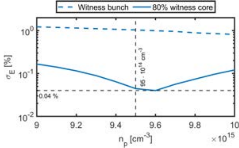
Figure 3.8: Energy spread of the bunch \sigma_E as a function of the input plateau density for the reference charge configuration 30 pC (dashed line) and for the 80% core of the distribution (continuous line).
