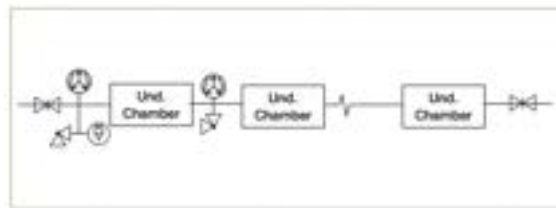
Figure 16.17: Undulators: Vacuum Schematic Layout
