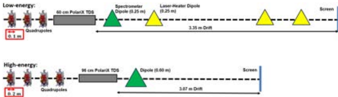
Figure 11.14: Simplified 2D layout of the diagnostic beamlines hosting the PolariX TDS. The setup includes matching quadrupoles, the TDS cavity (situated before the dipole spectrometer), a drift section, and a downstream screen.
