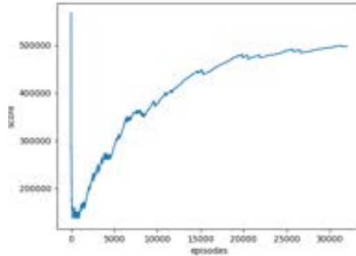
Figure 15.5: Q-learning system to adjust the beam energy changing the RF power and phase. The target energy is 511 MeV. The final energy after 30000 episodes ( \sim 42 s) is 514 \pm 3 MeV.
