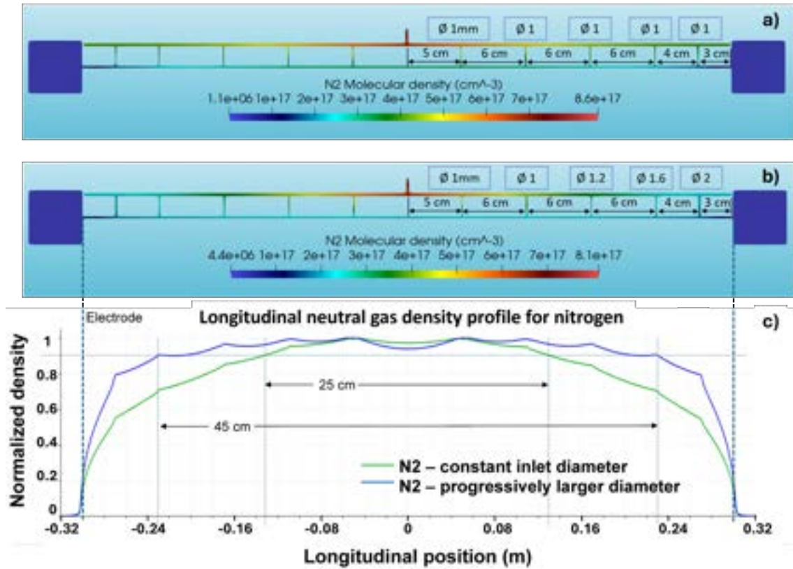
Figure 7.4: Numerical design of 60 cm long discharge capillaries performed with CFD simulations. a) Capillary design composed of ten gas injectors with the same diameter of 1 mm, b) Capillary design composed of ten gas injectors with increasing diameter towards the extremities, c) Longitudinal nitrogen density profiles for both solutions.
