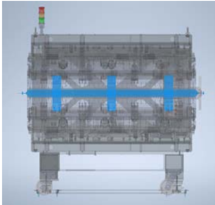
Figure 8.55: Undulator frame with the vacuum chamber in place. On the right side it is visible the vacuum chamber extension required to host the phase shifter (see Sec. 8.6)
