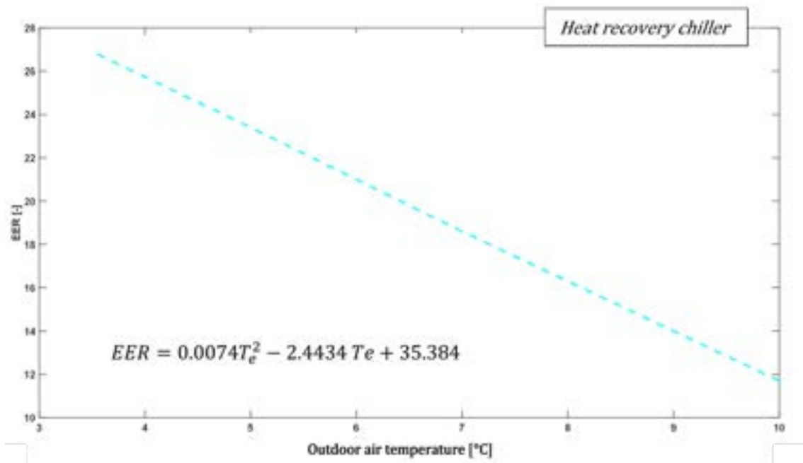
Figure 21.5: EER depending on outdoor air temperature, free cooling operating mode
