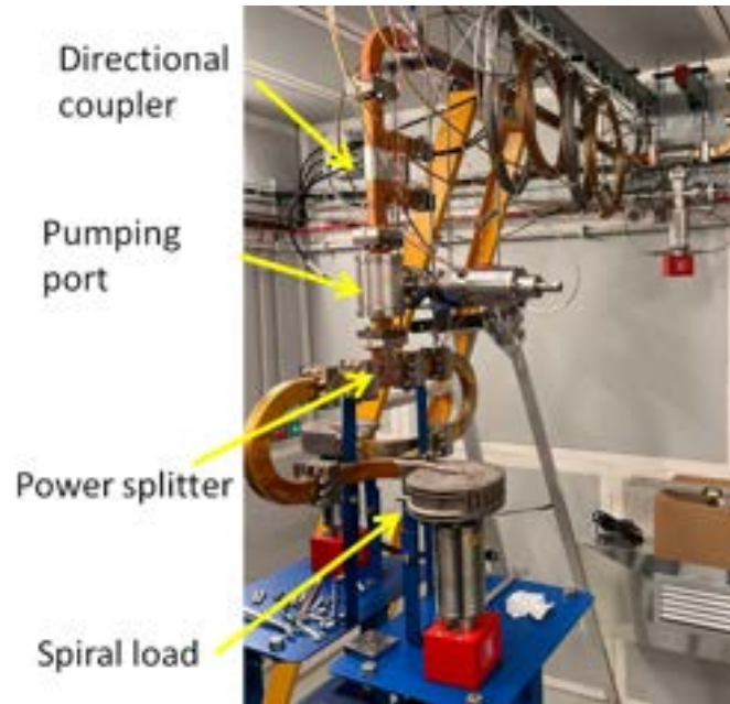
Figure 6.12: X-band components under test at the LNF TEX test facility.
