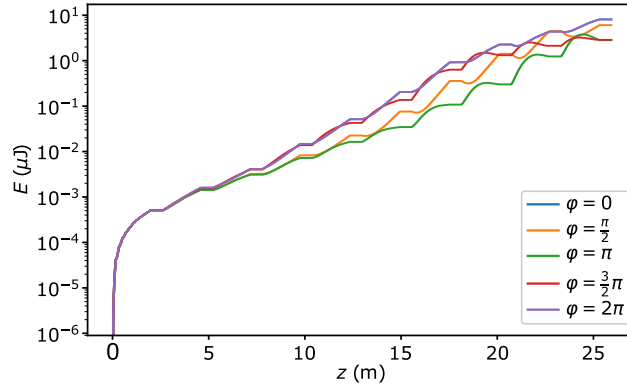
Figure 8.34: Intensity growth of the FEL radiation as a function of the phase advance in the separations between the modules of the AQUA undulator line. Cases for \phi = 0 and \phi = 2\pi are equivalent and then overplotted.
