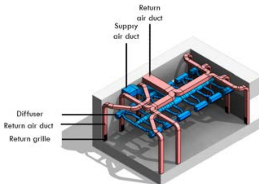
Figure 18.21: Experimental Hall ventilation system.
