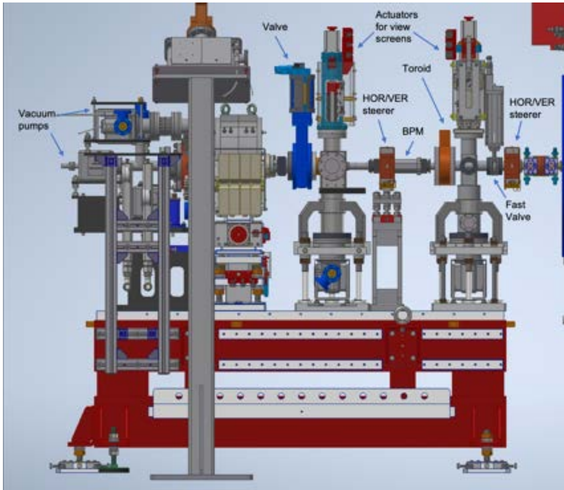
Figure 5.12: Gun to first boosting section layout.
