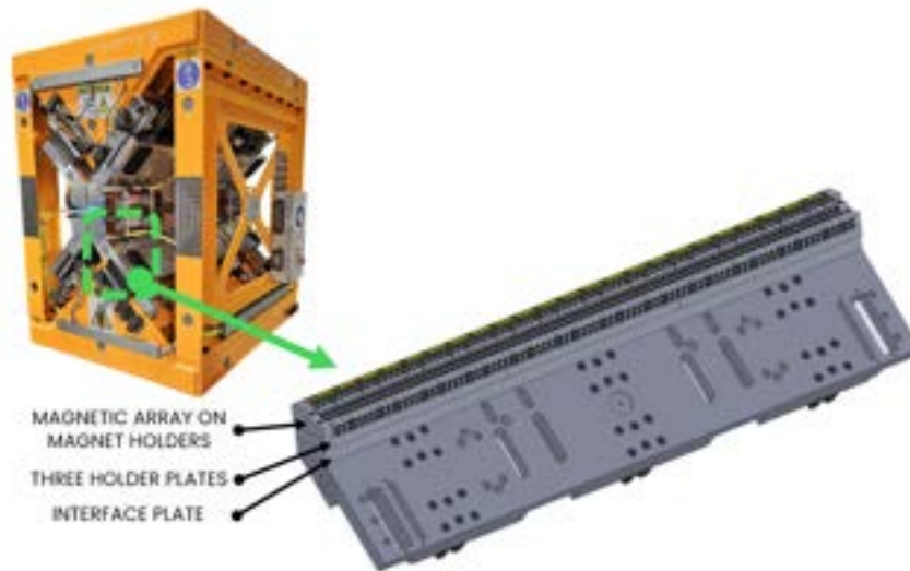
Figure 8.30: Mechanical structure under investigation.
