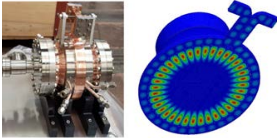
Figure 6.17: Picture of the X-band BOC (left); electromagnetic field configuration of the BOC operating mode TM_{18,1,1} [14].
