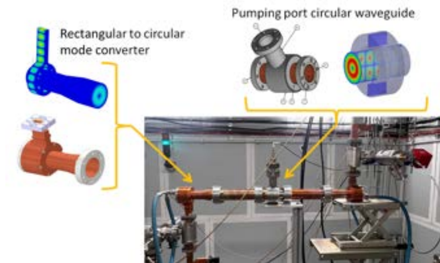
Figure 6.14: Rectangular to circular mode converter, pumping units and circular waveguide installed in the TEX facility.
