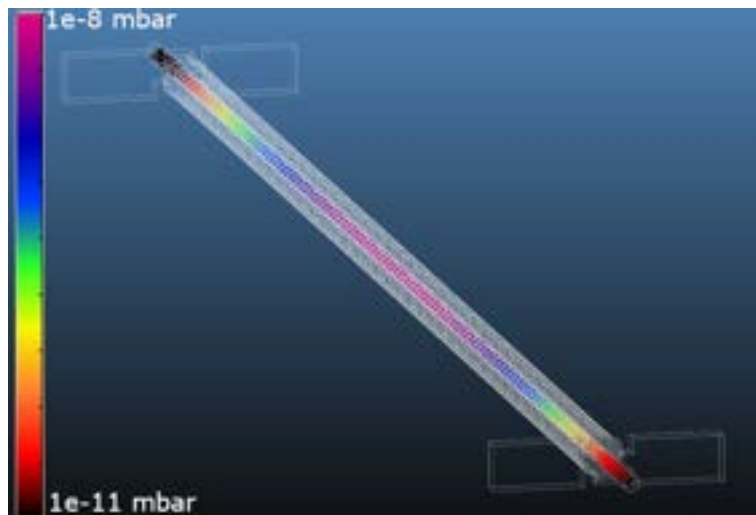
Figure 16.12: X-Band Accelerating Structure: pressure distribution simulated for q = 1 \cdot 10^{-12} mbar l/s \text{cm}^2
