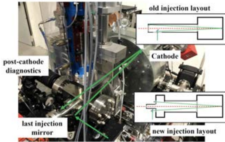
Figure 5.5: S-band RF gun installed at SPARC_LAB with highlighted the new laser injection system. On the insets are the layouts of the new and old systems [19].
