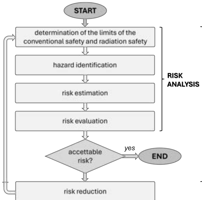
Figure 19.28: Risk assessment procedure to evaluate risk reduction measures.
