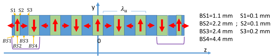
Figure 8.21: End magnets design scheme after optimization.
