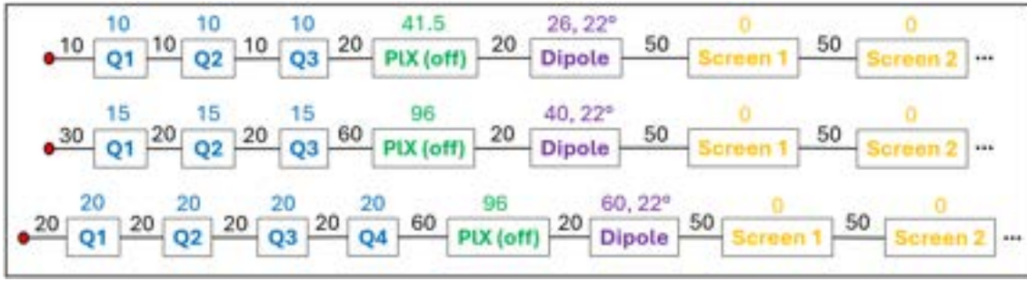
Figure 11.11: Lattice schemes assumed in the simulations, at the design energy of 120 MeV (top), 400 MeV (middle) and 1 GeV (bottom). The numbers without units indicate lengths in centimeters. The red dots indicate where the simulations start. The quadrupoles are represented in blue. The PolariX RF transverse deflecting structures (see Section 11.2.8) are in green. They are switched off during the beam energy measurements, so the tracked macroparticles see them as drifts. Design length and bending angle of each dipole are indicated in purple. The dipole operating at 120 MeV is rectangular, whereas the other two are sector magnets. In simulation, the beam spot is analyzed at six evenly-spaced positions (‘screens’ with zero length) after each dipole, starting from 50 cm from the dipole exit and ending at 3 m.
