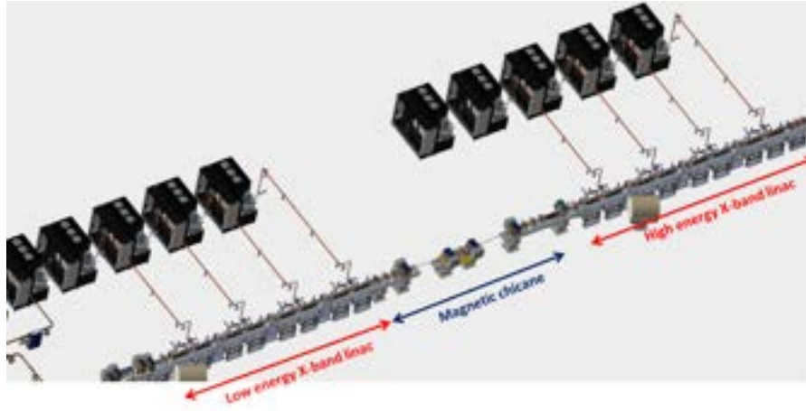
Figure 6.1: X-band linac layout.
