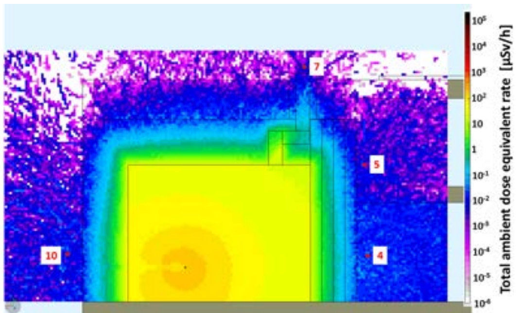
Figure 19.17: H^*(10) - 800 MeV diagnostic beam dump - xy plane.
