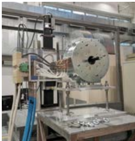
Figure 17.2: SPARC_LAB gun solenoid during the Hall probe measurements at LNF
