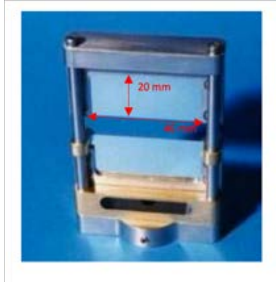
Figure 11.19: Picture of the CDR target. From [37].
