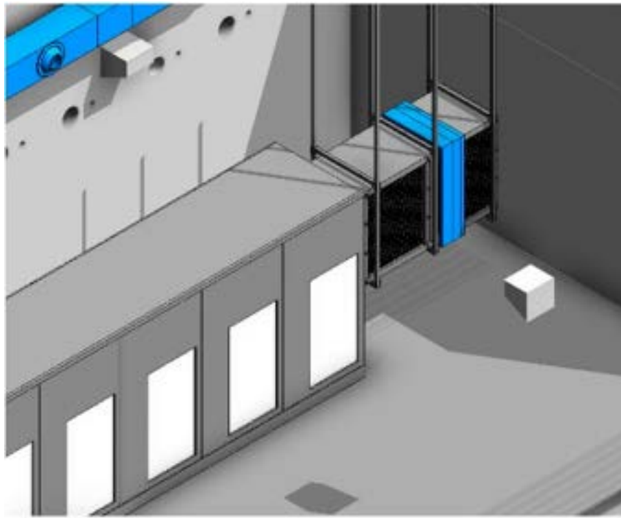
Figure 18.27: Undulators enclosure ventilation system.
