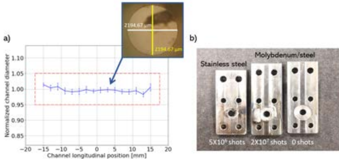
Figure 7.13: a) Longitudinal profile of the capillary channel cross section, measured after 20 million shots at 30-150 Hz and normalized to the channel profile measured at 0 shots. The insert shows a microscopic image acquired from the capillary center, in which the cross section diameter is computed by the average of the horizontal and vertical measurements, that in this case are coincident. b) Comparison between different electrode configurations, tested at high repetition rate with the ceramic capillary. The use of an inner disk made of molybdenum allows to better preserve the integrity of the electrodes after 20 million shots.
