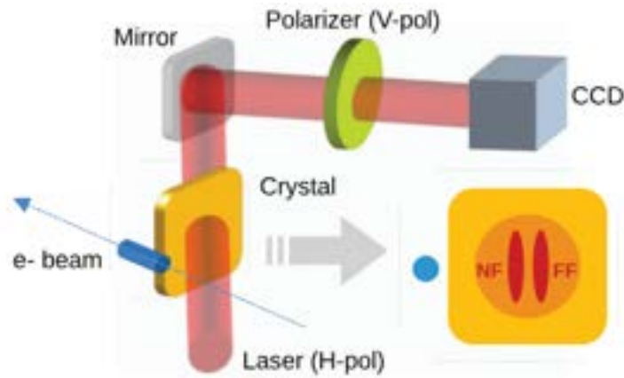
Figure 11.18: Experimental setup of the EOS system: the laser crosses the crystal and its polarization changes under the effect of the external field. The laser is then polarized vertically, and the signal is recorded by the CCD downstream of the crystal [36].
