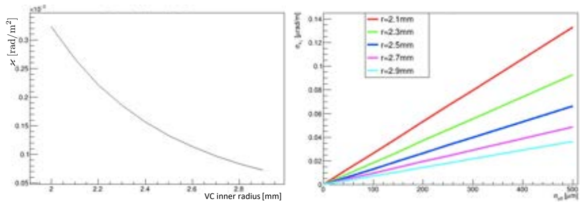
Figure 8.49: Left: kick parameter per unit length per transverse offset as a function of the vacuum chamber inner radius. Right: uncertainty in the kick angle per unit length as a function of the misalignment jitter value, for different vacuum chamber inner radii.
