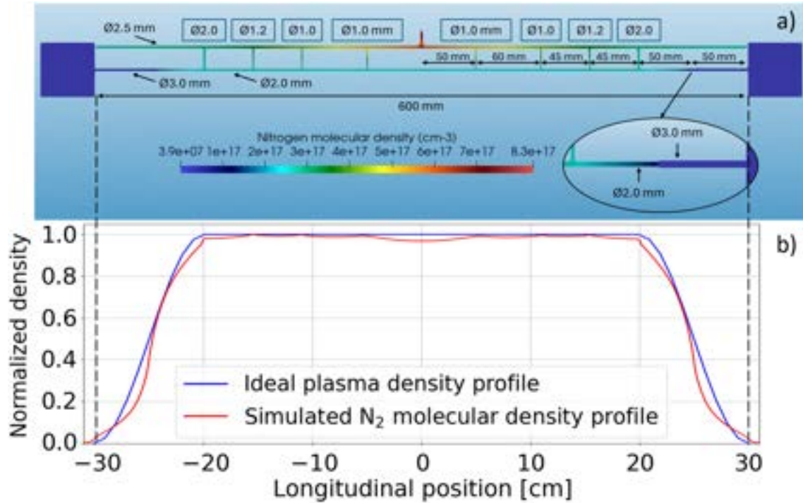
Figure 7.9: Numerical design of the 60 cm long gas-filled discharge capillary to reach the final energy of 1 GeV. a) 2D nitrogen density distribution showing the geometrical design of the capillary, constituted by 8 inlets, whose diameter ranges from 1 to 2 mm, and a widening of the horizontal channel diameter from 2 mm to 3 mm in the outer 5 cm of the channel at both sides. b) Comparison between the ideal plasma density profile described in Sec. ??, with squared cosine ramps and a 40 cm long density plateau, and the simulated nitrogen density profile.
