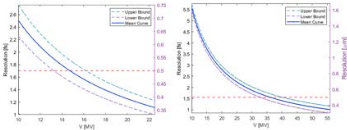
Figure 11.15: Left: Longitudinal resolution for the low-energy station, assuming a nominal natural beam transverse size of \sigma_y \sim 60\ \mu\text{m} , and for a 0.6-m-long PolariX. Right: Longitudinal resolution for the high-energy station, assuming a nominal natural beam transverse size of \sigma_y \sim 14\ \mu\text{m} , and for a 0.96-m-long PolariX. The red dashed lines correspond to time resolutions of 0.5\ \mu\text{m} , which represents the target value achievable for this measurement. The upper and lower boundaries takes into accounts for shot-to-shot variations in the measured beam size.
