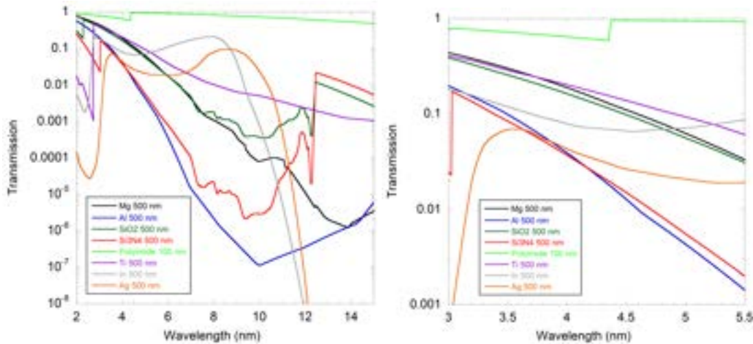
Figure 9.6: Transmission of 500 nm filter made from various materials. Some materials require a polyimide substrate (plotted separately). The right plot zooms in around the carbon K-edge.
