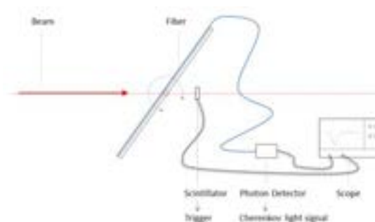
Figure 11.26: Schematic of the time-of-flight measurement setup, used to determine the location of a beam loss along the accelerator.
