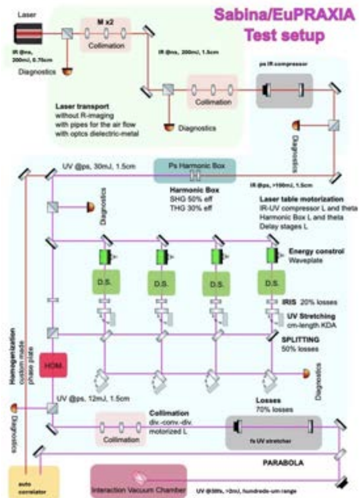
Figure 12.4: Schematic of the laser chain after compression.
