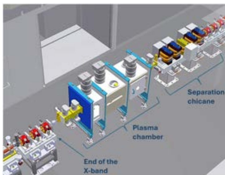
Figure 7.1: Plasma module zoomed view in the accelerator layout.
