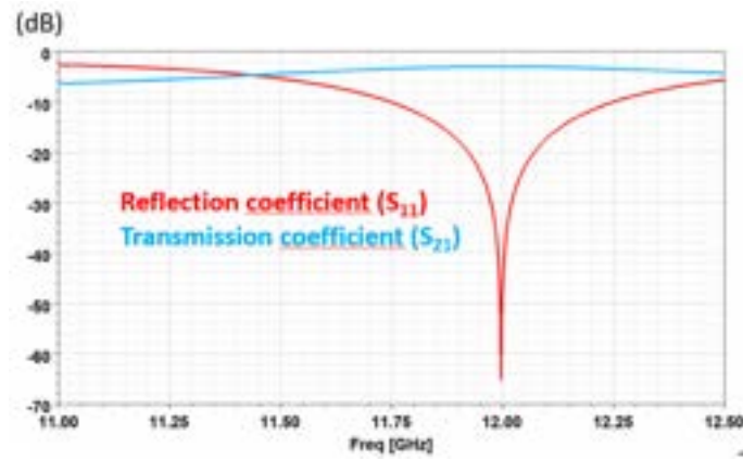
Figure 5.9: Reflection coefficient (in red) and transmission coefficient (in blue) of the RF power splitter.
