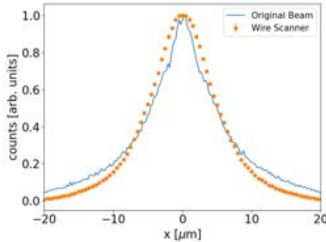
Figure 11.23: GEANT4 simulations of the wire scanner. Blue line: original transverse distribution of the driver and witness bunches from start-to-end simulations of the linac. Orange points: simulated secondary photons collected between 1 and 4 mrad with respect to the beam direction for different wire positions.
