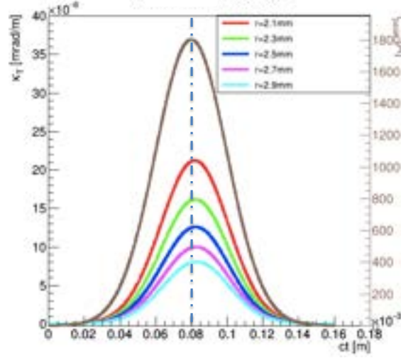
Figure 8.50: Kick angle per unit length for different vacuum chamber inner radii, and for a transverse offset of 50 \mu\text{m} , superimposed to the long bunch current profile (brown curve).
