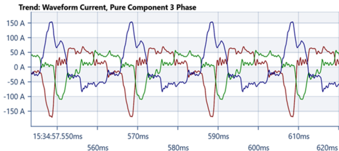
Figure 18.13: Current Waveform for 100 Hz operated Modulator.
