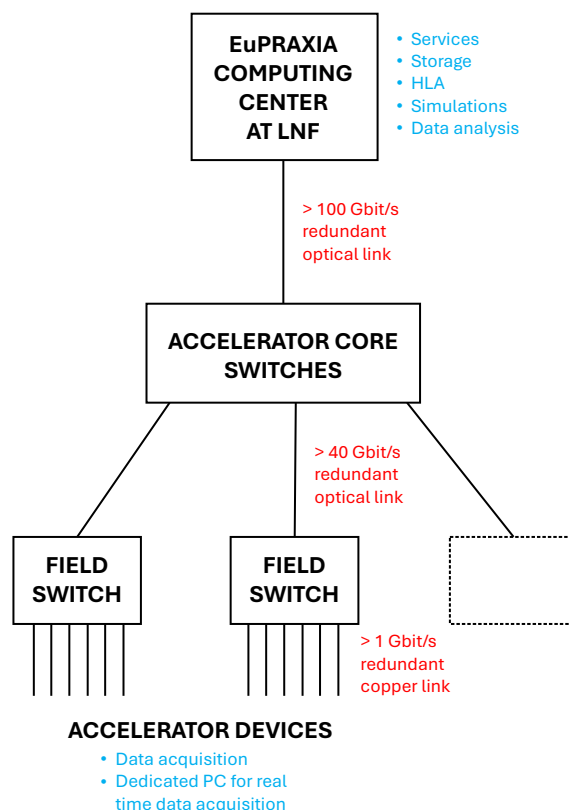
Figure 15.7: EuPRAXIA network design scheme.
