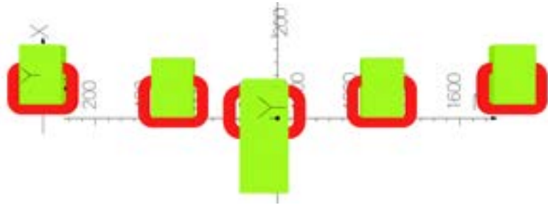
Figure 17.19: The 3D view of the driver-witness separator chicane, showing from left to right: dipoles D1 and D2, the septum, and dipoles D3 and D4.
