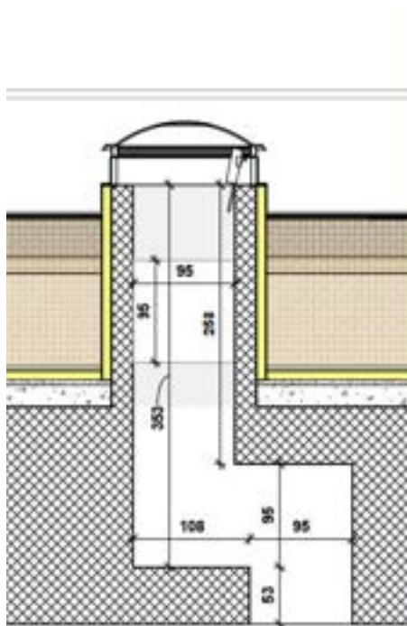
Figure 19.5: Section of a SHEVS exhaust opening showing the "double-L" structure
