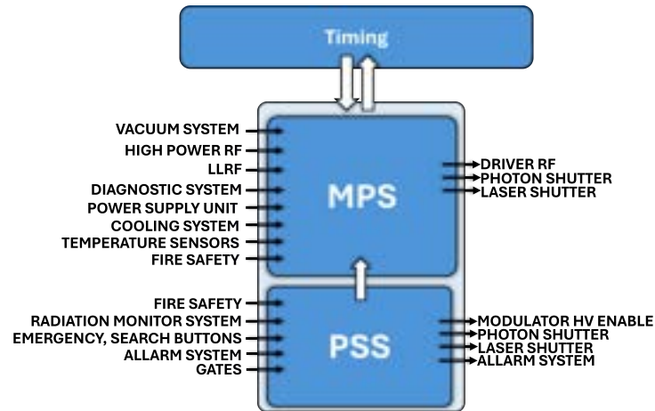
Figure 19.32: Diagram of the PSS at EuPRAXIA@SPARC_LAB, showing its control and monitoring of all safety-related systems, including fire protection, radiation monitoring, alarm systems, access gates, and search and emergency buttons, and its role in sending an enable signal to the MPS to ensure the system operates safely according to PSS requirements.
