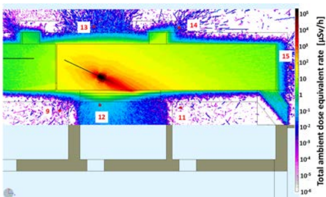
Figure 19.18: H^*(10) - 1.2 GeV diagnostic beam dump - xz plane.
