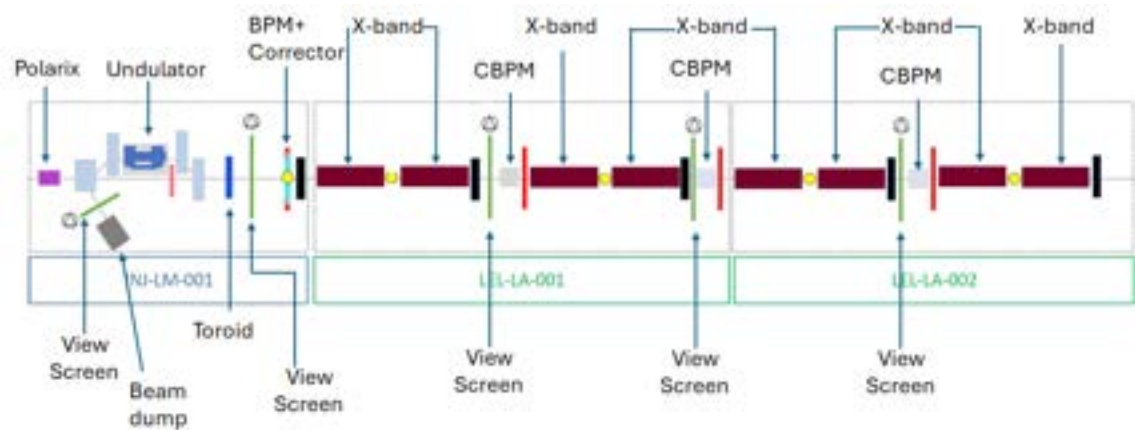
Figure 11.34: Diagnostics positions in low energy linac.
