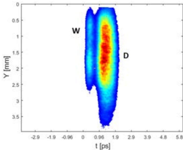
Figure 11.16: Measured signals of the driver (D) and witness (W) bunches, obtained at the SPARC_LAB facility [33]. The horizontal axis represents the longitudinal bunch distribution, while the vertical axis is the probe laser transverse profile. The measured relative distance is about \sim 1 ps.
