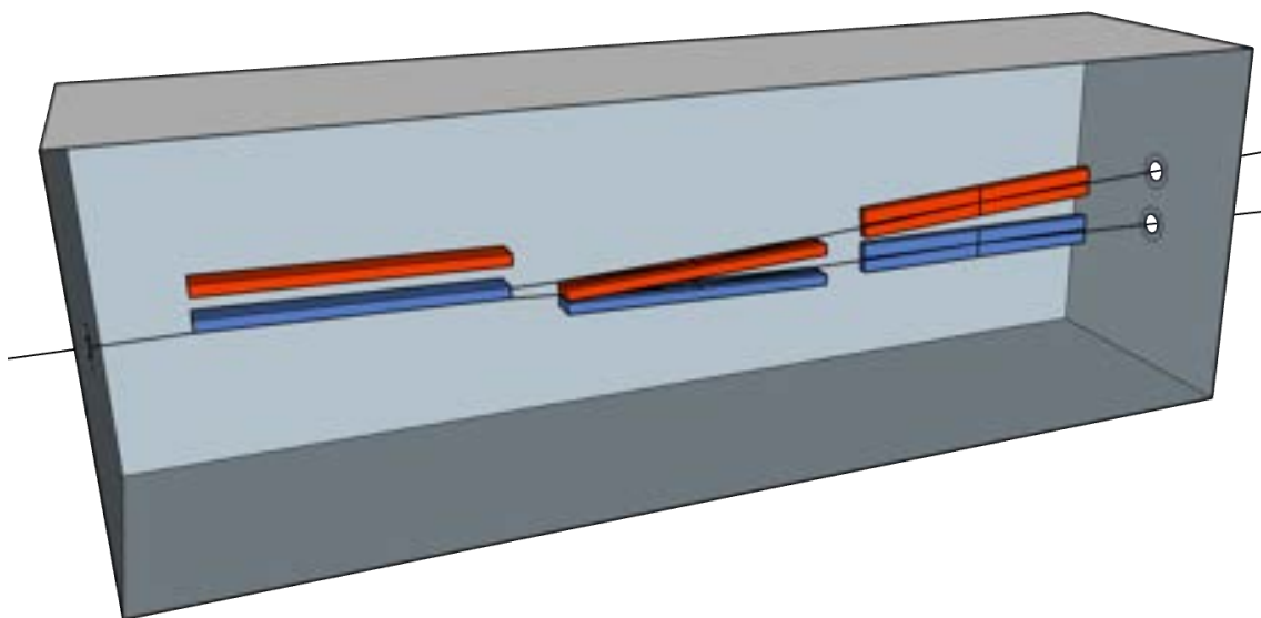
Figure 9.12: 3D schematic view of mirror configurations with (blue) and without (red) the vertical steering mirror.
