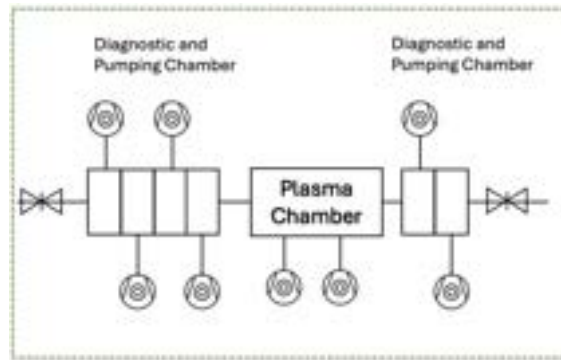
Figure 16.15: Plasma Area: Vacuum Schematic Layout
