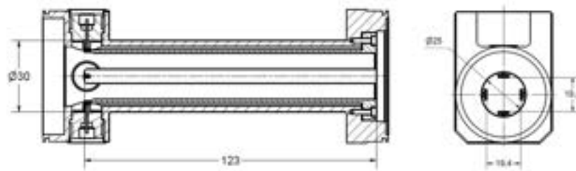
Figure 11.2: Technical design of the strip-line BPM pickup. All distances in mm.
