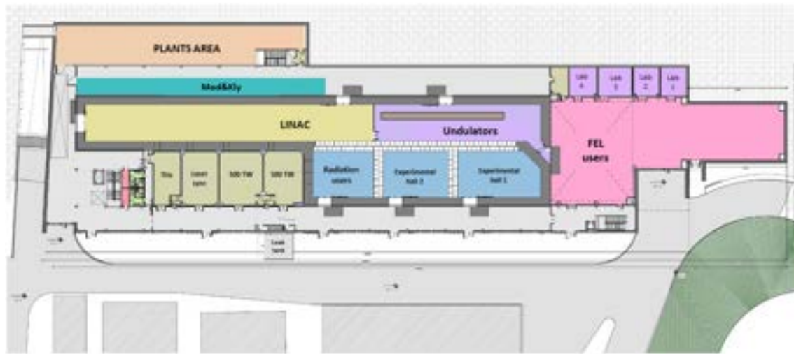
Figure 18.5: EuPRAXIA@SPARC_LAB building functional layout - Level 0.
