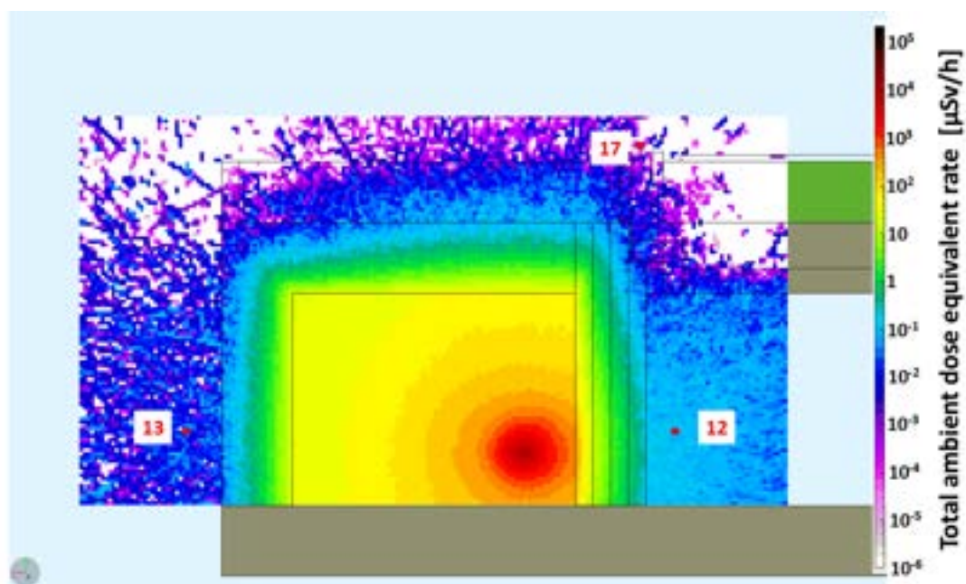
Figure 19.19: H^*(10) - 1.2 GeV diagnostic beam dump - xy plane.
