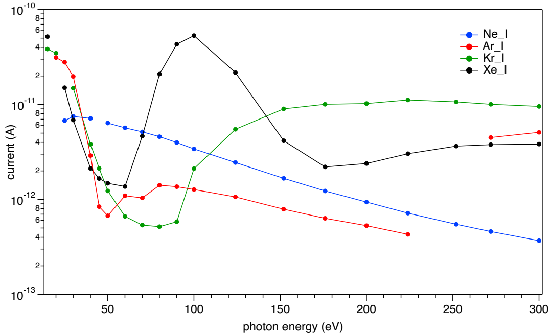
Figure 9.14: Estimate of the expected current from a GMD according to Eq. (9.1), using z_{\text{eff}} = 22 cm, p = 10^{-5} mbar, 10^{10} photons/pulse, and 100 Hz repetition rate at room temperature. Four different rare gases are considered. Breaks in the curves correspond to resonance regions. Cross section and mean charge data from [23].
