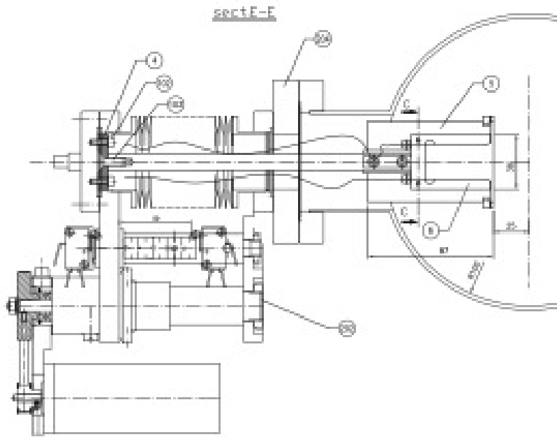
Figure 9.15: Layout of the plate BPM
