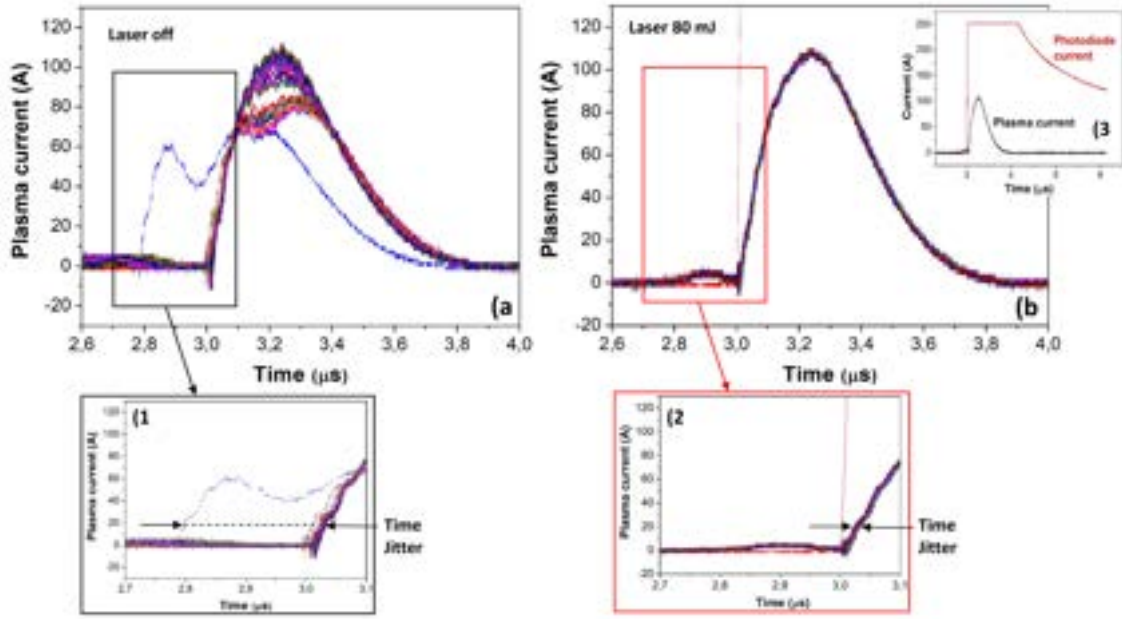
Figure 7.16: Current discharge waveforms obtained with laser turned off (a) and on with 80 mJ pulse energy (b). Each plot shows a set of 50 measurements obtained by applying 5 kV between the capillary electrodes. Insets 1) and 2) show the time jitter without and with the use of the stabilizing laser, respectively. The inset 3) shows the laser pulse signal measured with a photo-diode.
