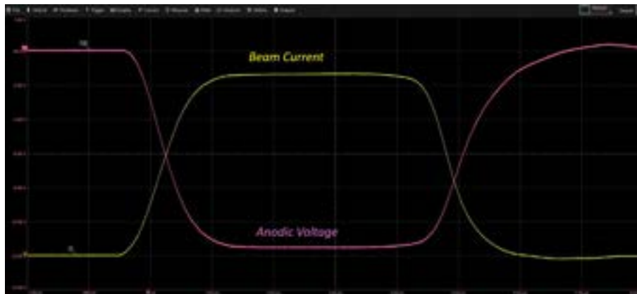
Figure 13.9: Example of measured klystron anode voltage and corresponding beam current waveforms.
