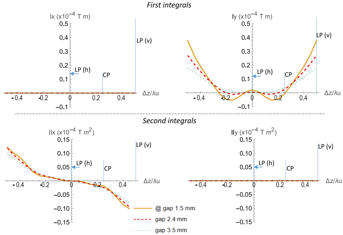
Figure 8.22: Undulator field integrals. The first I_{x,y} and the second II_{x,y} integrals are plotted for the radial (x) and vertical (y) components depending on the phase value ( \Delta z/\lambda_u ) which determines the polarization mode. Different lines refer to different gap values, 1.5 mm (minimum gap), 2.4 mm (resonance 4 nm) and 3.5 mm ( K_{rms} \approx 0.6 ).
