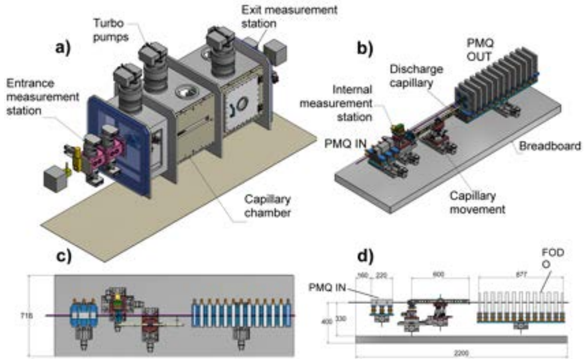
Figure 7.3: Plasma source housing chamber. a) Chamber external view. All turbo pumps are mounted on the top of the chamber. Two small auxiliary chambers are positioned upstream and downstream to accommodate the entrance and exit beam diagnostics. b) Chamber inside view: a PMQ triplet is positioned at the entrance and a FODO cell at the exit. c) Top view and d) side view of the internal elements of the plasma chamber.
