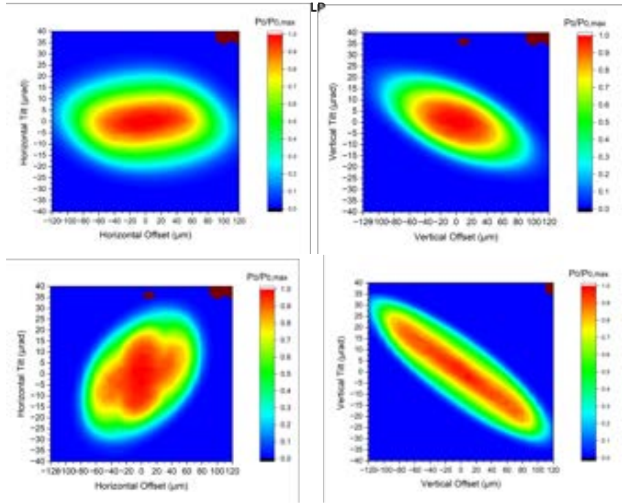
Figure 8.45: FEL emission from the nominal electron bunch with \beta_T = 8 m (top line) and \beta_T = 5 m (bottom line). Maximum achievable radiation power level P_0 for a given transverse misalignment, normalized to the maximum FEL power P_{0,max} achieved along the undulator line in the whole range of explored misalignments in linear polarization (LP) as a function of the initial horizontal (left) and vertical (right) tilt angles ( \mu\text{rad} ) and offsets ( \mu\text{m} ).
