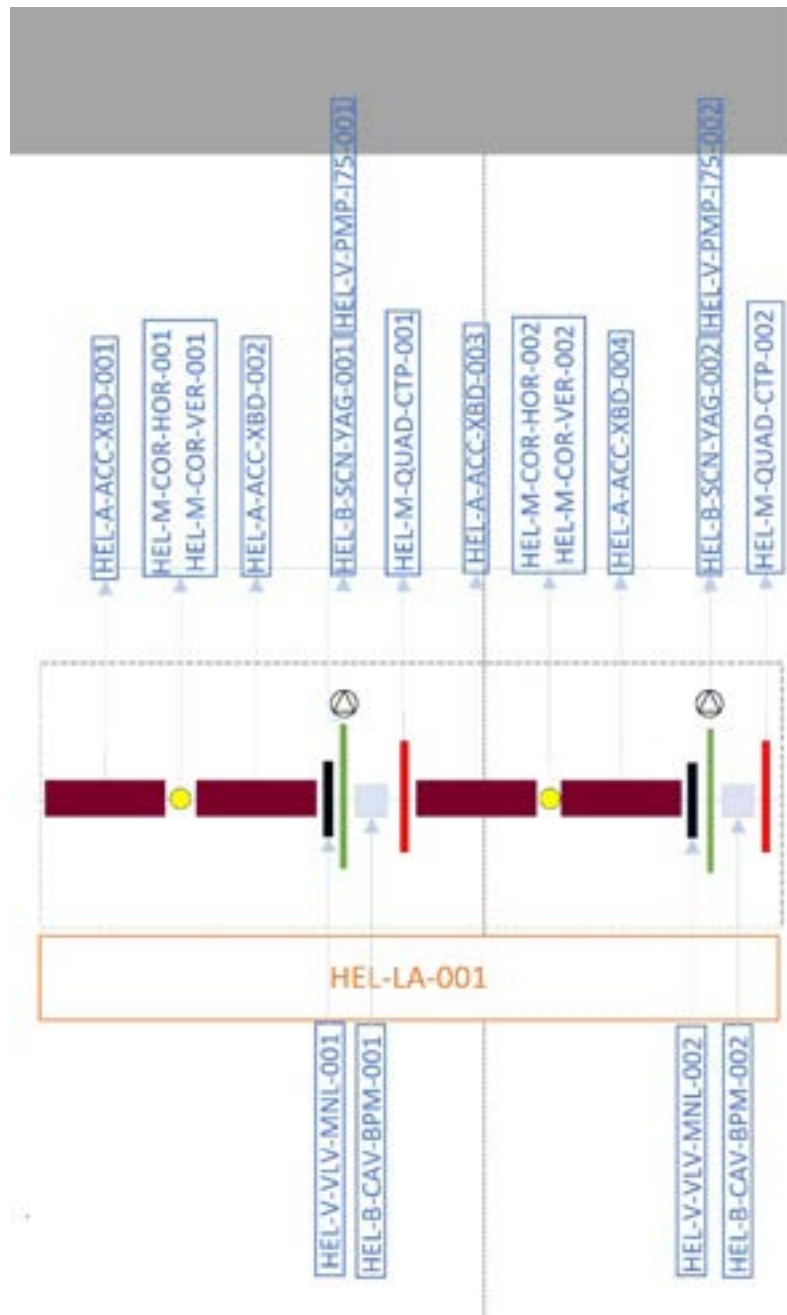
Figure 20.14: Schematic Layout of the Second Module of the X-Band Accelerating Section.
