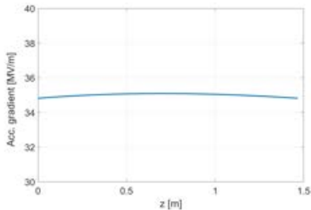
Figure 13.5: Quasi-constant accelerating gradient across the 1.5 m structure.
