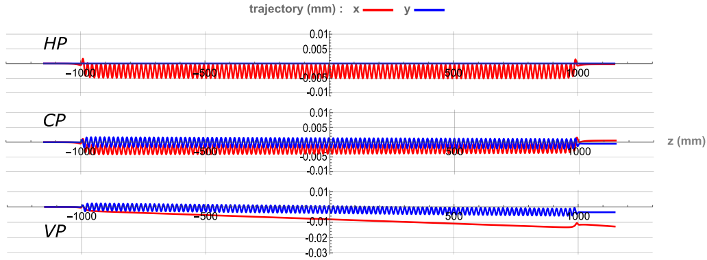
Figure 8.23: Trajectory in the undulator for an electron with initial null offset and angle at the entrance in the undulator. The linear Horizontal (HP), Circular (CP) and linear Vertical (VP) polarization cases are plotted.
