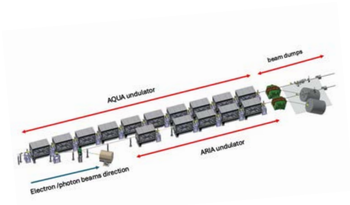
Figure 4.9: Layout of the Free Electron Laser undulators area
