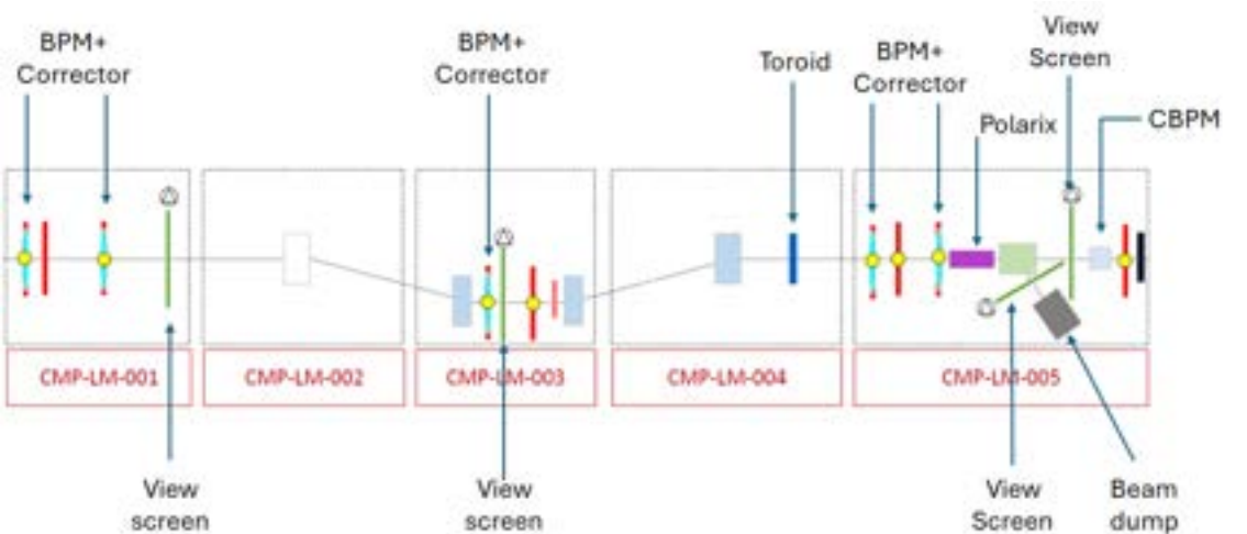
Figure 11.35: Diagnostics positions in bunch compressor
