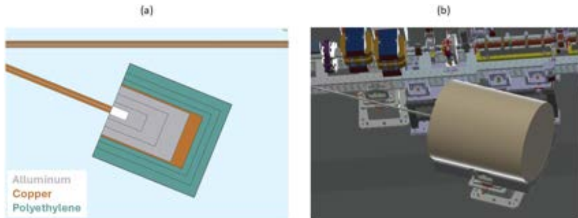
Figure 19.11: Diagnostic beam dump layout in 2D (a) and 3D (b).
