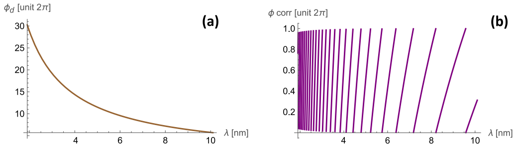
Figure 8.35: (a) Phase delay introduced by the break section with variation of the resonant wavelength of operation. (b) Required phase correction from the phase shifter in the operational wavelength range. The phase values are given in units of 2\pi .
