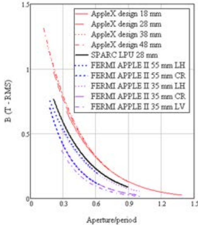
Figure 8.2: Undulator on axis field (RMS) as a function of the aperture/period ratio for different undulator types and polarizations. Data for SPARC and FERMI undulators correspond to measurements on real devices. The APPLE X undulator is designed and simulated in RADIA [8]. The RMS field in APPLE-X type undulator devices is independent from the polarisation.
