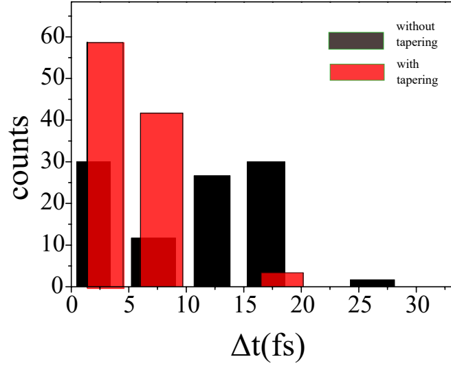
Figure 3.18: Histogram of the number of event as function of the FEL photon pulse length \Delta t in fs. Black columns: without tapering, red columns: with tapering
