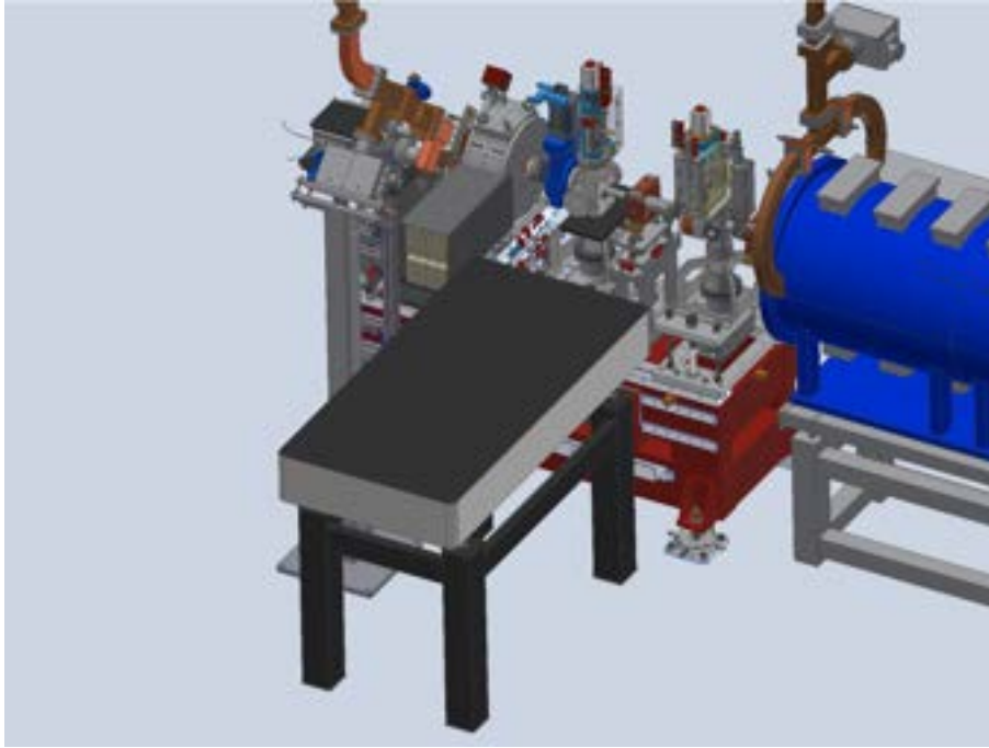
Figure 12.9: Side view of the gun with the optical table for laser diagnostics.
