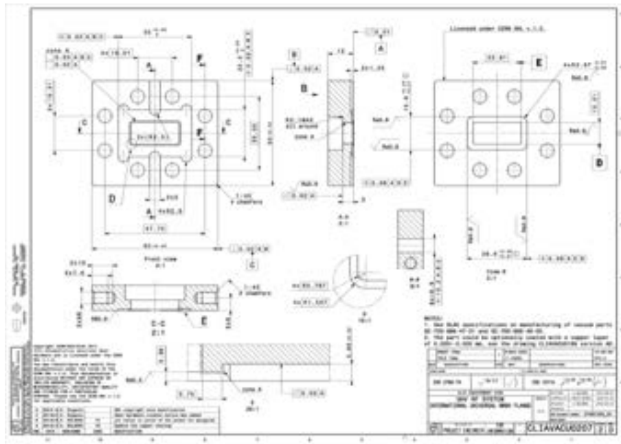
Figure 6.13: Rectangular X-band flange (International flange) adopted for waveguide connections CERN drawing (CERN design and open source repository).
