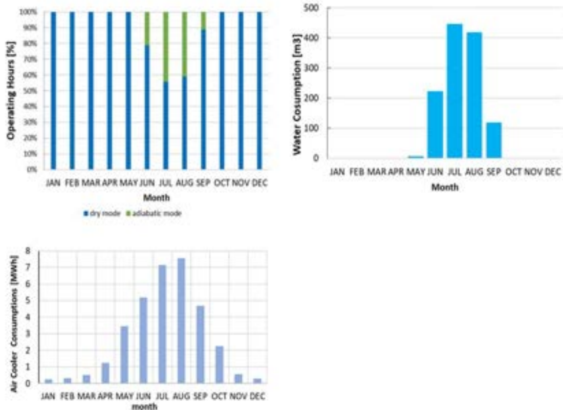
Figure 18.16: Top-left: Monthly operating hours – dry mode and adiabatic mode; Top-right: Monthly water consumption of the dry cooler in adiabatic mode; Bottom-left: Monthly electrical consumption of the air cooling system.
