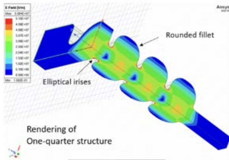
Figure 5.6: Rendering of one quarter structure of the RF cavity from Ansys.
