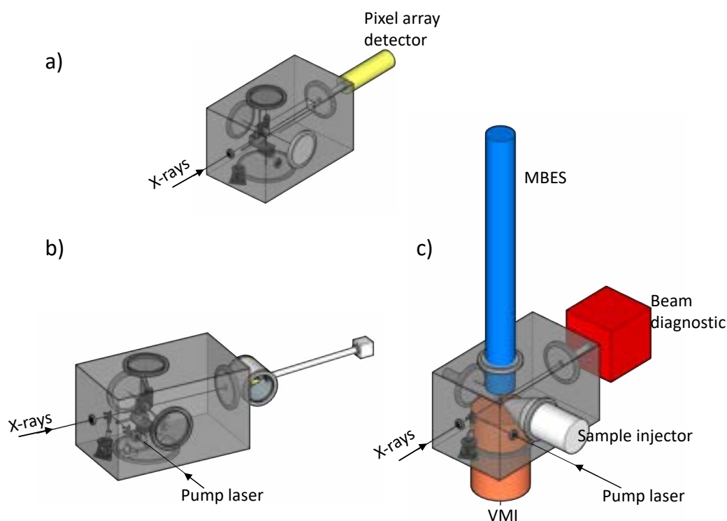
Figure 10.1: Schematic representation of planned configurations for the experimental chambers during P0–2 . Panel (a) illustrates the P0 setup for CDI experiments, featuring the pixel-array detector positioned downstream of the sample. Panels (b) and (c) depict possible configurations for P1 and P2 , corresponding to XAS and ion/electron spectroscopy, respectively. In panel (b), soft X-ray absorption signals are measured with a photodiode placed downstream of the sample, used together with an upstream spectral measurement for correlation spectroscopy. Panel (c) shows an arrangement combining a sample injector, velocity-map imaging (VMI) spectrometer, and beam-diagnostic module (i.e. Hartmann sensor).
