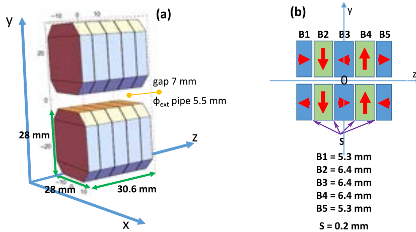
Figure 8.36: (a) Structure of the phase shifter for the AQUA undulator. (b) Longitudinal scheme showing the orientation of the magnetic field in the blocks and the end magnets design.
