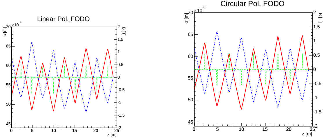
Figure 8.13: Transverse rms size of the electron beam subject to the undulator plus FODO sections in Linear (left) and Circular (right) polarization operations.
