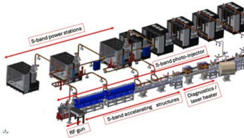
Figure 4.6: Layout of the S-band photo-injector
