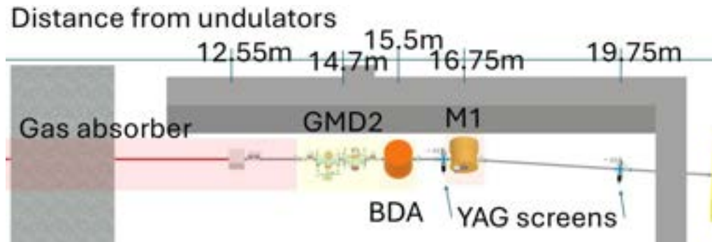
Figure 9.3: Layout of the AQUA beamline inside the bremsstrahlung shielding area (Fig. 9.1, view B). BDA: beam defining aperture; M1: mirror chamber.
