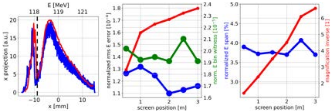
Figure 11.12: Simulation results for the driver and witness at 120 MeV. Left: projection (blue) of the camera FOV on the horizontal axis, for the screen placed at 2 m from the dipole exit. The energy axis is derived from the horizontal one by using the leftmost formula in Eq. 11.2. The energy profile of the initial beam distribution is in red. The witness and driver bunch profiles can be distinguished on the screen, respectively on the left and right of the dashed black line. Middle: normalized rms energy errors for the witness (blue) and driver (red), and the normalized energy resolution for the witness (green), as a function of the distance between the screen and the dipole exit. Normalizations are performed with respect to the mean of the corresponding initial energy profile. Right: energy span (blue), covered by the horizontal FOV and normalized by the mean of the initial beam energy profile. The inverse of the magnification is in red.
