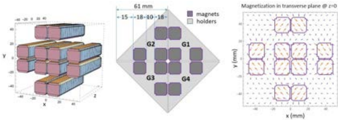
Figure 8.28: Compensating magnets scheme of the undulator array.
