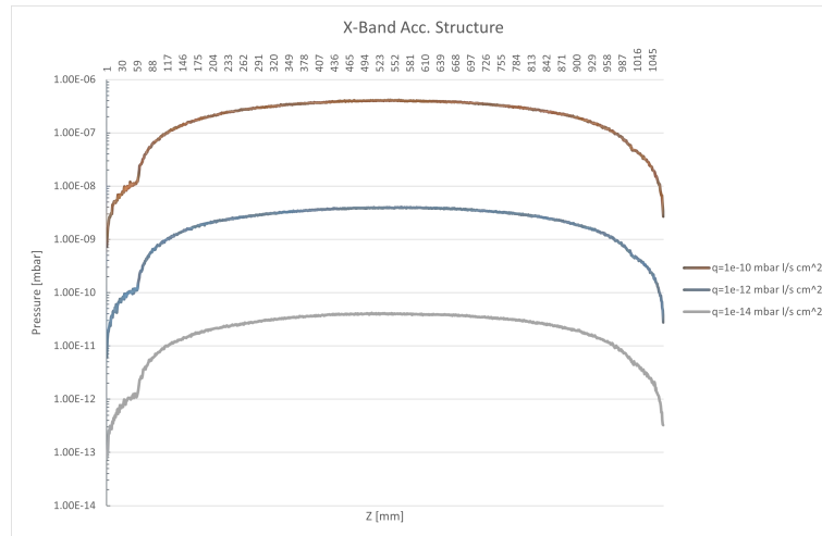
Figure 16.13: X-Band Accelerating Structure: Pressure Distribution
