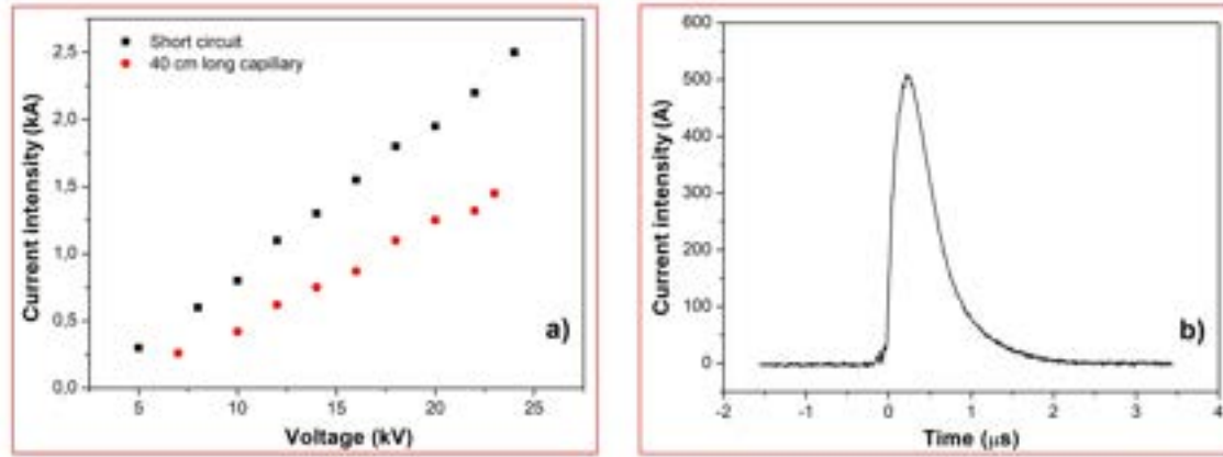
Figure 7.15: High-voltage source characterization: a) Current pulse peak, measured at the output of the pulser circuit as a function of the generator voltage, under short-circuit conditions (black squares) and closed circuit conditions on a 40-cm-long gas-filled discharge capillary (red circles); b) Single current profile measured at the output of the pulser circuit with 11 kV generator voltage, when the circuit is closed on a 40-cm-long capillary.
