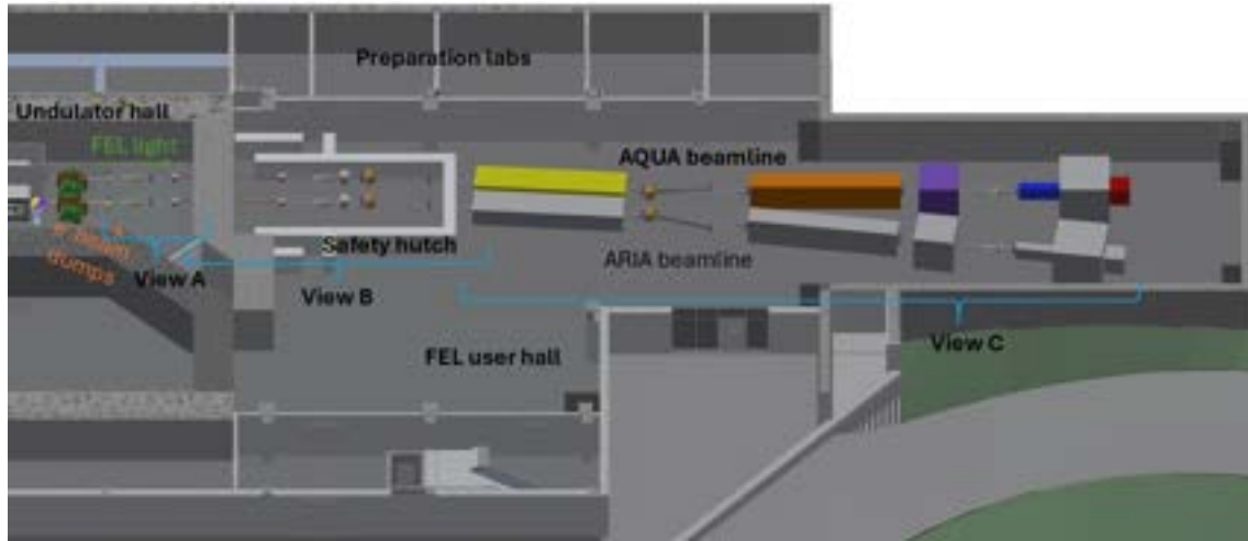
Figure 9.1: Layout of the AQUA (upper) and ARIA (lower) beamlines in the FEL user hall
