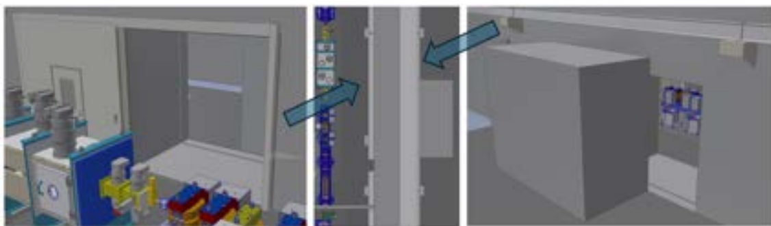
Figure 20.4: Left: View from Plasma Area; Center: Top View; Right: View from Service Tunnel.
