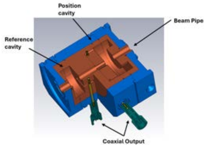
Figure 11.3: Cavity BPM PSI model "BPM8". ©2024 Fabio Marcellini (PSI)
