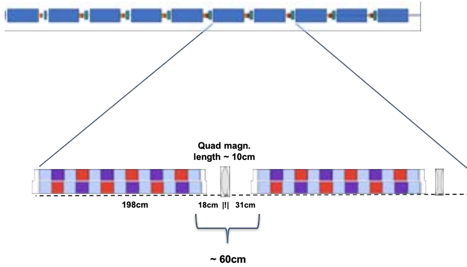
Figure 8.11: AQUA FODO cell schematic layout.
