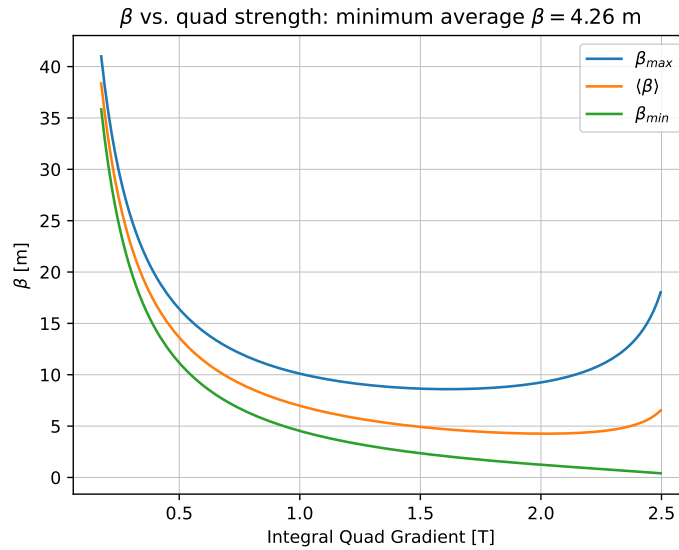
Figure 8.12: Maximum, average and minimum Twiss \beta values as a function of the integral quadrupole strength (@ 1 GeV).
