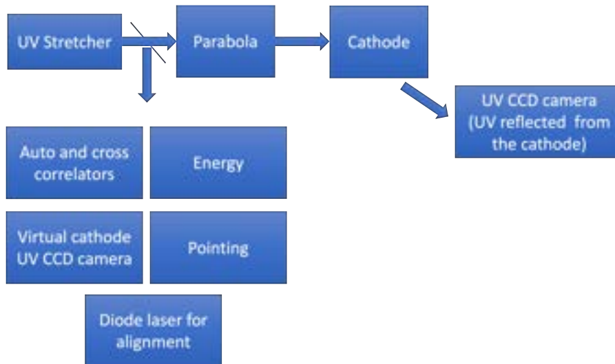
Figure 12.10: Schematic of the laser diagnostics installed on the optical table near the cathode.
