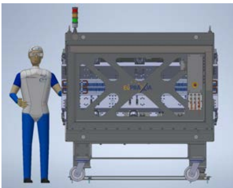
Figure 8.32: Rendering of one of the AQUA undulator modules. Side view.
