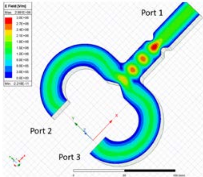
Figure 5.8: RF power splitter.
