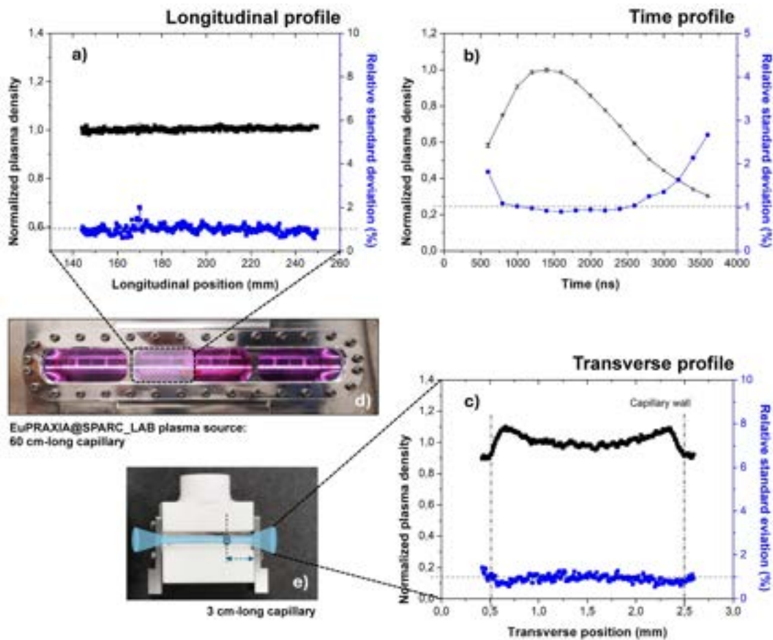
Figure 7.21: Characterization of gas-filled discharge capillaries: a) Longitudinal plasma profile obtained for 60 cm long capillary by using the optical line 2; b) Longitudinal plasma profile measured as a function of the plasma recombination time for 60 cm long capillary; c) Transverse plasma profile obtained for 3 cm long capillary by using the optical line 1; d) Measurement area for 60 cm-long capillary; e) Measurement area for 3 cm-long capillary.
