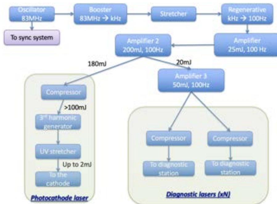
Figure 12.8: Simplified schematic of the complete laser systems.
