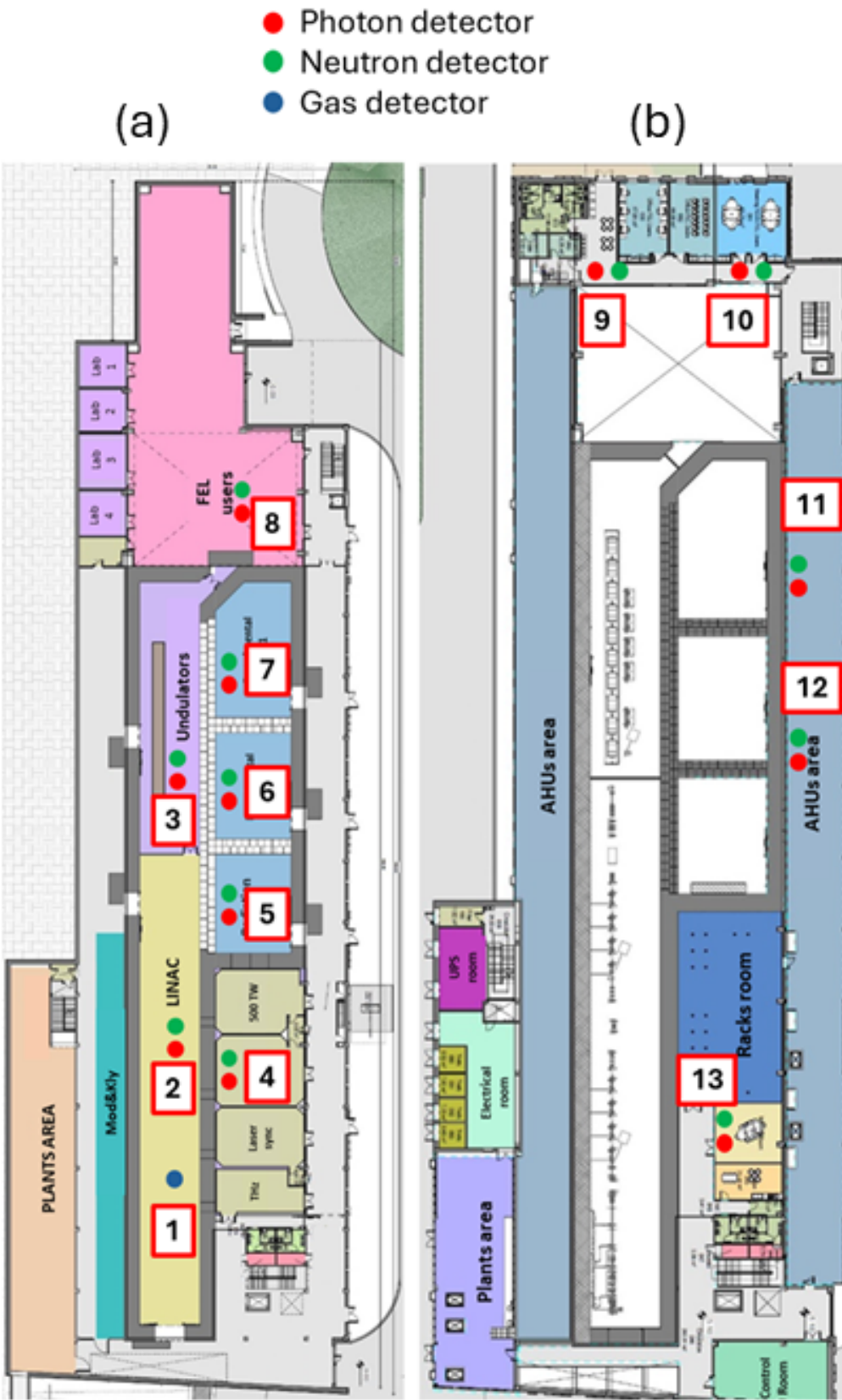
Figure 19.7: Planned detector position on the first (b) and ground (a) floor.
