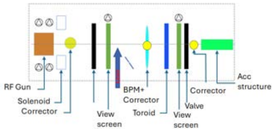
Figure 11.31: Diagnostics positions between RF gun and the first accelerating module.
