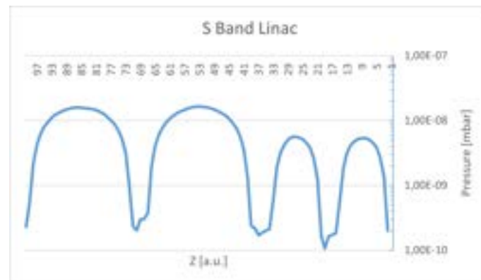
Figure 16.8: S-Band Linac: Simulated Pressure Distribution
