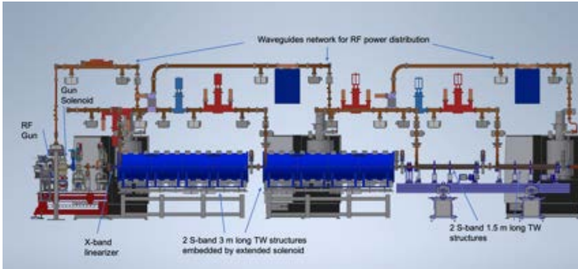
Figure 5.13: S-band boosting section layout.
