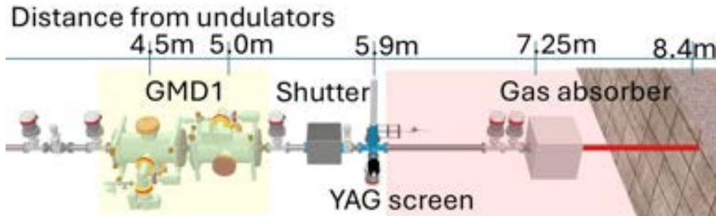
Figure 9.2: Details of the layout of the AQUA beamlines inside the undulator hall (Fig. 9.1, view A). GMD: Gas Monitor Detectors, Shutter: bremsstrahlung radiation stopper (for maintenance), YAG screen: transverse diagnostic chamber with scintillating screen and alignment laser, Gas absorber: gas attenuation module with gas insertion station and differential pumping
