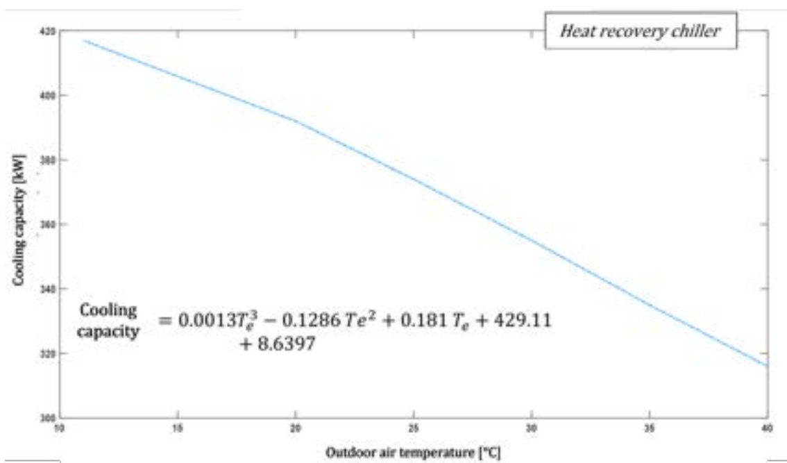
Figure 21.4: Cooling capacity depending on outdoor air temperature (under peak load conditions), operating mode without free cooling
