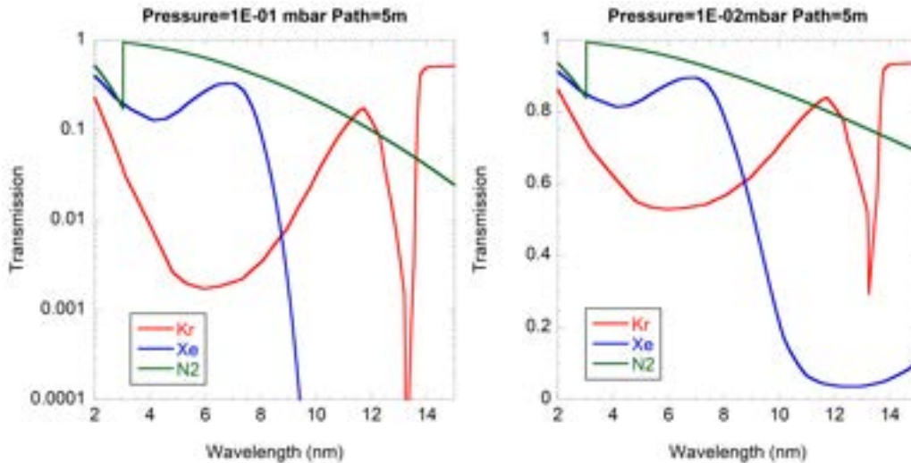
Figure 9.8: Transmission for 0.1 mbar (left) and 0.01 mbar gas pressure in a 5 m gas cell for N_2 (green line), Kr (red), Xe (blue)
