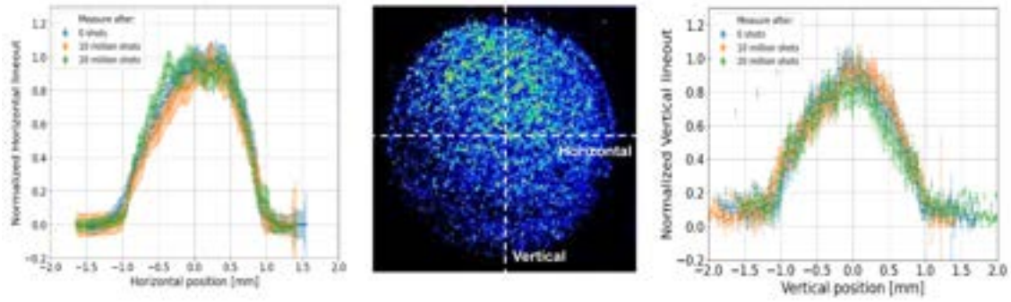
Figure 7.12: Measurement of the laser spot deformation as a function of the number of plasma discharges, up to 2 \times 10^7 shots, produced inside the gas-filled Shapal capillary to assess its degradation.
