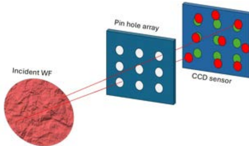
Figure 9.16: Schematic of the HWFS. Green dots on the detector plane correspond to the reference spot positions for a planar wavefront, while red dots indicate the displaced positions for an aberrated wavefront.
