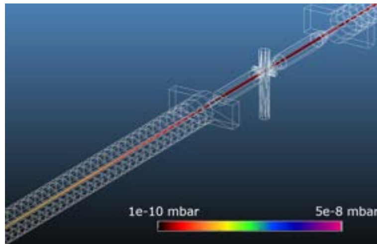
Figure 16.7: S-Band Linac: detail of pressure simulation in the area of the diagnostic chamber between 2 nd and 3 rd S-band accelerating structures
