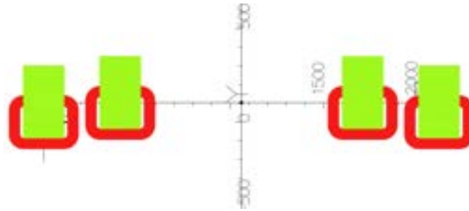
Figure 17.10: Top view of the 3D design of the magnets for the Laser Heater chicane.
