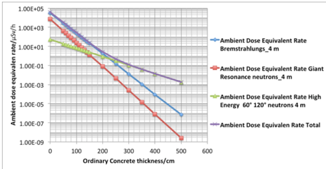
Figure 19.9: Ambient dose equivalent rate (4 m - 90°).
