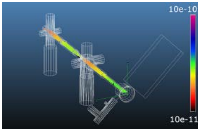
Figure 16.4: RF-gun Vacuum System: CAD Layout
