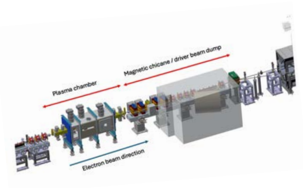
Figure 4.8: Layout of the area dedicated to plasma acceleration
