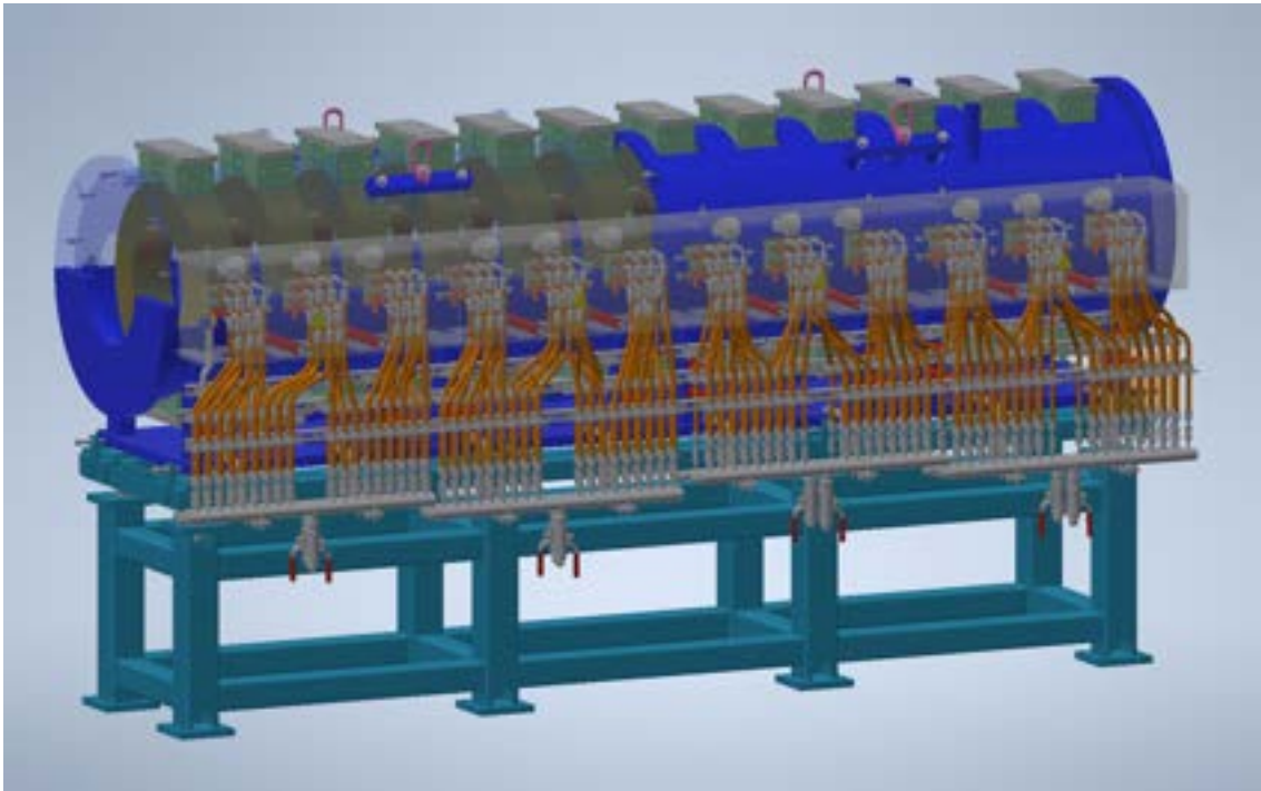
Figure 5.14: CAD view of the long solenoid foreseen to surround the first two S-band accelerating structures: coils and the iron yoke (blue shielding) are highlighted. The exploded layout highlights the arrangement of the coils.
