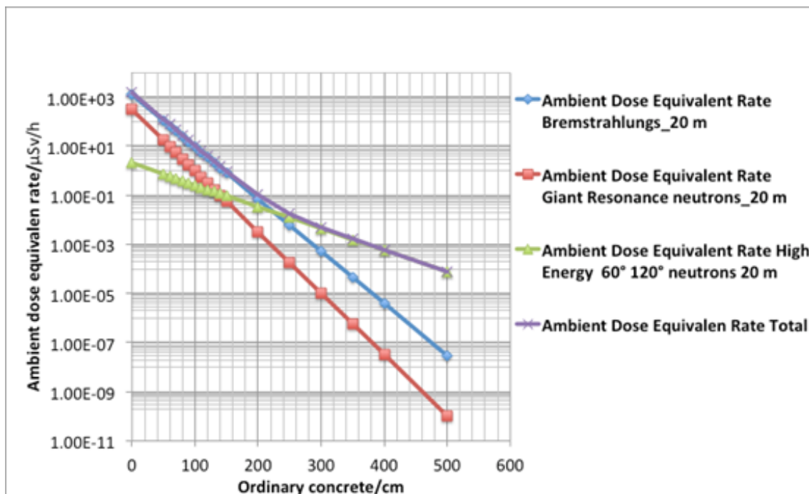
Figure 19.10: Ambient dose equivalent rate (20 m - 90°).
