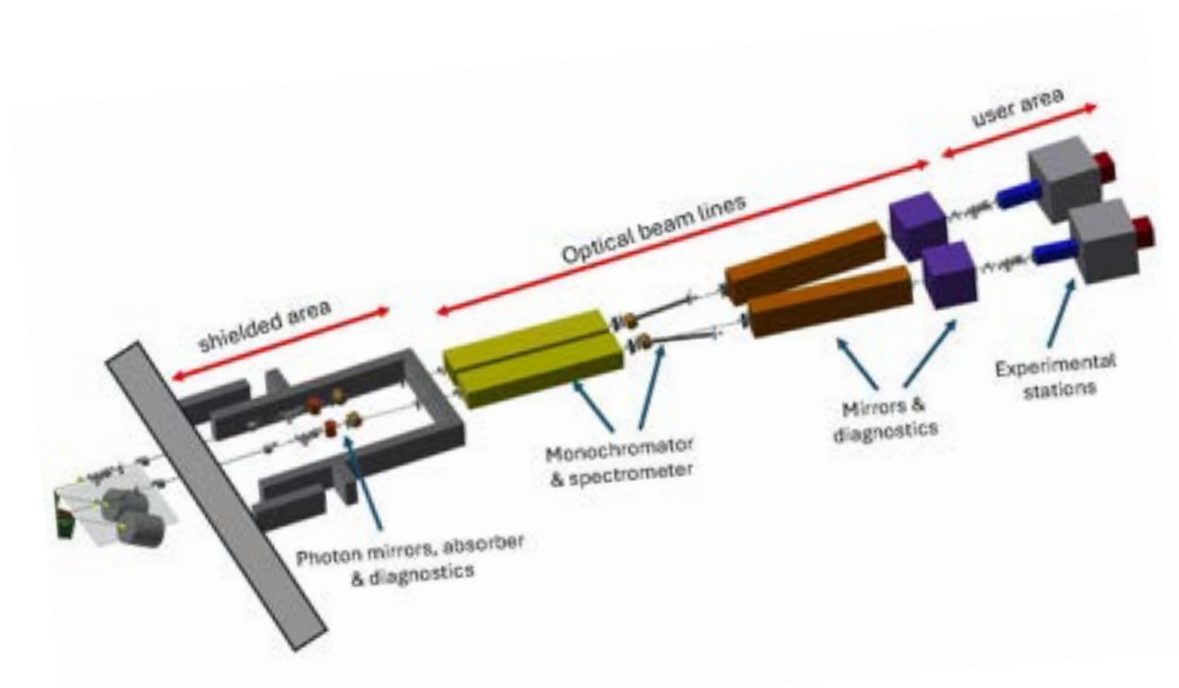
Figure 4.10: Schematic layout of the FEL beamlines and experimental stations
