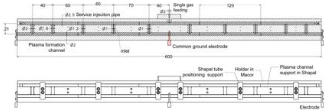
Figure 7.5: Design of the 60 cm long discharge capillary, composed of an external holder, connected to the gas injection pipe and the electrodes, and an internal support structure, into which the gas injectors and the plasma confinement channel are created.
