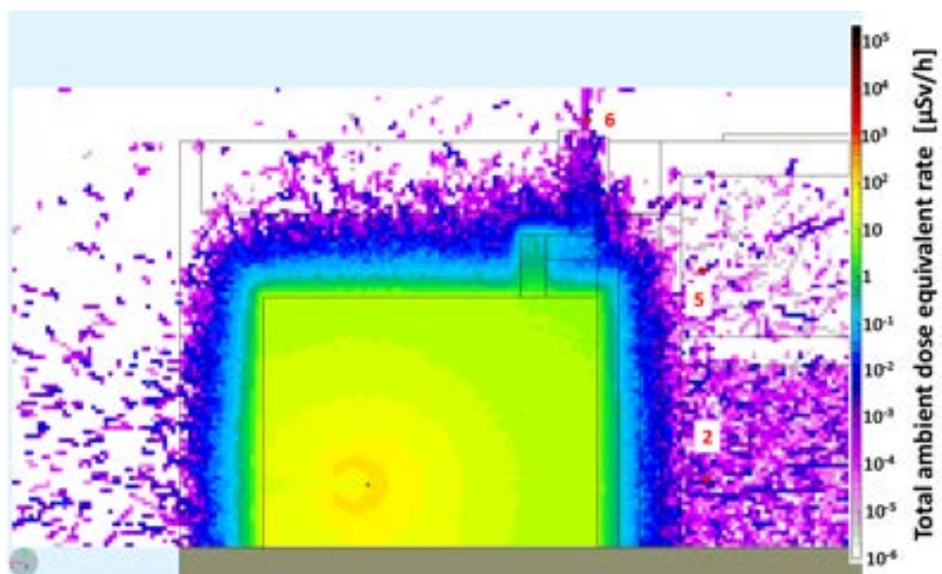
Figure 19.15: H^*(10) - 300 MeV diagnostic beam dump - xy plane.
