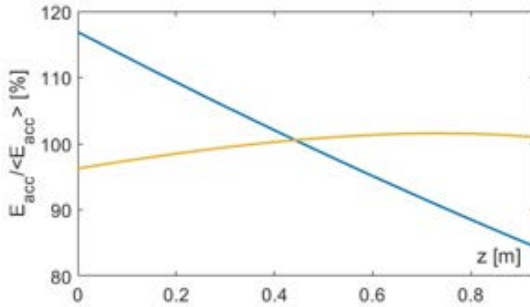
Figure 6.7: Peak accelerating field in each cell in case of constant impedance (blue curve) and tapered irises (yellow curve) structures (in the two cases the energy gain per structure is the same).
