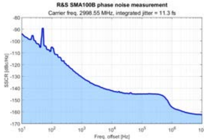
Figure 14.3: SSB PSD of Rohde & Schwarz ® SMA100B microwave signal generator [3] (with ultra low noise option) and its timing jitter from integrated between 10 Hz and 10 MHz from the carrier
