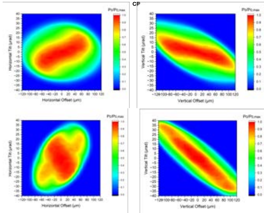
Figure 8.44: FEL emission from the nominal electron bunch with \beta_T = 8 m (top line) and \beta_T = 5 m (bottom line). Maximum achievable radiation power level P_0 for a given transverse misalignment, normalized to the maximum FEL power P_{0,max} achieved along the undulator line in the whole range of explored misalignments in circular polarization (CP) as a function of the initial horizontal (left) and vertical (right) tilt angles ( \mu\text{rad} ) and offsets ( \mu\text{m} ).
