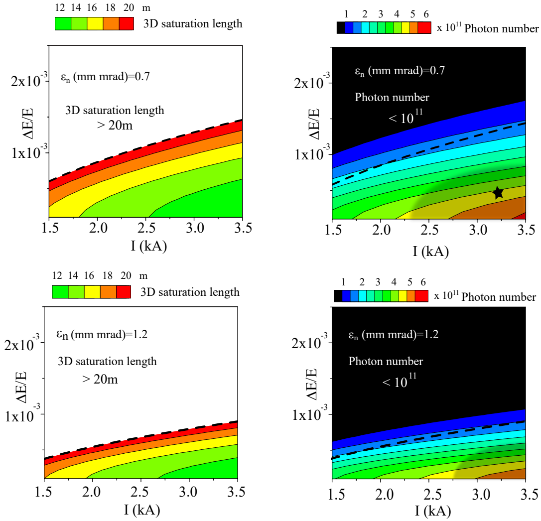
Figure 3.1: FEL saturation length and number of photons: Q = 30 pC, E = 1 GeV, K_{rms} = 0.84 , \lambda = 4 nm for normalized emittance \epsilon_n = 0.7 mm mrad (top figures), \epsilon_n = 1.2 mm mrad (bottom figures). Left figures: saturation length (evaluated as 20 times the three-dimensional gain length) mapped in the plane I(A) vs. \Delta E/E . In the white region, the saturation length is larger than 20 m. The dotted black line indicates the edge of the 20 m. Right figures: photon number per shot. In the black region the number of photons is less than 10^{11} . The black dotted line is the limit of saturation length equal to 20 m. The star in the top-right window is the start to end simulated working point for the plasma acceleration configuration, referring as well to Fig. 8.10.
