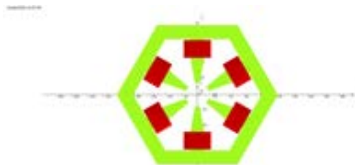
Figure 17.12: Front view of the 3D design of the sextupole for the Laser Heater chicane.
