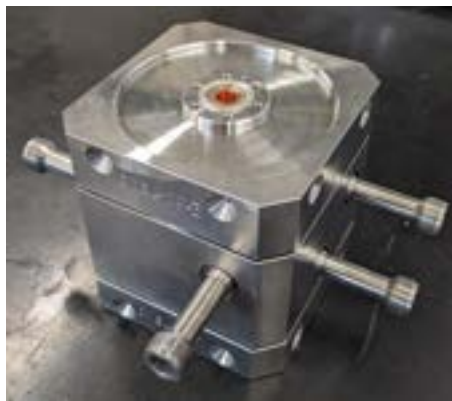
Figure 11.4: Cavity BPM PSI model "BPM8".
