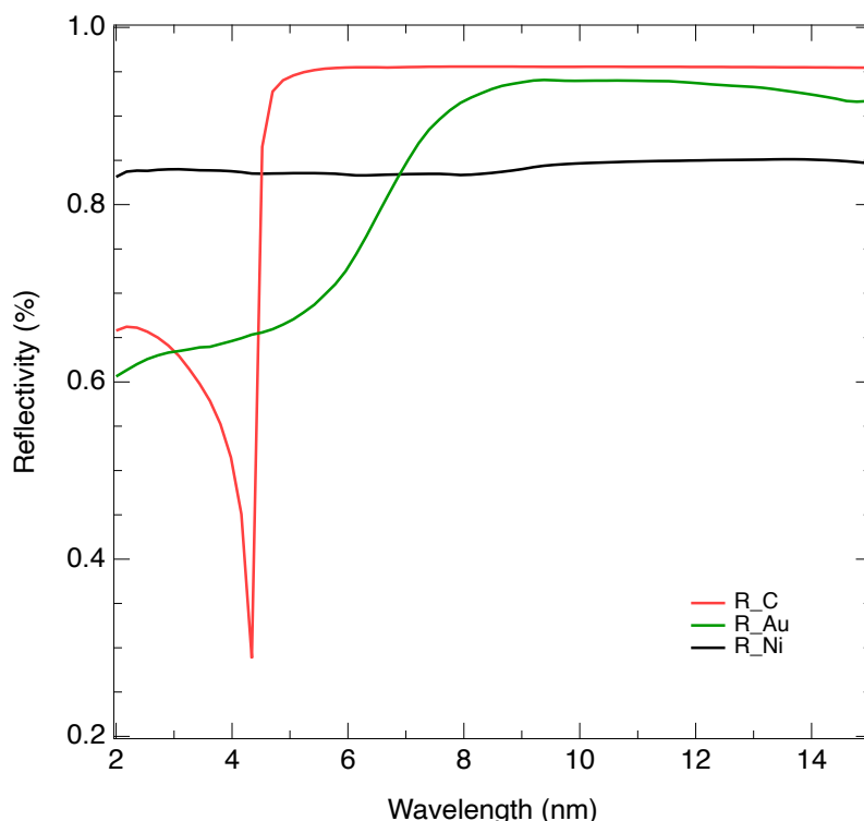
Figure 9.10: Mirror reflectivity as function of the wavelength at 88° angle of incidence under ideal conditions (no roughness, no contamination).
