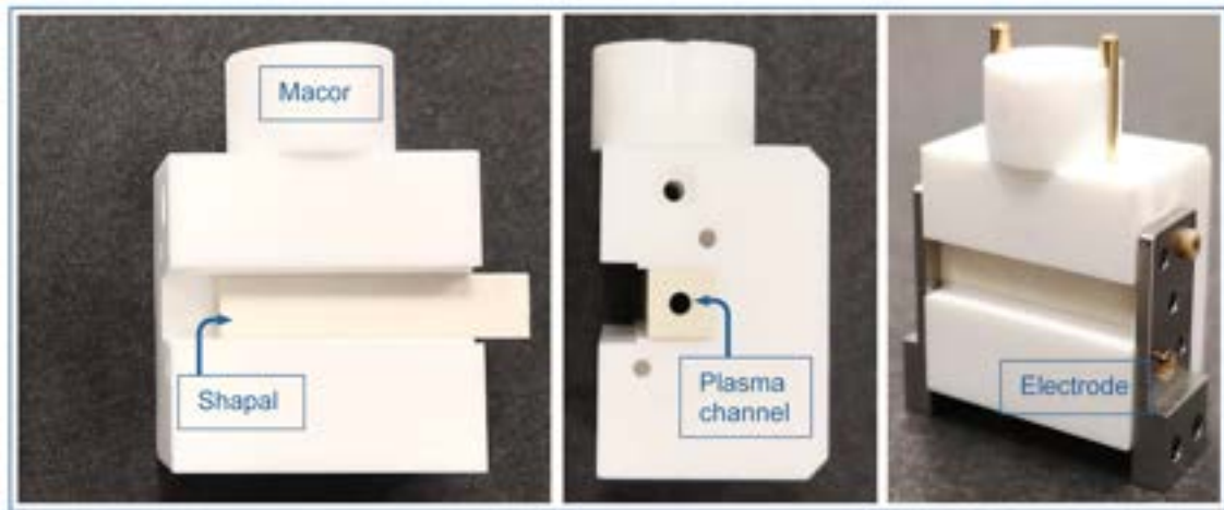
Figure 7.10: Image of basic elements that make up the test sample of the gas-filled discharge capillary for high repetition rate operation. The holder is composed of Macor ceramic and the support for the plasma formation channel is made of Shapal ceramic. The plasma formation channel is 30 mm in length and 2 mm in diameter.
