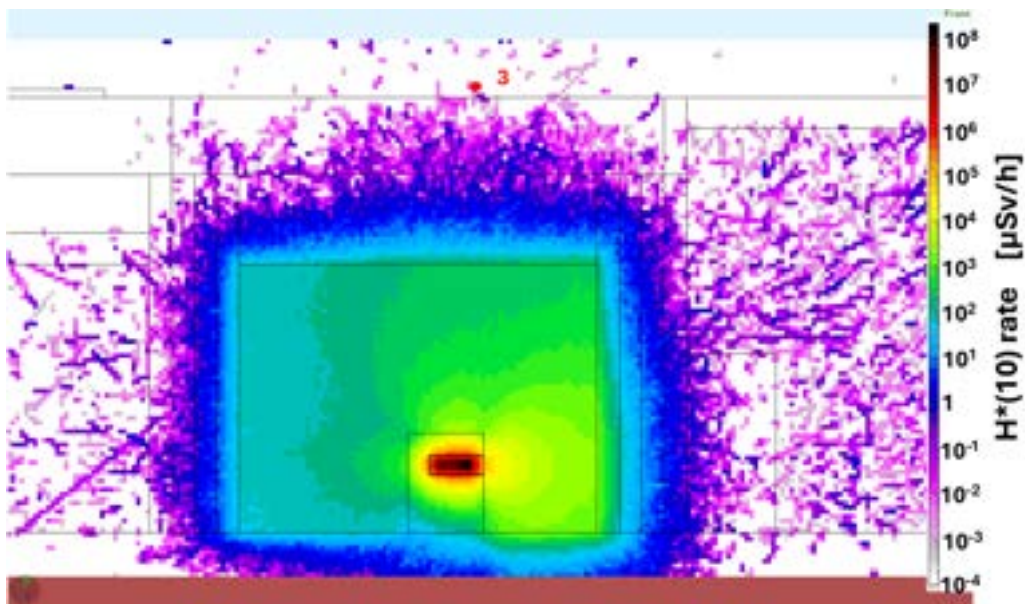
Figure 19.27: H^*(10) - driver beam dump - xy plane
