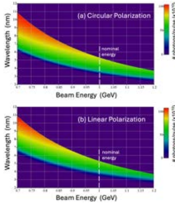
Figure 8.4: Photon count per pulse as a function of both resonant wavelength and beam energy, assuming an APPLE-X type undulator with a minimum magnetic aperture of 6 mm, a minimum gap of 1.5 mm, and B_r = 1.35 T. Panel (a) shows results for circular polarization, while panel (b) shows results for linear polarization. The conservative beam parameters of Table 8.1 and a pulse duration of \sim 15 fs (FWHM) have been assumed.
