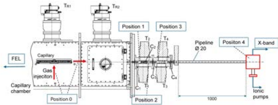
Figure 7.19: Sizing of the vacuum pumping system under the most stringent conditions near the X-band, based on continuous nitrogen gas injection for plasma production in a 60-cm long capillary.
