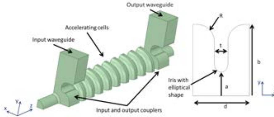
Figure 6.5: HFSS model of the X-band accelerating structure (reduced number of cells).
