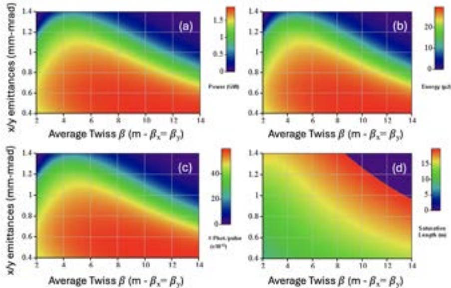
Figure 8.7: The four panels represent the dependence of the peak power (a), the pulse energy (b), the number of photons per pulse (c) and the saturation length (d) as functions of the transverse normalised emittances and the average \beta_T . The undulator is in circular polarisation, the energy spread and peak current are the one of Table 8.1.
