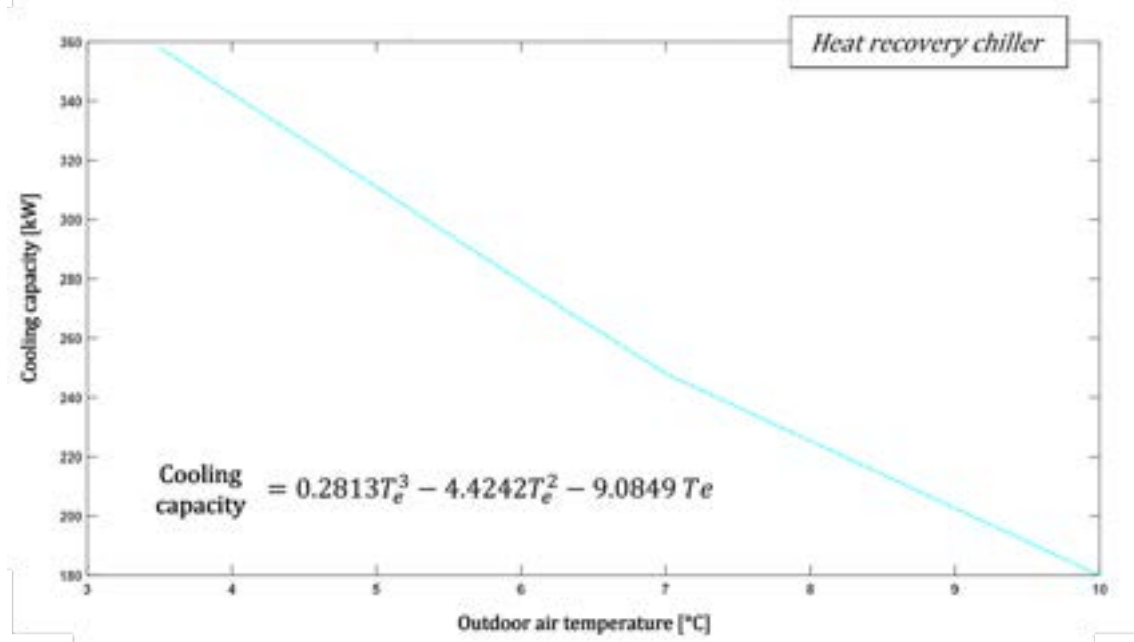
Figure 21.6: Cooling capacity depending on outdoor air temperature, free cooling operating mode
