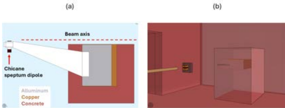
Figure 19.24: Driver beam dump layout 2D (a) and 3D (b).
