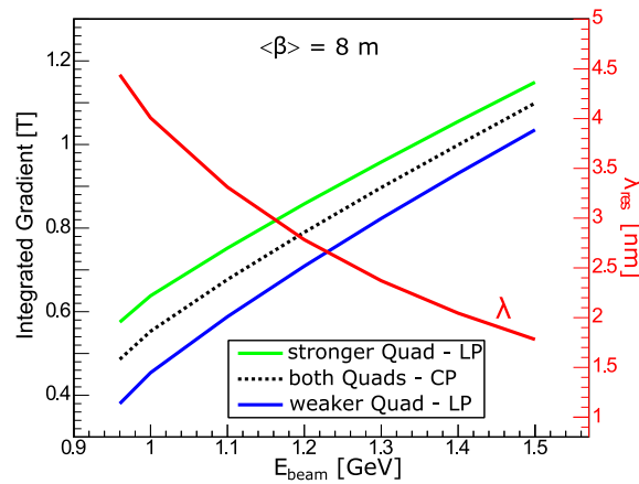
Figure 8.14: Quadrupole Integrated gradient as a function of beam energy with a Twiss \beta = 8 m, for both LP and CP configurations, superimposed to the achievable wavelength \lambda as a function of the electron beam energy. Calculated for \lambda_u = 18 mm, K_{rms} = 0.84 .
