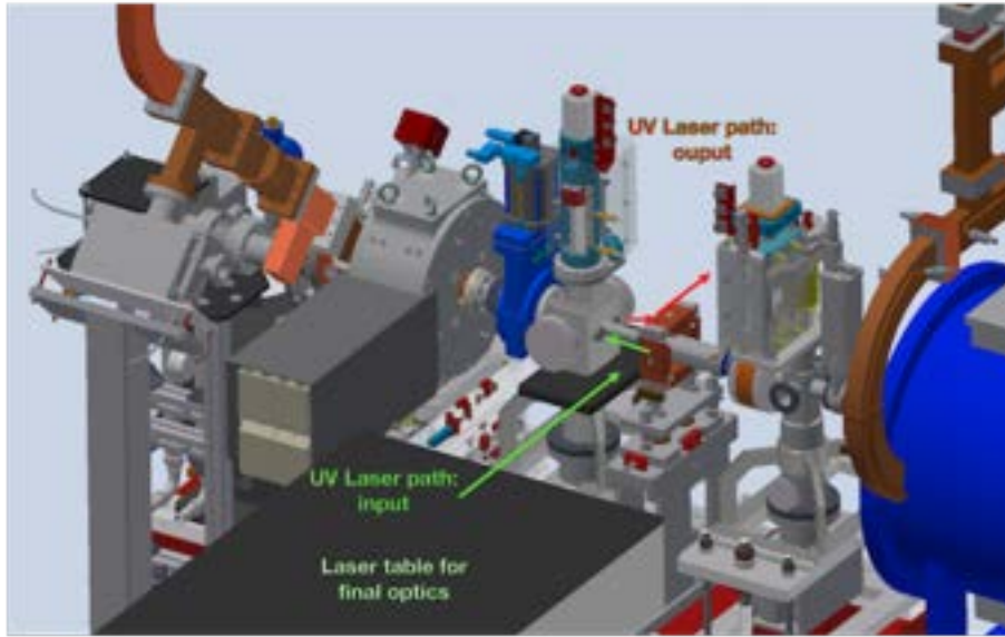
Figure 5.2: Prospective view of the laser injection scheme.
