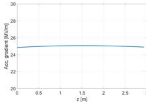
Figure 13.3: Quasi-constant accelerating gradient across the 3 m structure.
