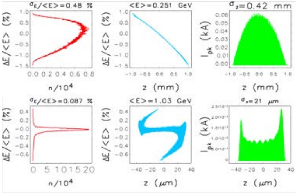
Figure 3.25: Full Rf case with purely magnetic compression: Energy (left column), longitudinal phase space (center column), and axial e-beam distributions (right column) at the photoinjector exit (above), and at undulator entrance (below), obtained with Tstep-Elegant simulation of 3.2 M macroparticles.
