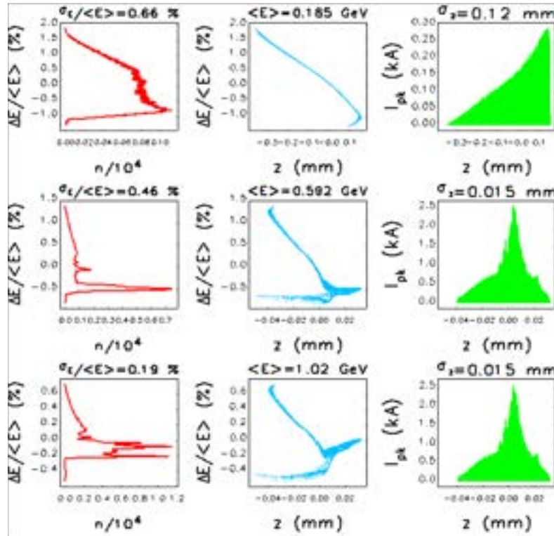
Figure 3.21: Electron beam longitudinal phase space evolution through the linac (Full RF case): Energy (left), longitudinal phase space (center) and axial (right) e-beam distributions after Photoinjector (top), after BC chicane (center row) and at undulator entrance (bottom), as obtained with Tstep-Elegant simulation of 400k macroparticles.
