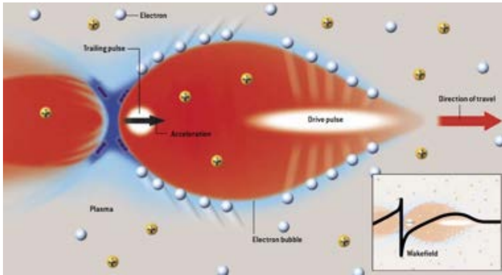
Figure 1.1: Plasma wakefield accelerators rely on charge separation in the plasma sustaining fields known as a wakefield. The drive bunch blows the electrons (blue) away from axis, leaving behind a region of positive charge (red). Along the axis where the bunches propagate, the electric field (plotted in the little box) causes the drive bunch to lose energy, and a trailing pulse of electrons injected near the rear of the bubble to experience strong acceleration [24].
