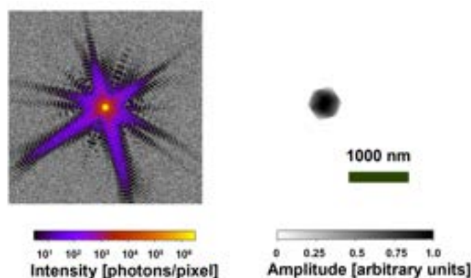
Figure 2.3: Simulated, ideal CDI diffraction pattern of a poliovirus. The simulation was performed using the Condor software [49], assuming the FEL beam parameters expected at AQUA, namely 10^{11} photons per pulse at a wavelength of 4.3 nm, focused onto a 5\ \mu\text{m} spot size. Gaussian (detector readout) and Poisson (FEL shot) noise were added to emulate experimental conditions.
