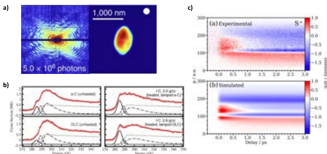
Figure 2.1: Literature examples corresponding to the scientific areas described above. a) Diffraction pattern and reconstructed electron density of an aerosolised living cyanobacterium. Image adapted from [22] b) TR-XAS measurements on liquid carbon reveal changes in bonding structure and bond length under varying densities, providing insights into its behavior as warm dense matter. Image adapted from [23]. c) Time-resolved Coulomb explosion imaging of photoexcited CS 2 using soft X-ray pulses. Image adapted from [24].
