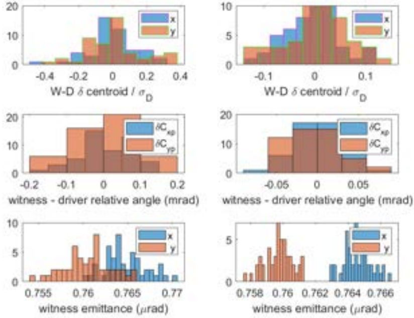
Figure 3.16: Witness-driver relative offset (top row), relative angle (middle row), and witness beam emittance (bottom row) at the plasma entrance, before (left) and after (right) the Beam-Based Alignment procedure.
