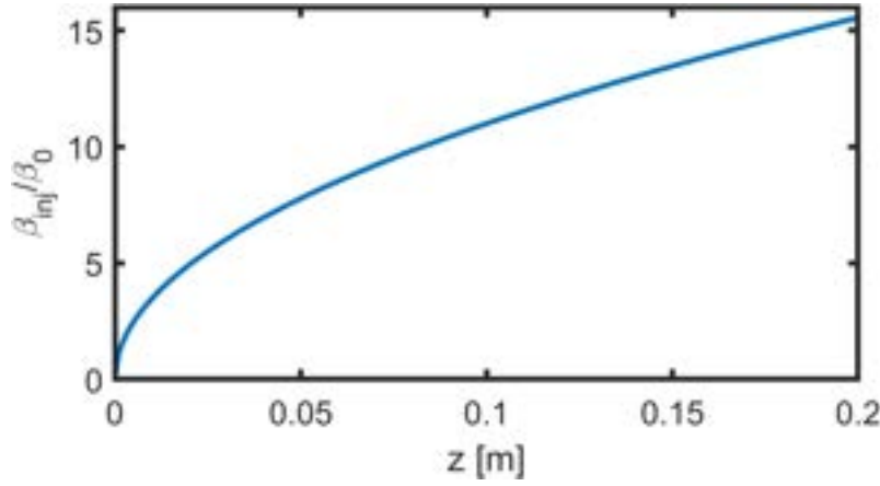
Figure 3.7: Normalized optimal \beta -function at the entrance of a plasma ramp, expressed as a function of the ramp length. The \beta -function is normalized to the matched value at the peak plasma density, \beta_0 . In this evaluation, the bunch has a Lorentz factor of \gamma = 1000 and is assumed to be injected into a plasma channel with a peak density of n_p = 10^{16} \text{ cm}^{-3} .
