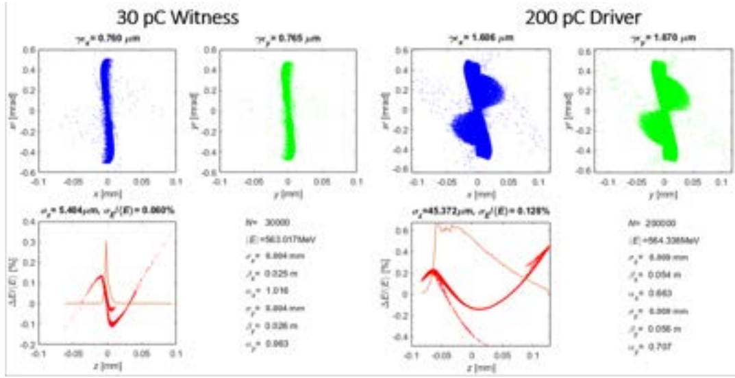
Figure 3.6: Longitudinal and transverse phase space of the electron beam at the plasma injection for the reference working point as obtained with TStep and Elegant codes.
