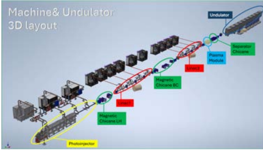
Figure 3.2: The layout of the EuPRAXIA@SPARC_LAB accelerator
