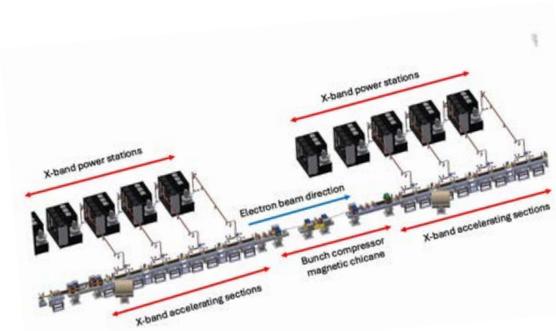
Figure 4.7: Layout of the X-band accelerator
