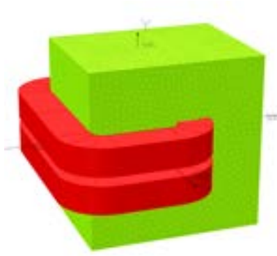
Figure 17.18: The 3D design of C-shaped dipoles for the driver-witness separator chicane.
