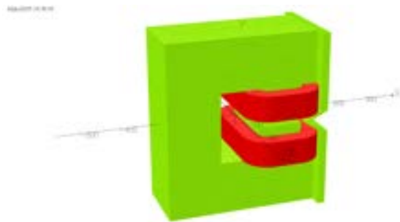
Figure 17.20: The 3D design of the septum dipole.
