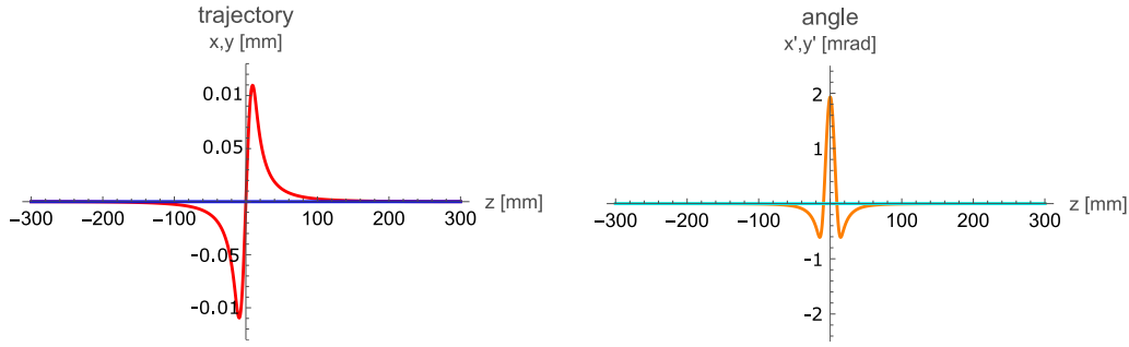
Figure 8.39: Trajectory and kick angle of a electron entering in the phase shifter with null offset and angle at minimum gap. Since the planar geometry, one electron oscillates, and its angle varies, only in the horizontal plane.
