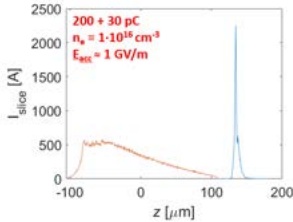
Figure 3.4: Electron beam longitudinal profile (PWFA case) in terms of slice current as obtained with TStep for the 200+30 pC comb beam.
