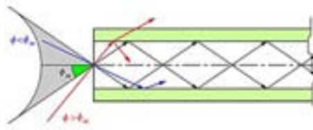
Figure 11.25: Cherenkov UV light propagates along the fiber if the incidence angle is smaller than the critical angle (blue line). Otherwise, the light is lost (red line).
