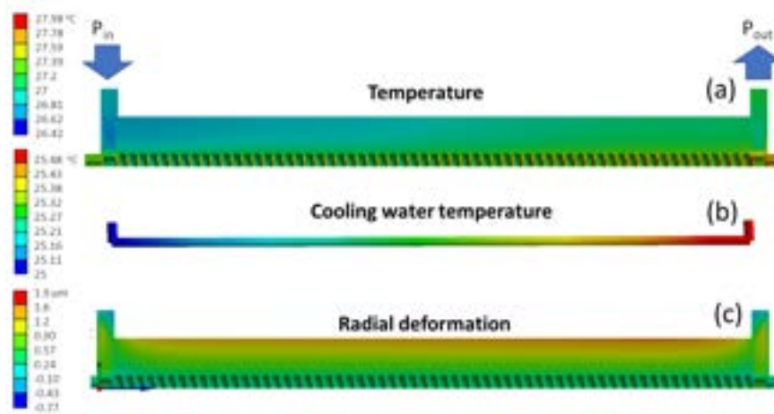
Figure 6.9: Results of the thermo-mechanical analysis performed by ANSYS (model with a reduced number of cells).
