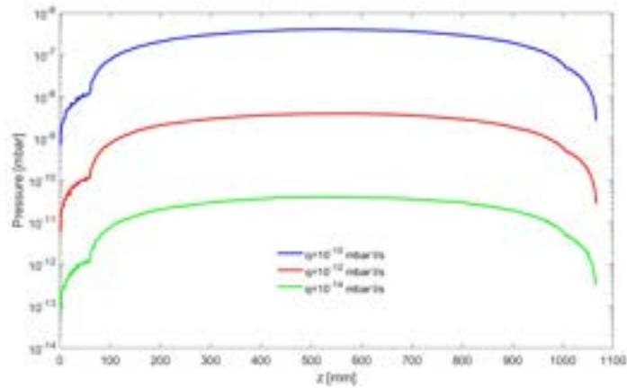
Figure 6.10: Simulated pressure along the X-band structure assuming different specific outgassing rates for copper (in \text{mbar}/\text{l}/\text{sec}/\text{cm}^2 ).
