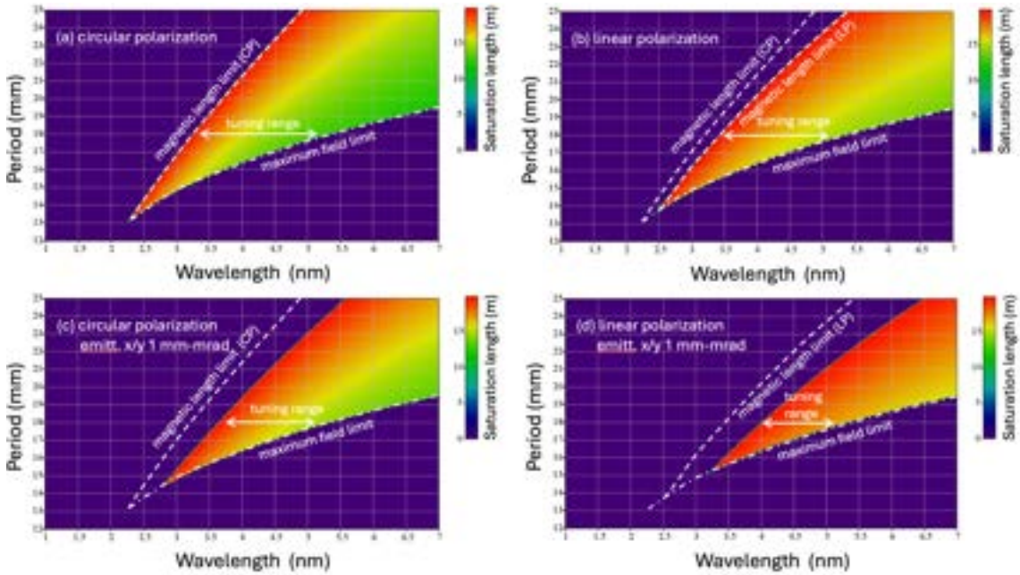
Figure 8.3: FEL saturation length vs. period length and undulator resonant wavelength. The parameters of an APPLE-X undulator with minimum magnetic aperture of 6 mm ( B_r = 1.35T ) have been assumed. In (a) and (c) the polarization is circular; in (b) and (d) the polarization is linear. In (a) and (b) the beam parameters are those in Table 8.1. In (c) and (d) the slice x/y emittances are increased to 1.0 mm-mrad.
