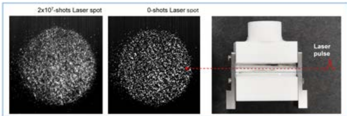
Figure 7.11: Comparison of laser spots to assess the deterioration of gas-filled discharge capillary made in Macor-Shapal ceramics before and after performing 2 \times 10^7 shots at up to 150 Hz.
