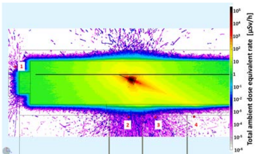
Figure 19.14: H^*(10) - 300 MeV diagnostic beam dump - xz plane.
