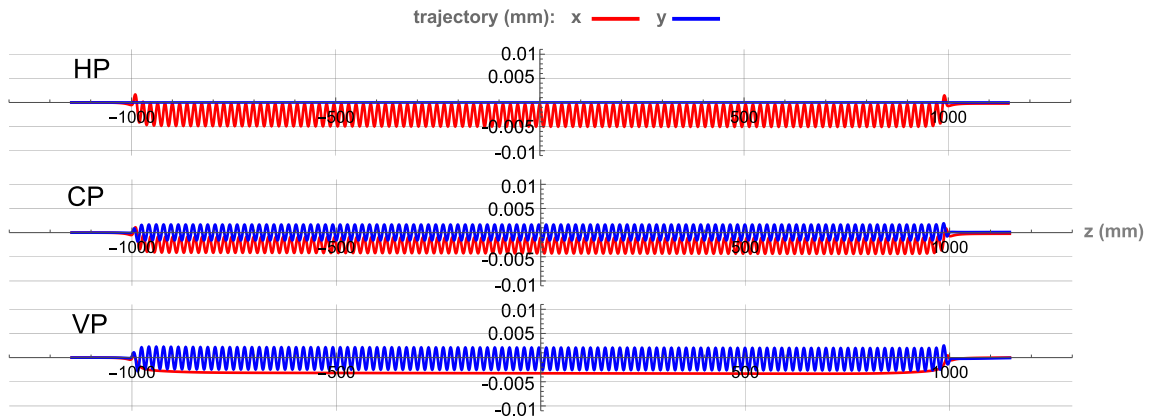
Figure 8.26: Corrected trajectory by means of the Correction Coils system. The three cases of linear Horizontal (HP), Circular (CP) and linear Vertical (VP) polarization mode are plotted.
