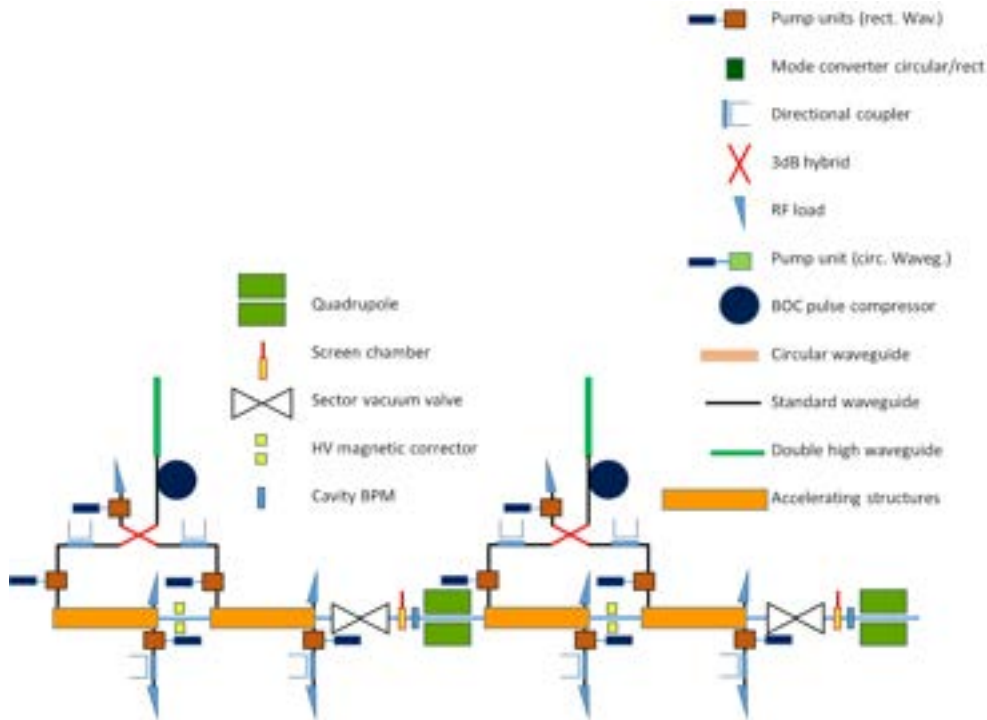
Figure 6.4: Schematic layout of two consecutive modules.
