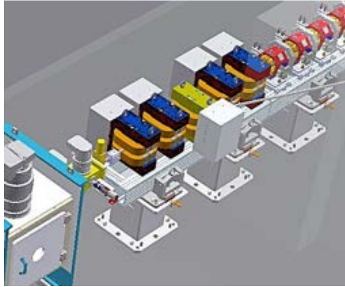
Figure 7.17: Layout of the chicane line where the energy-depleted driver is spatially separated from the witness beam. The driver is then transported up to the beam dump.
