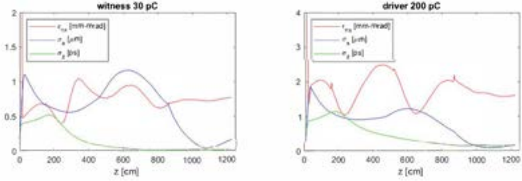
Figure 3.3: Evolution of the electron beam transverse normalized emittance (red line), spot size (blue line) and bunch length (green line) of the witness and driver, respectively, from the cathode to the photoinjector exit as obtained with the TStep code for the PWFA case. The picture shows the control on the transverse emittance value through all the RF compression process in the photoinjector that leads to the desired bunch length, at the same time optimizing the beam transverse envelope.
