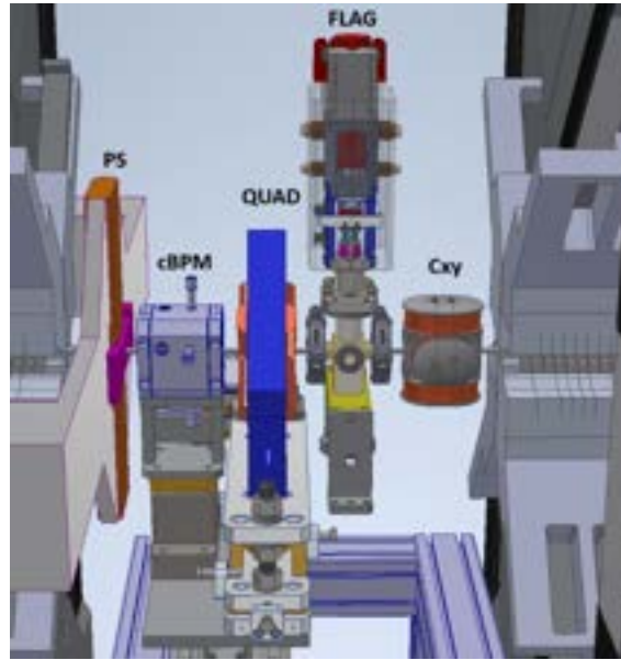
Figure 8.56: Intra-undulator section elements. From left to right: phase shifter (PS), cavity BPM (cBPM), quadrupole (QUAD), photons diagnostic chamber (FLAG) and steerers (Cxy).
