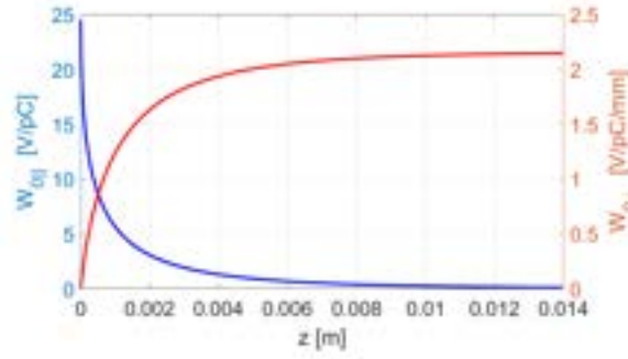
Figure 3.5: X-band longitudinal and transverse wakefield calculated for an average iris radius of 3.5 mm and a cell length of 8.332 mm.
