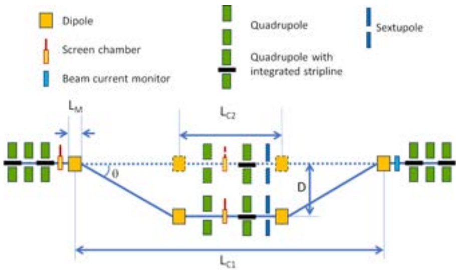
Figure 6.21: Schematic layout of the magnetic chicane.
