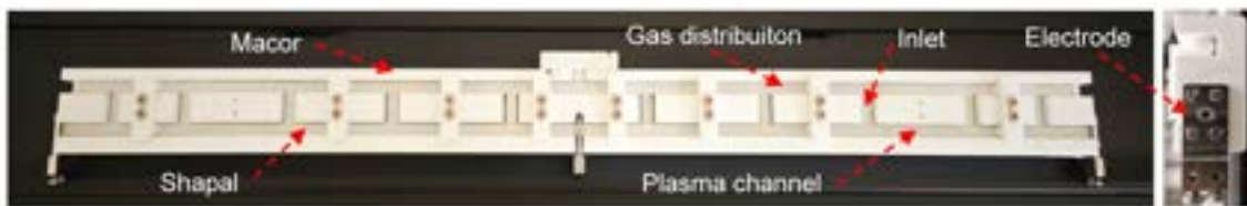
Figure 7.8: Final construction of the gas-filled discharge capillary in Shapal/Macor. The project is a copy of the prototype built in plastic, on which operational tests and characterization of the plasma properties were carried out.
