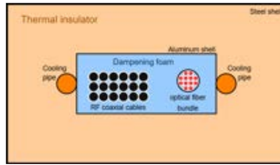
Figure 14.4: Conceptual cross-section design of the thermal-insulating vibration-dampening cable duct
