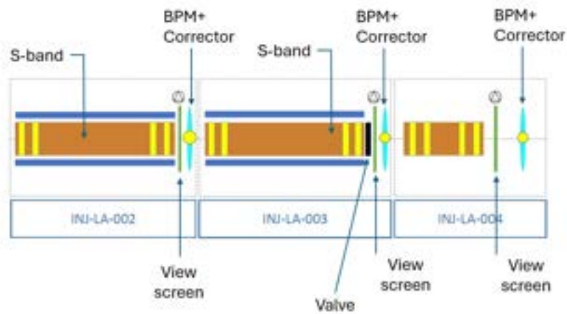
Figure 11.32: Diagnostics positions in the injector area INJ-LA-002-003.
