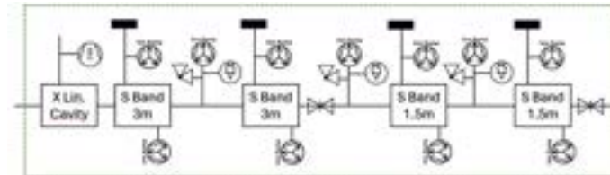
Figure 16.6: S-Band Linac: Schematic Vacuum Layout
