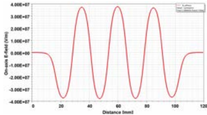
Figure 5.11: On-axis electric field profile.
