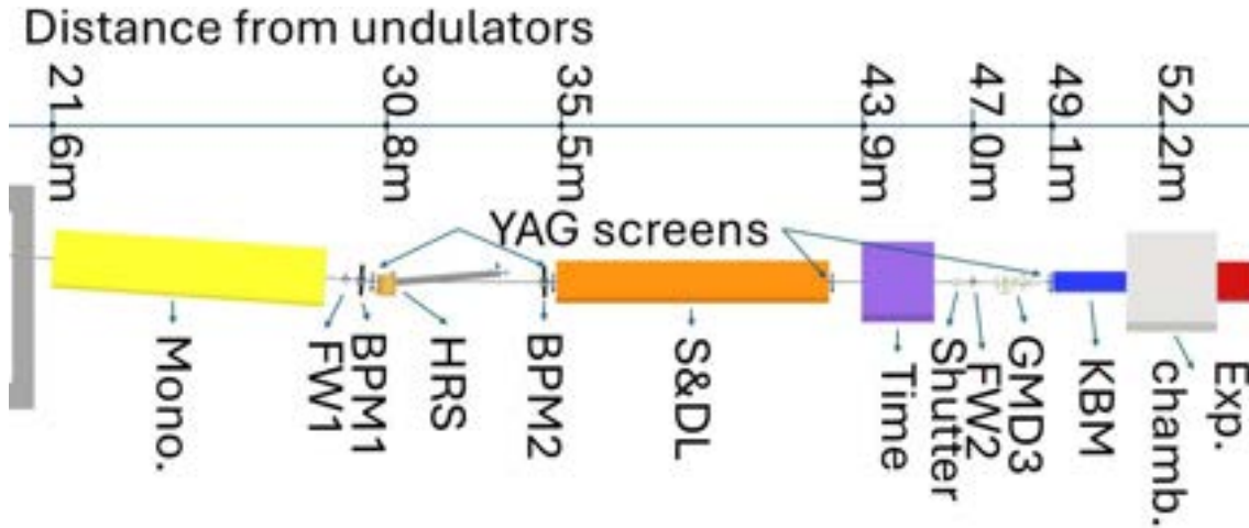
Figure 9.4: Details of the layout of the AQUA beamlines inside the user area (Fig. 9.1 view C). Mono.: monochromator area, FW: filter wheels, BPM: bladed beam position monitors, HRS: high resolution spectrometer, S&DL: split and delay line area, Time: time and polarization measurement area, Shutter: FEL photon shutter, KBM: K-B mirror chamber, Exp. chamb.: experimental chamber area.
