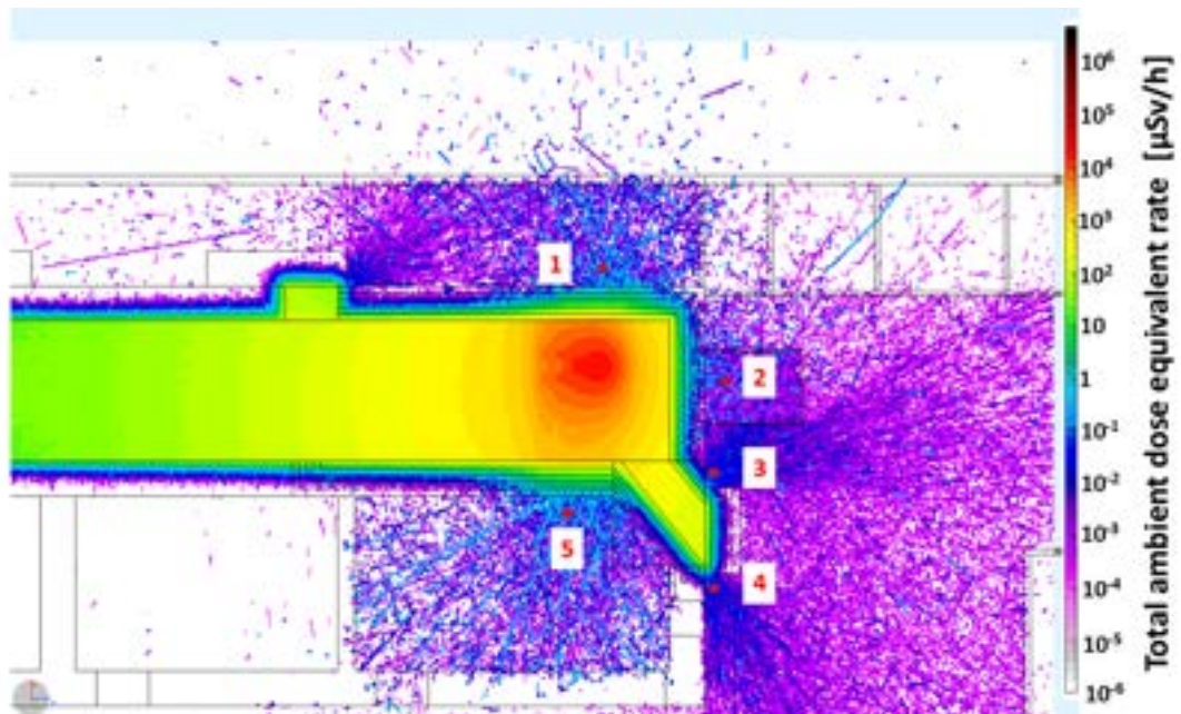
Figure 19.22: H^*(10) - FEL beam dump - without plasma acceleration - xz plane.
