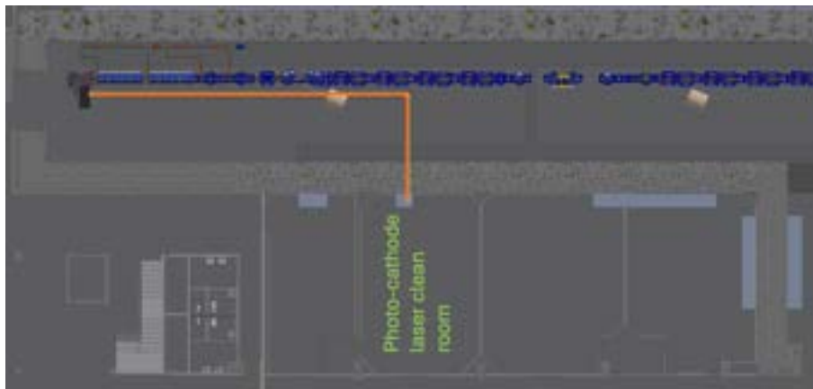
Figure 12.2: Transport beamline from cleanroom to cathode.
