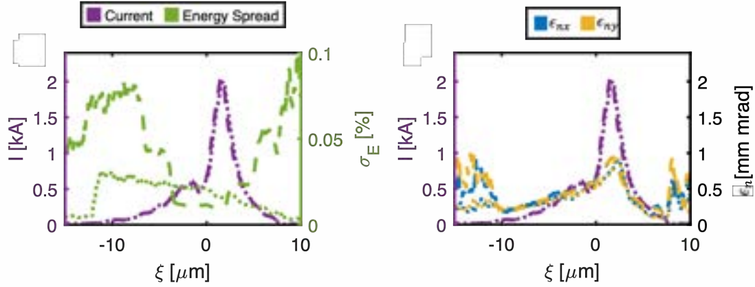
Figure 3.9: Slice analysis of the witness bunch at the injection (dots) and the extraction (dashed lines) of the plasma for the 30 pC charge reference working point: current and energy spread profile (left), transverse normalized emittance for both x,y planes (right). The coordinate \xi denotes the separation of the single slice centroid respect to the position of the longitudinal centroid of the witness charge distribution.
