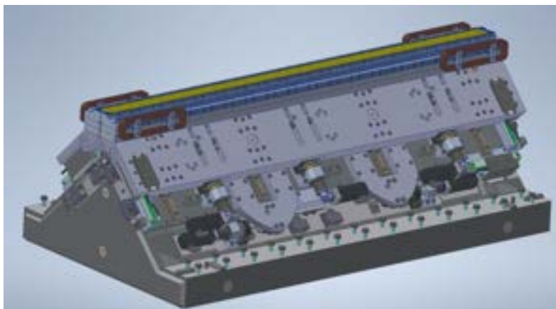
Figure 8.33: Undulator lower frame
