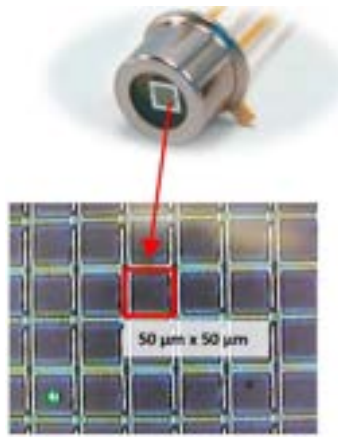
Figure 11.28: Hamamatsu MPPC sensor structure.
