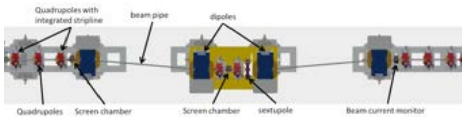
Figure 6.22: Layout of the magnetic chicane.
