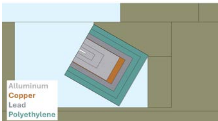
Figure 19.20: FEL Beam Dump (AQUA beamline) layout on yz plane.
