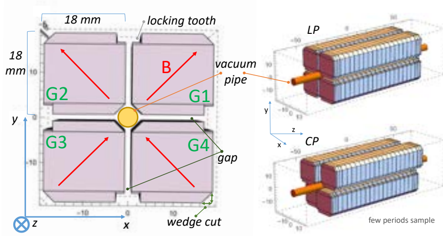
Figure 8.16: Structure of the AQUA APPLE-X undulator, transverse (left) and longitudinal (right) view. The positioning for the two linear (LP) and circular (CP) polarization modes are also plotted for a sample of few periods.
