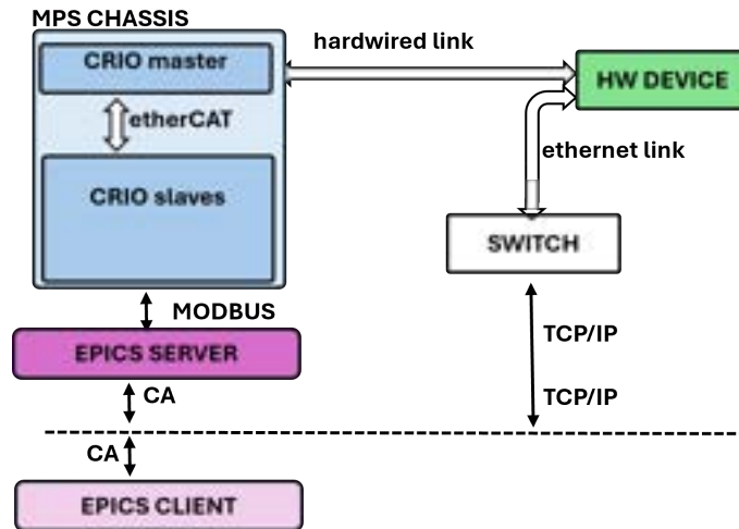
Figure 19.30: MPS Architecture
