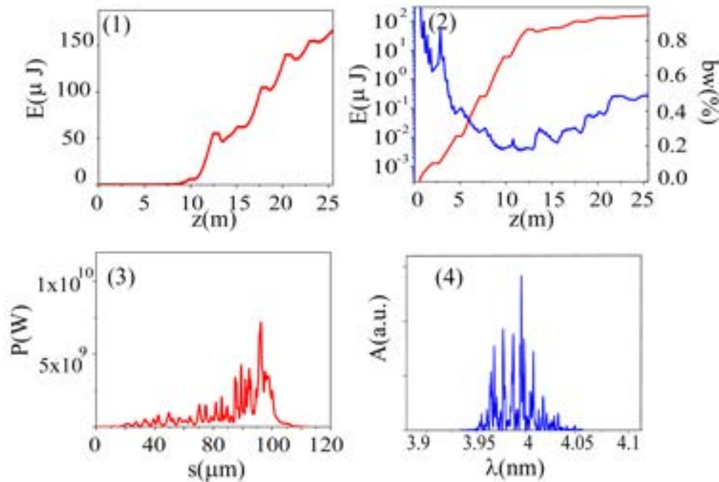
Figure 1.5: Genesis simulation results for Full RF working points with Undulator Tapering, Plot (1): energy growth in linear scale. Plot (2): energy growth in logarithmic scale and bandwidth in %. Plot (3): power distribution. Plot (4): a smplitude of spectral distribution.
