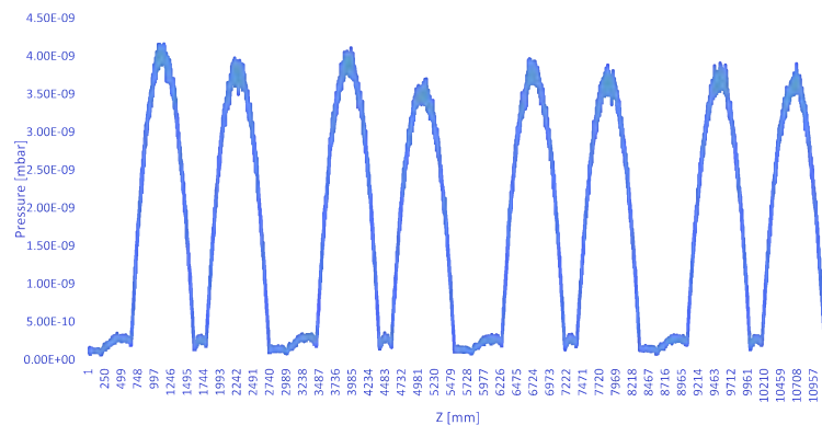
Figure 16.14: X-Band Linac: Simulation of Pressure Distribution
