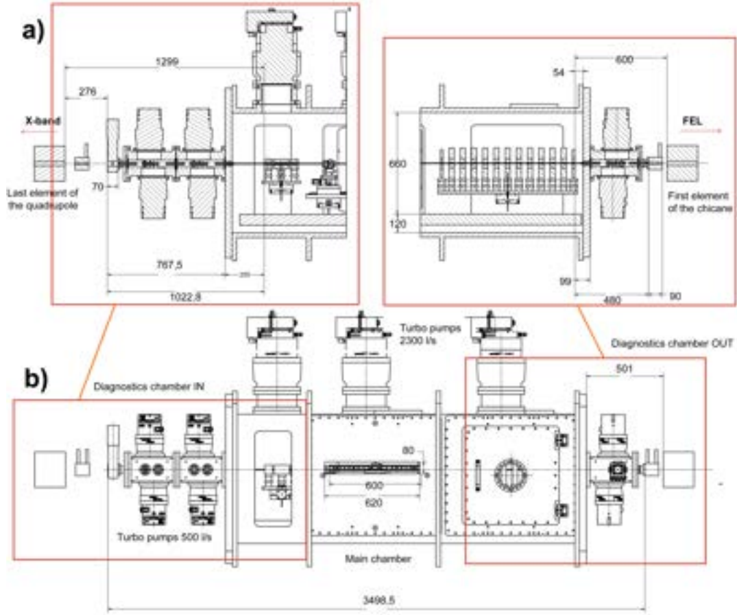
Figure 7.18: Plasma chamber and vacuum pumping system. a) Detailed view of the side chambers containing beam diagnostics and mounting part of the vacuum pumping system. b) Overview of the plasma chamber.
