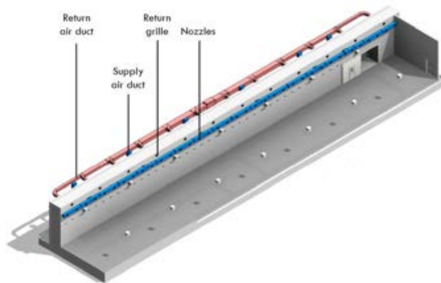
Figure 18.19: LINAC ventilation system.
