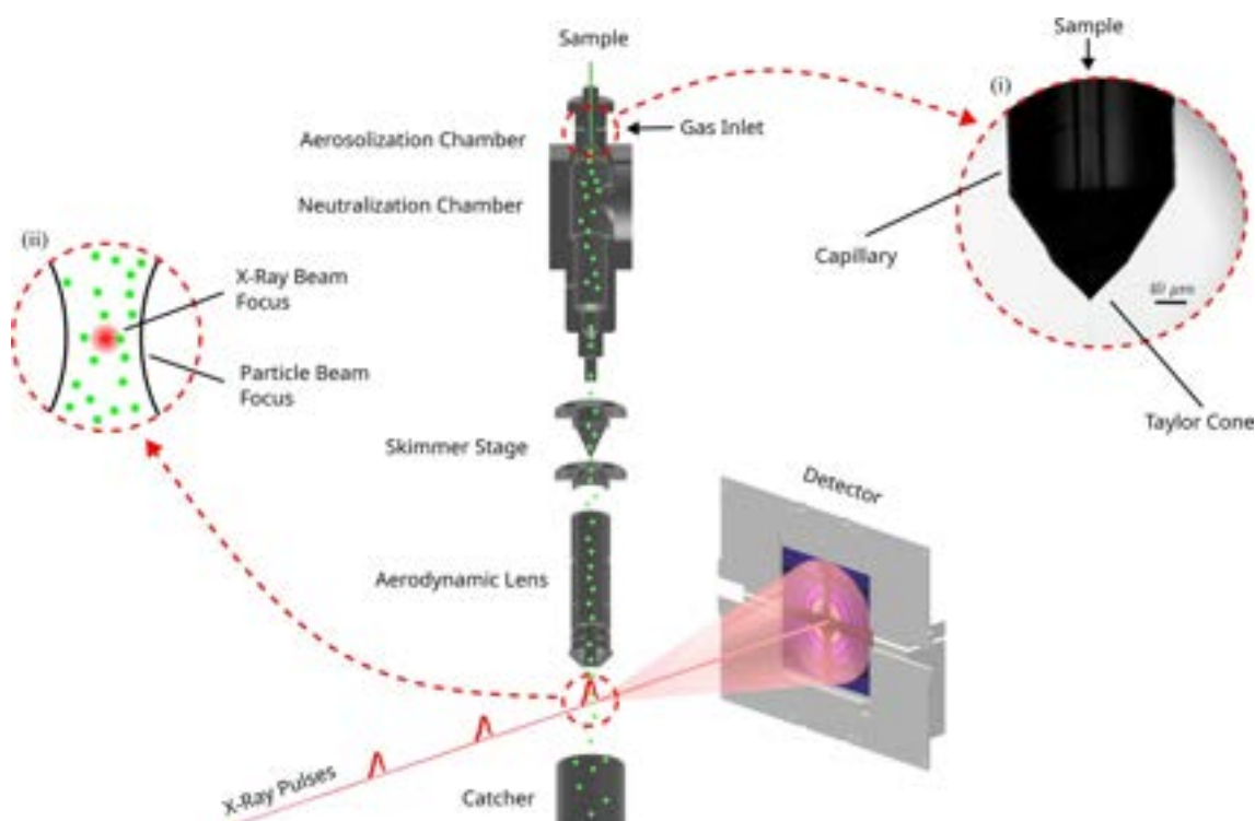
Figure 10.3: Schematic of the electrospray-based aerosol injector system used at the European XFEL for single-particle imaging. Image reproduced with permission from [23].
