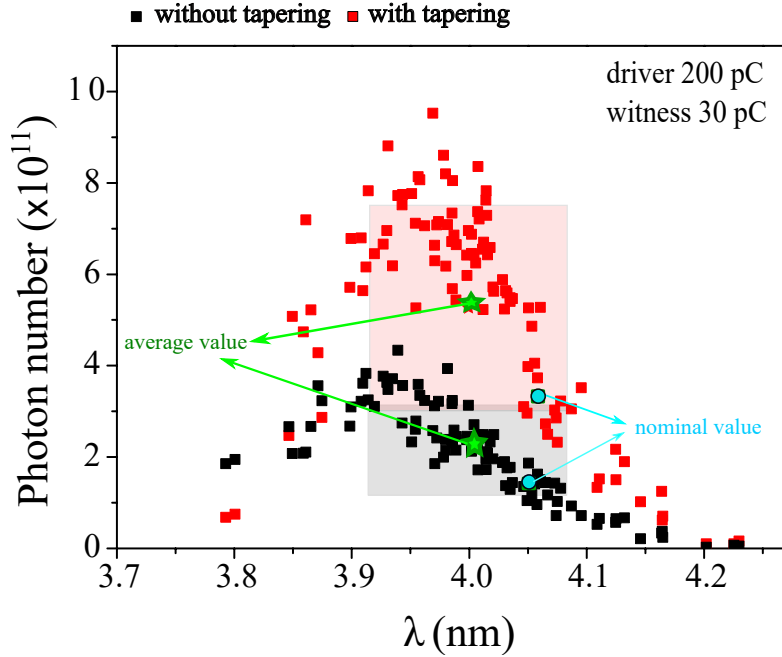
Figure 3.17: Photon number versus wavelength for 100 random events of the reference case at 1 GeV. Black squares: without tapering. Red squares: with a tapering with the K_{rms} values of Table 3.8. Green stars represent the average values. Cyan circles represent the values obtained with the nominal beams. The shaded areas (light gray for the case without tapering and light pink for the case with tapering) around the average values have the half height equal to the rms deviation of the photon number ( 1 and 2.33 \cdot 10^{11} ) and the half bases equal to the rms deviation of the peak wavelength (85 pm).
