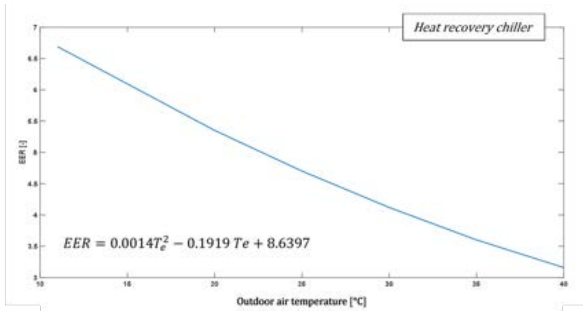
Figure 21.3: EER depending on outdoor air temperature (under peak load conditions), operating mode without free cooling
