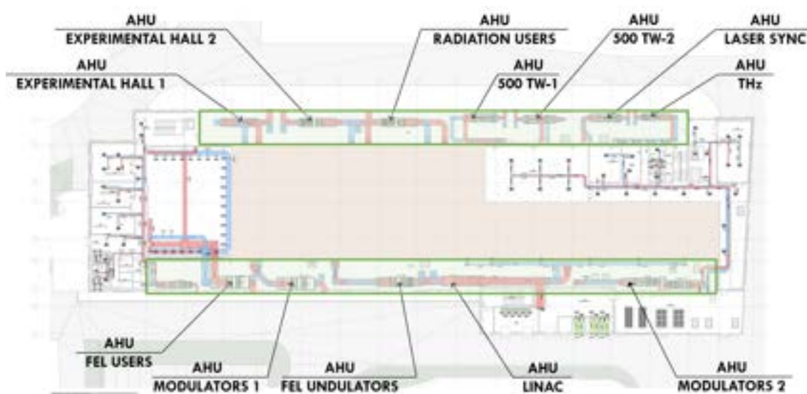
Figure 18.24: Technical balconies for AHUs.
