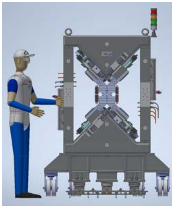
Figure 8.31: Rendering of one of the AQUA undulator modules. Front view.
