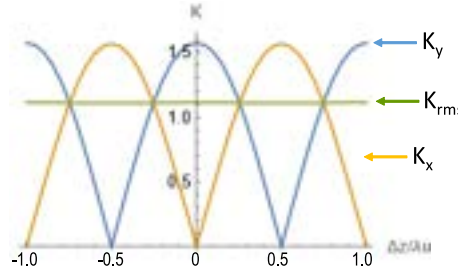
Figure 8.17: Undulator K parameter variation with different polarization setting given by a phase shift \Delta z in unit of \lambda_u , at the minimum gap 1.5 mm.
