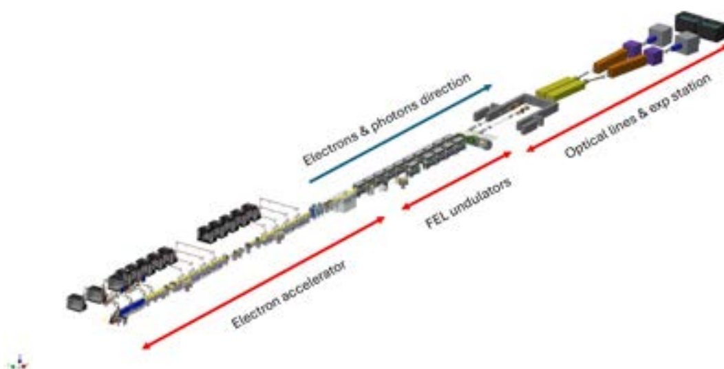
Figure 4.5: Layout of the accelerator and beamlines
