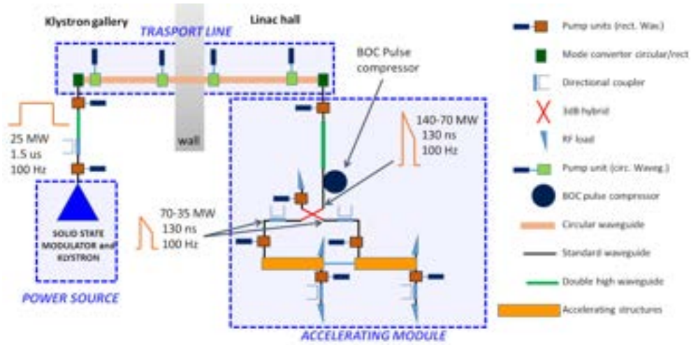
Figure 6.3: X-band RF module schematic layout.
