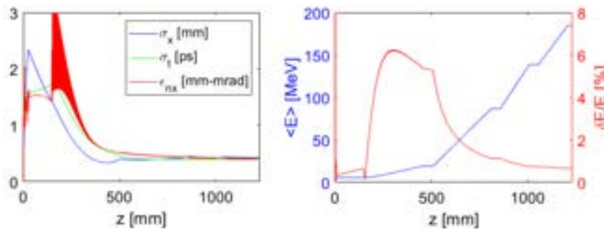
Figure 3.20: Electron Beam transverse phase space emittance and envelope (Full RF case). Left: evolution of transverse normalized emittance, spot size, and bunch length. Right: energy and energy spread along the beamline.
