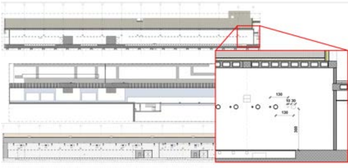
Figure 18.9: Layout and section views of the Experimental halls with systems ducts and penetrations.
