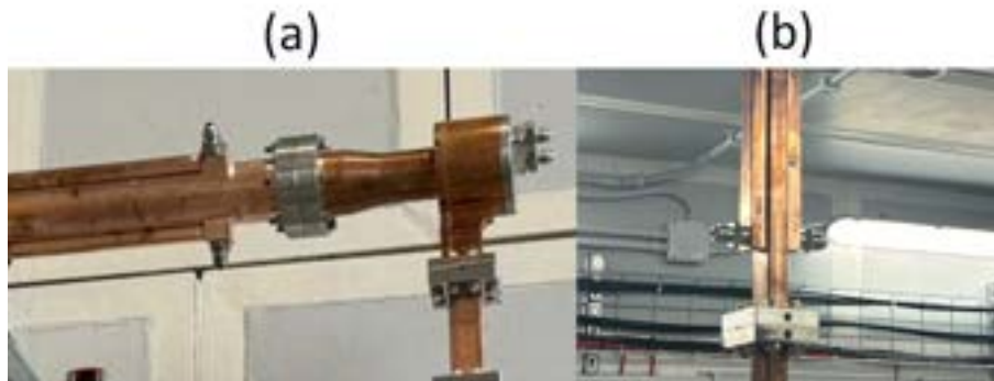
Figure 6.16: Detail of the cooling system of the circular (a) and rectangular (b) waveguides.
