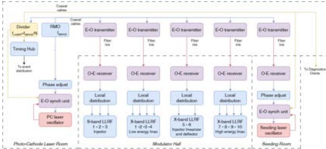
Figure 14.2: Layout of the synchronization system.
