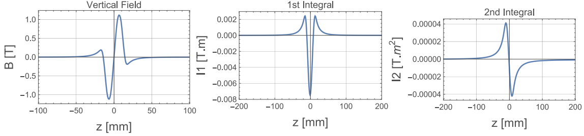
Figure 8.37: Vertical component of the field B_y , first and second field integrals for the AQUA phase shifter.
