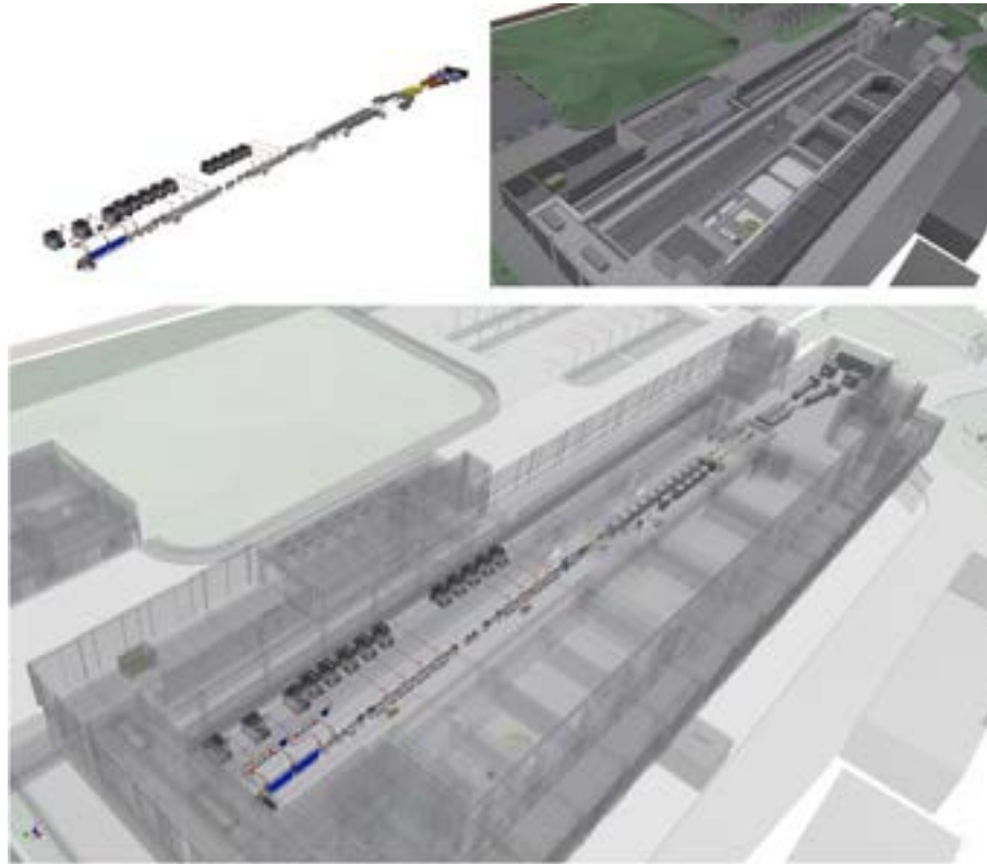
Figure 20.5: Top Left: Machine; Top Right: Civil Infrastructure; Bottom: Matching between Machine with Civil Infrastructure.
