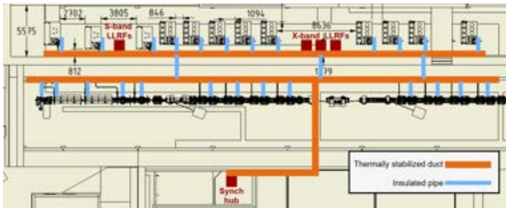
Figure 14.5: Conceptual network layout of the insulated ducts across the facility. This system is specifically designed to accommodate the coaxial cables and optical fibers utilized for both the reference signal distribution and the RF signal readbacks
