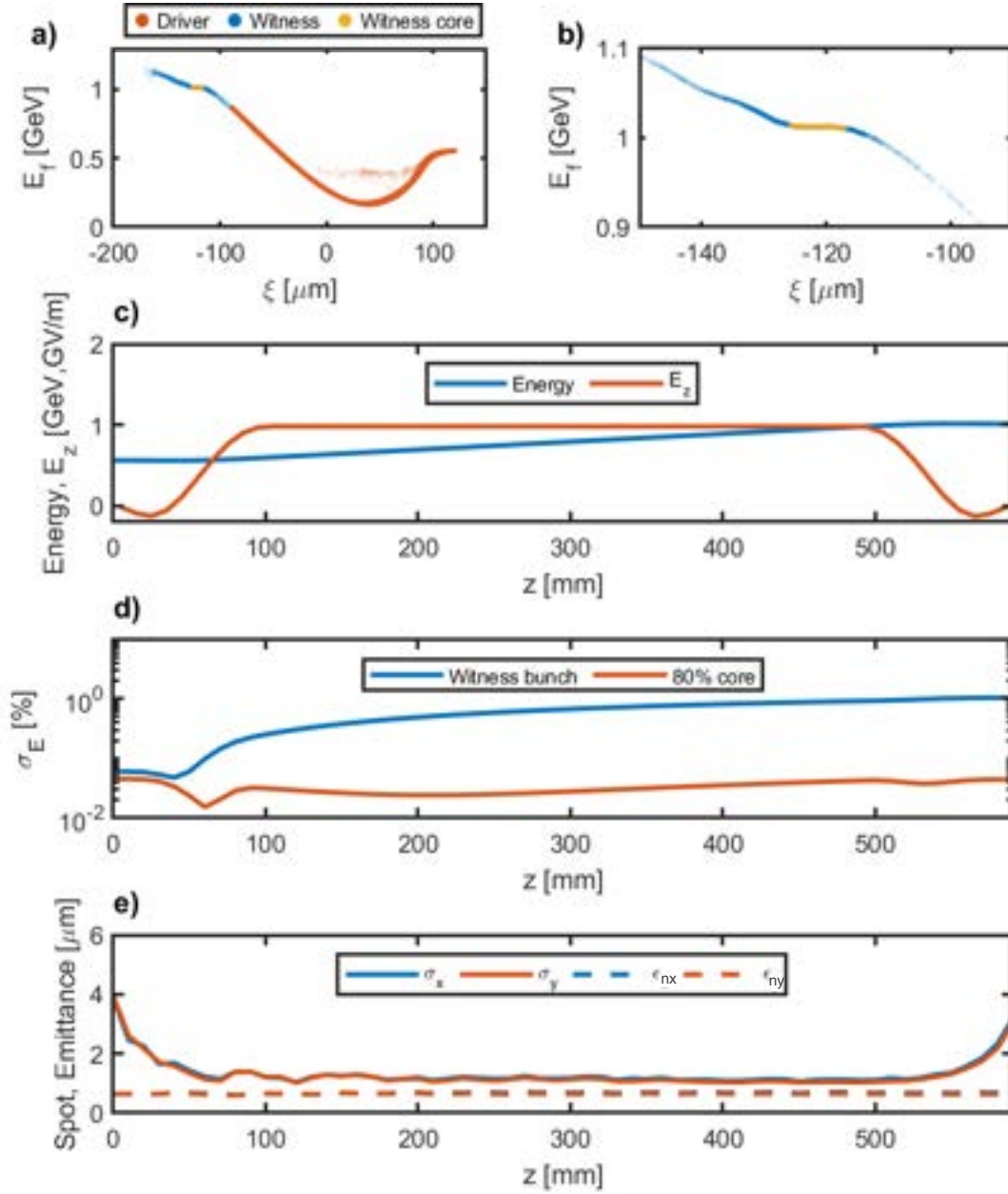
Figure 3.10: Longitudinal phase space of the driver and witness bunches (a) and of the witness only (b) at the end of the capillary. The coordinate \xi denotes the separation of the single particles respect to the position of the longitudinal centroid of the driver z . The witness energy evolution and its experienced accelerating gradient inside the plasma module are shown in (c), where a decelerating zone close to the capillary ends can be noticed, due to the fact that for low densities the witness is in the decelerating phase of the accelerating field. Energy spread evolution of the entire bunch and the witness core (d). Transverse size inside the capillary and normalized emittance evolution (e).
