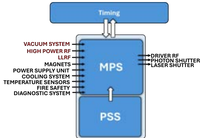
Figure 19.29: Overview of the devices and subsystems connected to the MPS, both for input, to read the interlocks, and for output, to enable or disable the systems. Critical subsystems that require a fast response to interlocks are highlighted in red.
