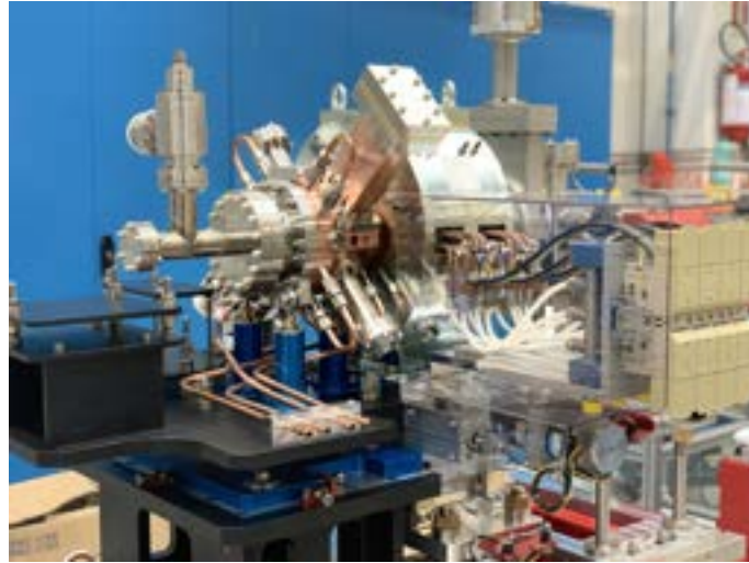
Figure 13.1: Picture of the S-band RF Gun realized for the CLEAR injector.
