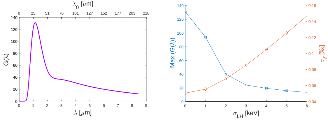
Figure 3.26: MBI spectral gain G = |b_f/b_0| . Left: spectral gain for the full RF -only magnetic- (250 pC). \lambda_0 and \lambda are the initial and compressed wavelength, respectively (two-stage magnetic compression). Right: peak spectral gain and respective \sigma_\delta as a function of the energy spread induced by the LH.
