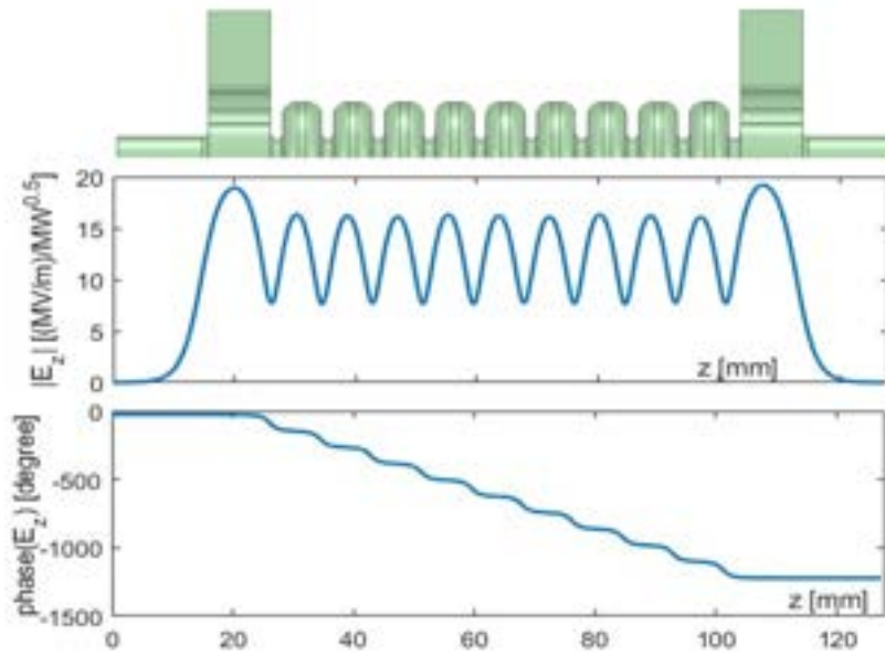
Figure 6.6: Amplitude and phase of the accelerating field along the structure (ANSYS-HFSS simulation result with a reduced number of cells, 9 instead of 113).
