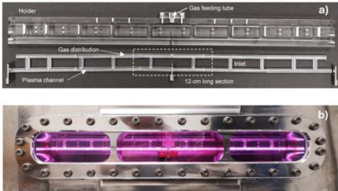
Figure 7.6: 60 cm-long gas-filled discharge capillary. a) Single components before the capillary assembly. b) Plasma discharge generated after the assembly.
