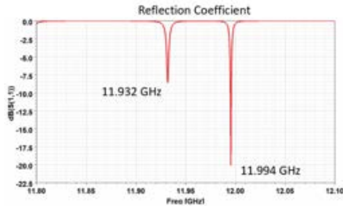
Figure 5.7: Reflection coefficient at the port of the input waveguide. The minimum is equal to -20 dB at the operation frequency. The mode separation is 62 MHz.
