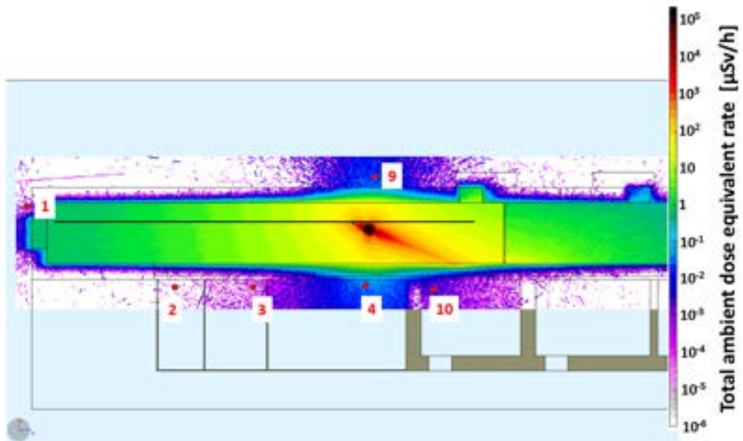
Figure 19.16: H^*(10) - 800 MeV diagnostic beam dump - xz plane.
