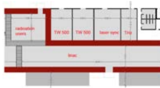
(a) Ground floor layout showing the room for the photocathode/synch laser.
