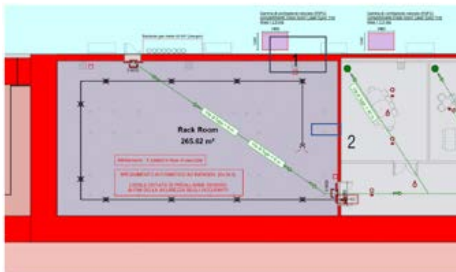
Figure 19.4: Example of first floor plan with identification of the area served by the automatic extinguishing system
