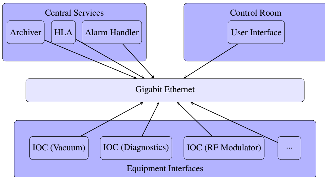
Figure 15.1: Three tier architecture scheme.
