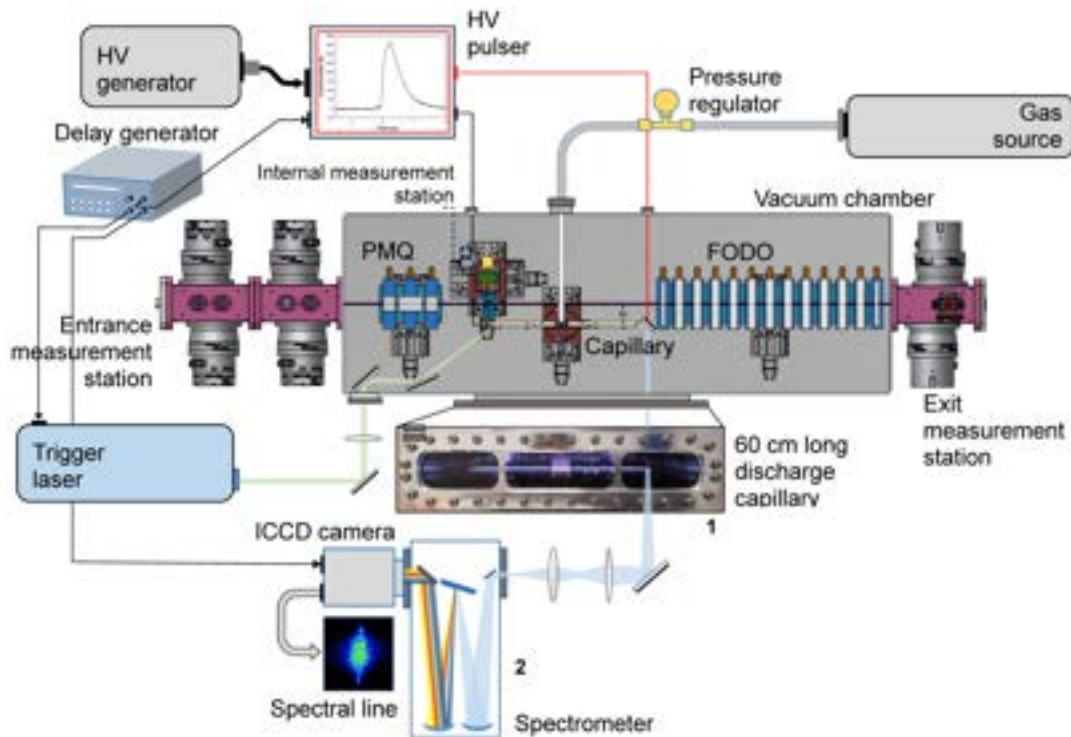
Figure 7.2: Schematic representation of the plasma module. A picture of a 60 cm long gas-filled discharge capillary (1) is shown in this scheme. The plasma diagnostics is based on the Stark broadening technique, for which the emitted plasma light is collected into an imaging spectrometer allowing to measure the spectral wavelengths of the hydrogen Balmer series (2).
