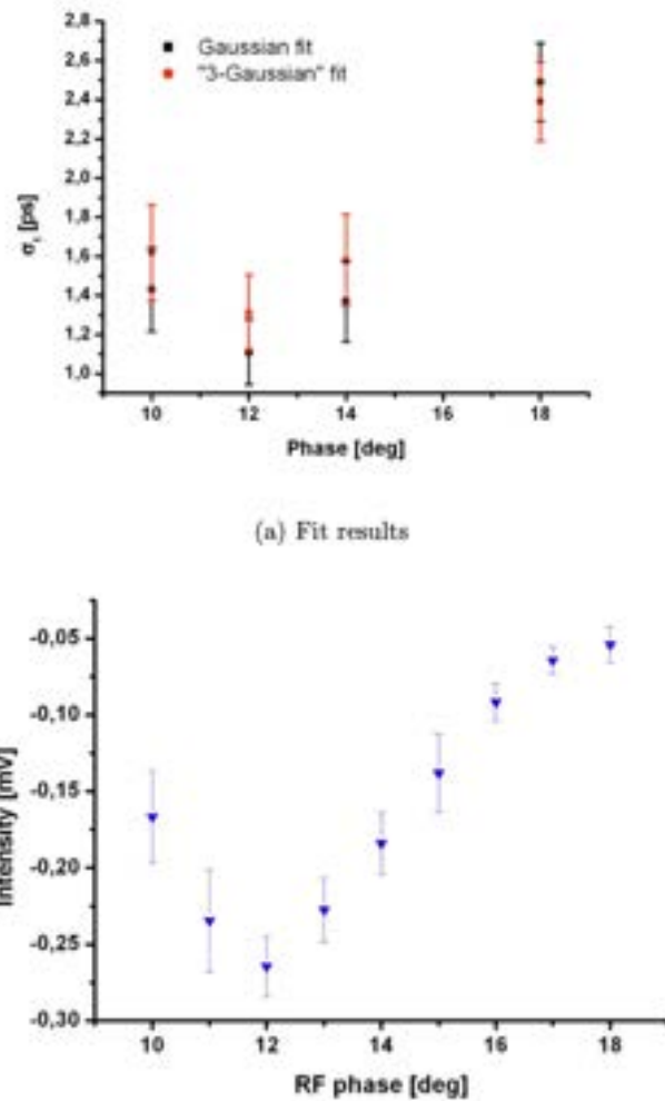
Figure 11.20: Top: bunch length, bottom: amplitude of the signal obtained from the CDR monitor as a function of phase compression at TTF VUV-FEL (DESY). From [37].
