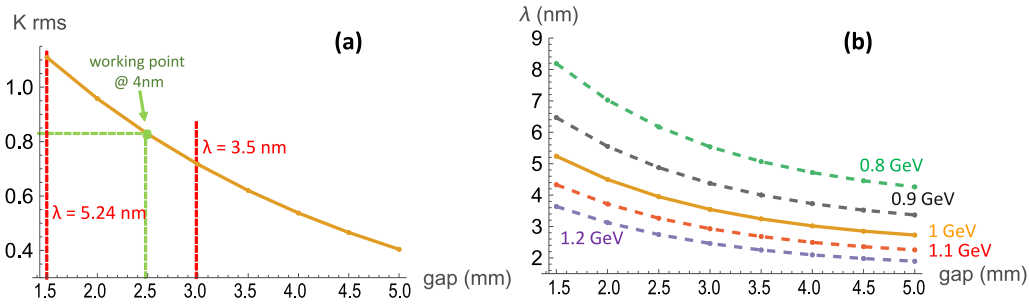
Figure 8.18: (a) K_{\text{rms}} variation vs gap and tuning range. Tuning range is the same for all operation modes of polarization. (b) Wavelength tuning range for different values of the e-beam energy; the continuous line stands for the reference case at 1 GeV.
