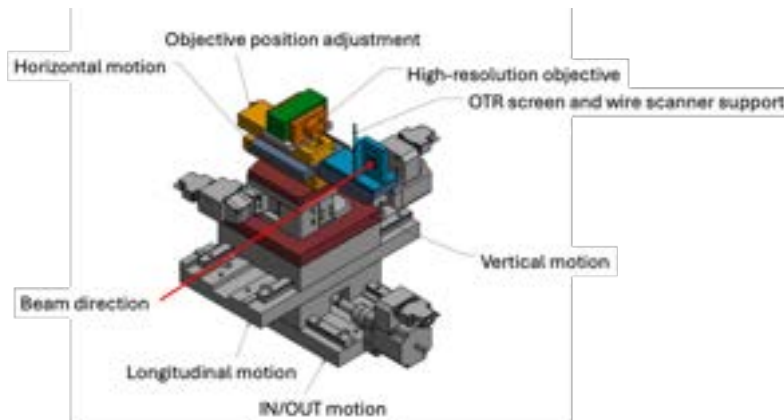
Figure 11.21: Axonometric projection of the diagnostic block at the entrance of the capillary. The beam direction is indicated by the red arrow.
