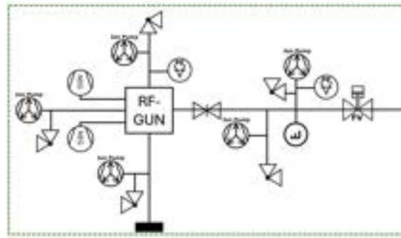
Figure 16.3: RF-gun Vacuum System: Schematic Layout
