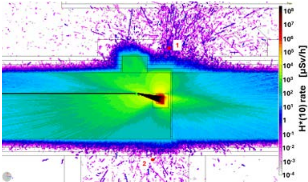
Figure 19.26: H^*(10) - driver beam dump - xz plane.
