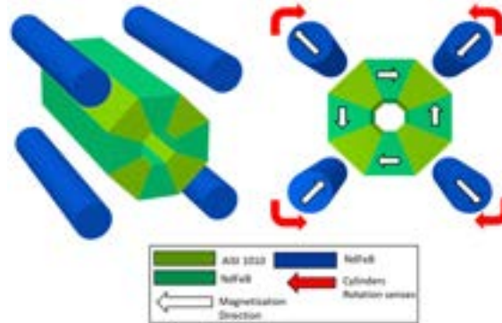
Figure 17.16: 3D view (left) and front view (right) of TPMQ. Legend of the blocks material, magnetization direction and cylinders rotation sense are shown (down).
