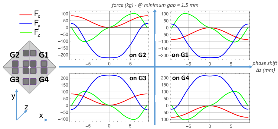
Figure 8.29: Integrated magnetic forces acting on the four undulator girders (G1, G2, G3, G4) in presence of the compensating magnets array.
