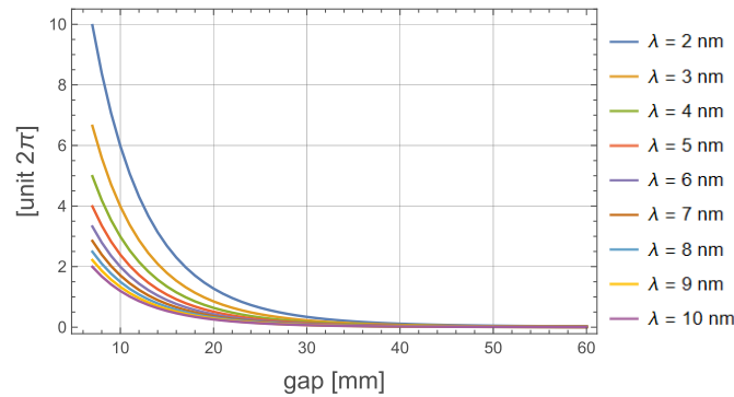
Figure 8.41: Phase correction as a function of the phase shifter gap, for different values of operational wavelength.
