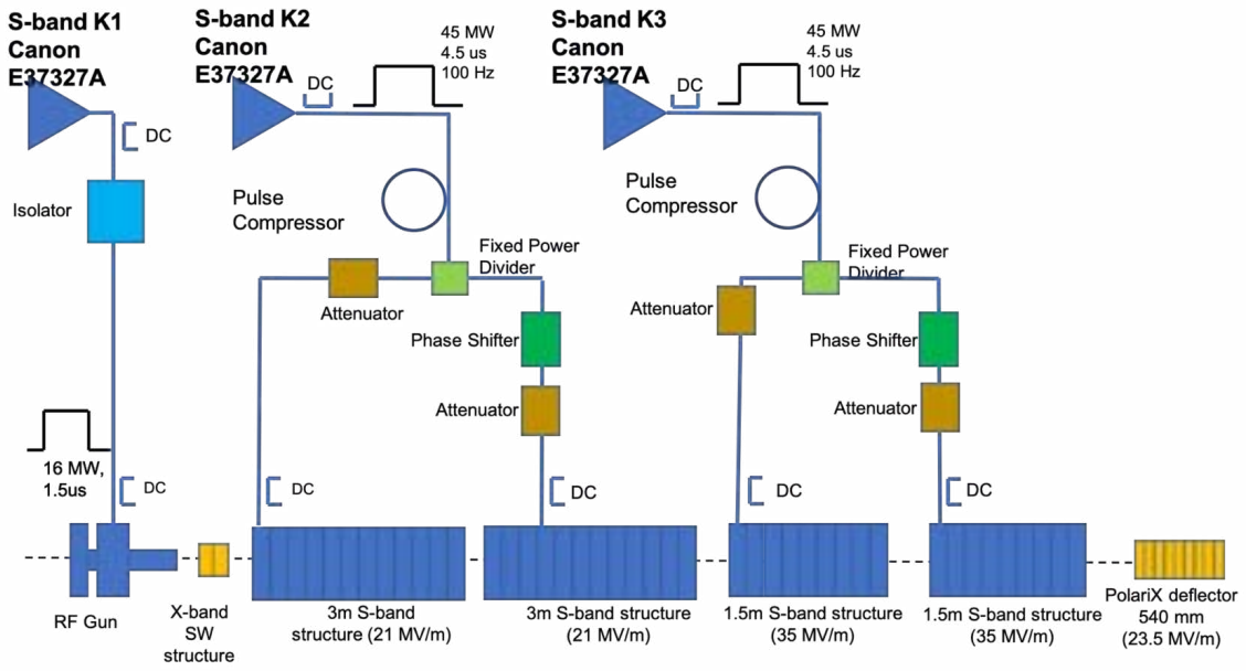
Figure 5.15: Layout for the S-band power distribution system taking into account the four S-band accelerating structures.
