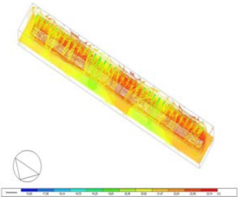
Figure 18.25: LINAC room Temperature simulation map.
