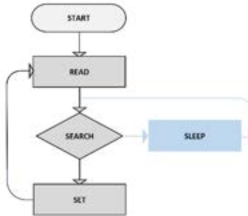
Figure 19.31: FPGA state machine implementing the read–search–set cycle used by the MPS, ensuring fail-safe operation and fast response to interlocks.
