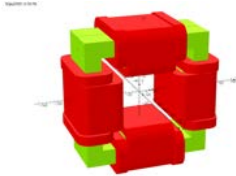
Figure 17.9: The 3D design of H-V steerer between accelerating sections.
