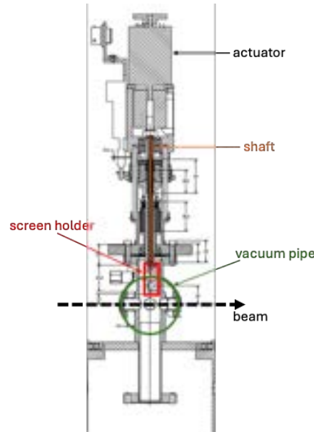
Figure 11.6: Mechanical drawing of the compact view screen, highlighting main components and beam propagation direction.
