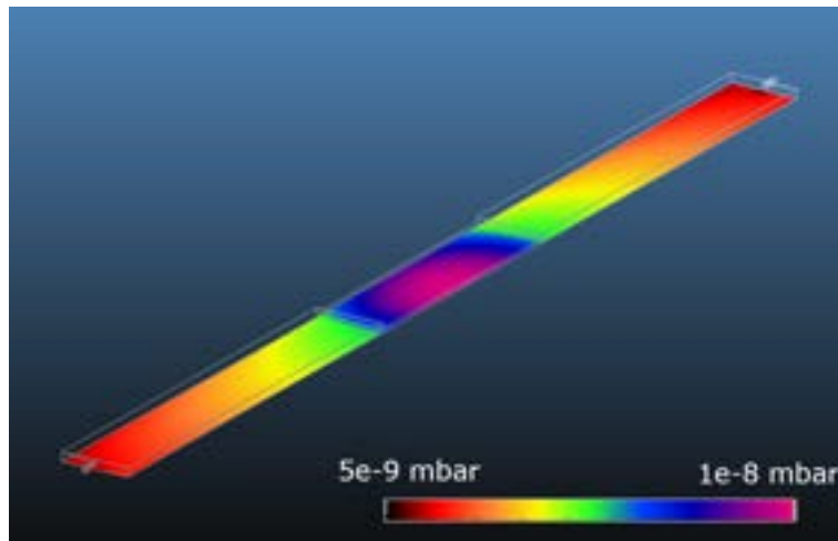
Figure 16.9: Laser Heater Chamber: Pressure simulation for a 100 l/s pumping system
