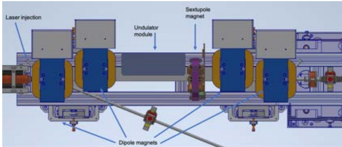
Figure 12.12: Schematic of the Laser Heater (LH) beamline.
