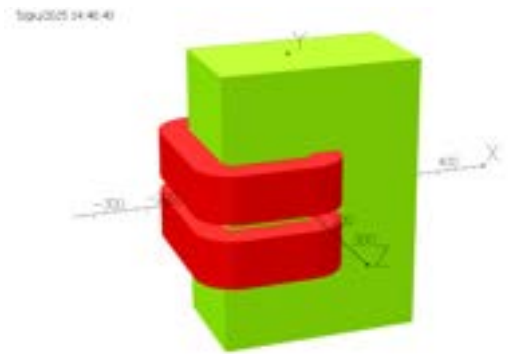
Figure 17.11: The 3D design of C-shaped dipoles for the Laser Heater chicane.
