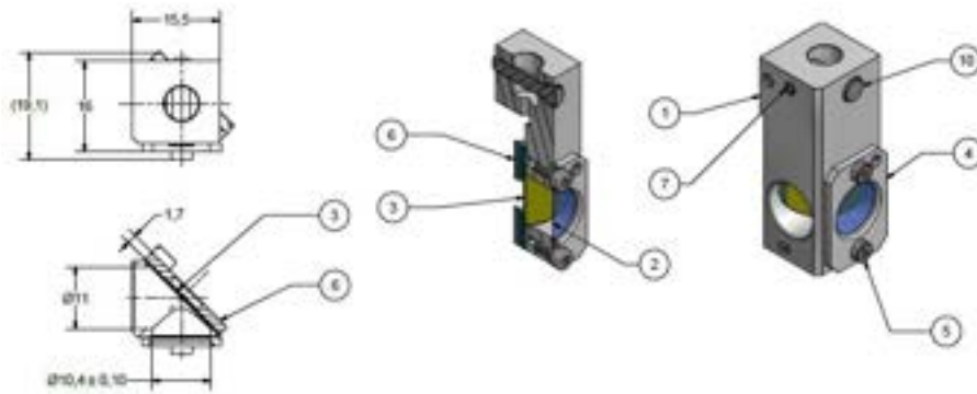
Figure 11.7: Mechanical drawing of the screen holder: 1) Base support; 2) Scintillator screen; 3) Mirror; 4) Scintillator casing; 6) Mirror casing; 7) Set screws with hex socket; 10) Plug.
