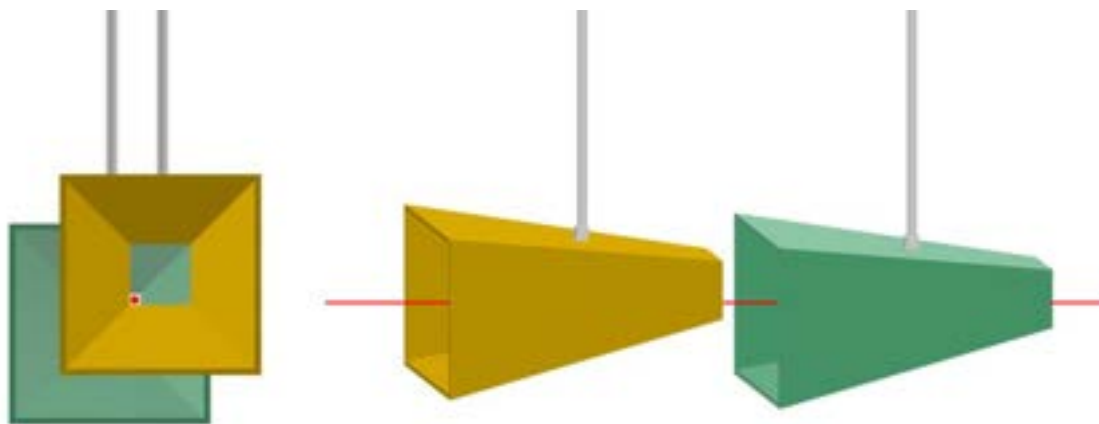
Figure 9.5: Schematic layout of the two consecutive truncated pyramids forming the BDA. Left: frontal view; right: side view. The red line represents the photon beam.
