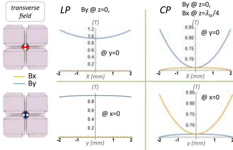
Figure 8.20: Transverse field profile of the AQUA undulator in Linear (LP) and Circular (CP) polarization.
