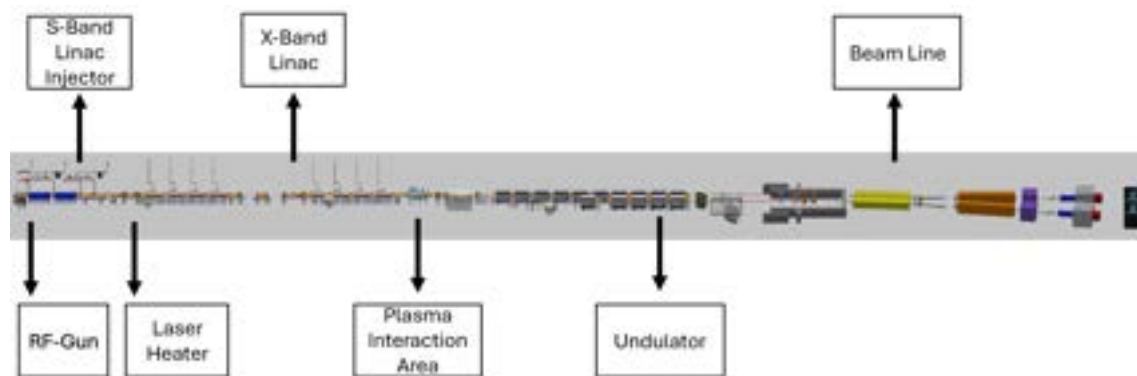
Figure 16.1: Vacuum Schematic Layout Legend
