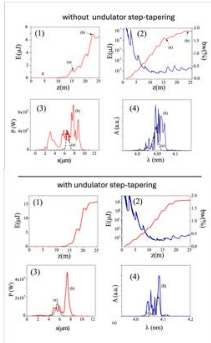
Figure 3.14: FEL simulation results for PWFA nominal working point. Top: case without tapering. Bottom: case with tapering, the corresponding values of the undulator parameters along the line are given in Table 3.8. Picture (1): energy growth in linear scale. Picture (2): energy growth in logarithmic scale and bandwidth in %. Picture (3): power distribution at (a) 17 m and (b) 25 m along the undulator ( s = z - 17 m and s = z - 25 m respectively) Picture (4): spectral distribution at (a) 17 m and (b) 25 m along the undulator.
