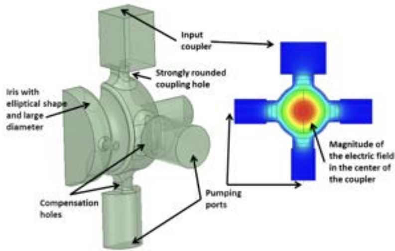
Figure 5.3: Electromagnetic model of the RF gun.
