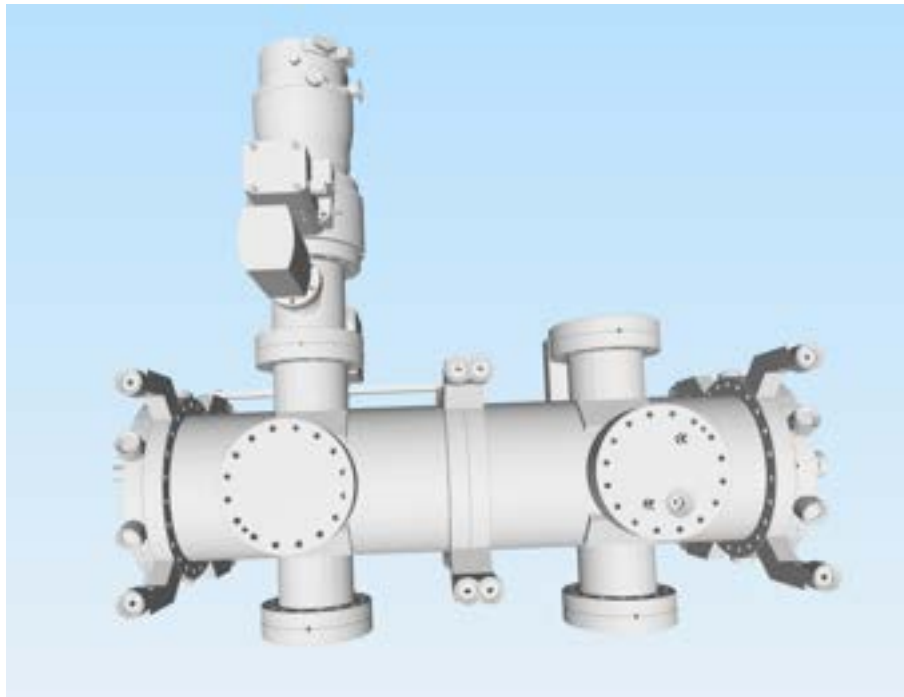
Figure 9.13: Draft of the GMD, Courtesy of Dr. K. Tiedke, Photon Diagnostic Team DESY, Hamburg.
