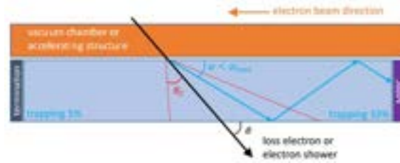
Figure 11.24: Cherenkov light produced by a lost electron is captured by an optical fiber. When the Cherenkov condition is satisfied, UV radiation propagates along the fiber under appropriate conditions.
