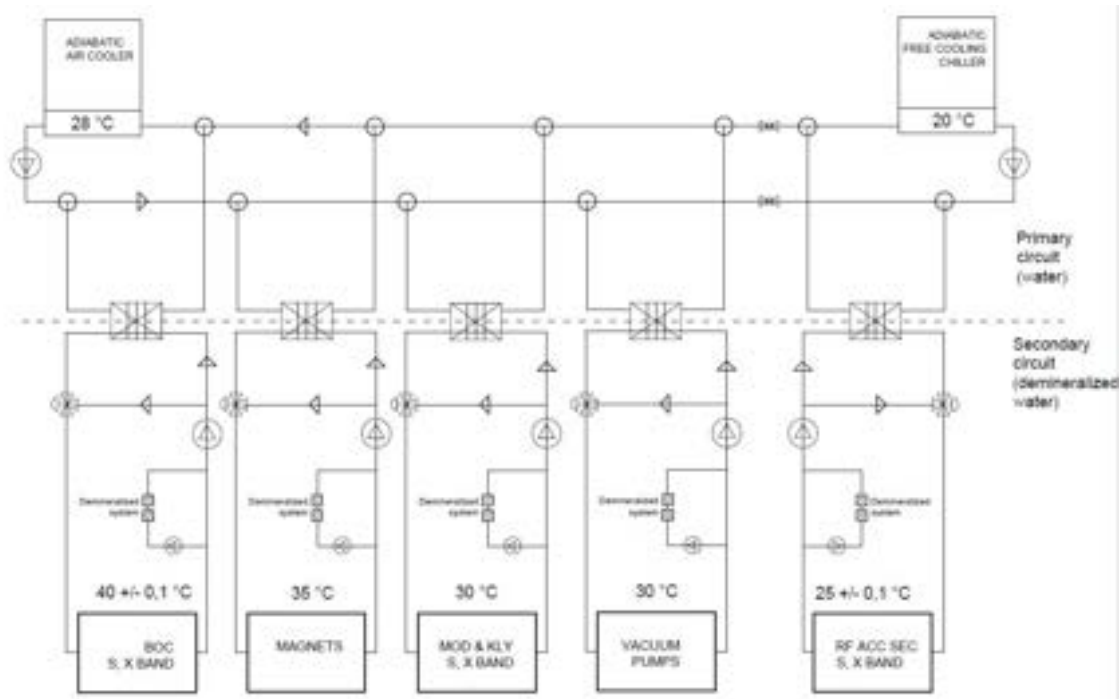
Figure 18.15: Cooling System Schematic.
