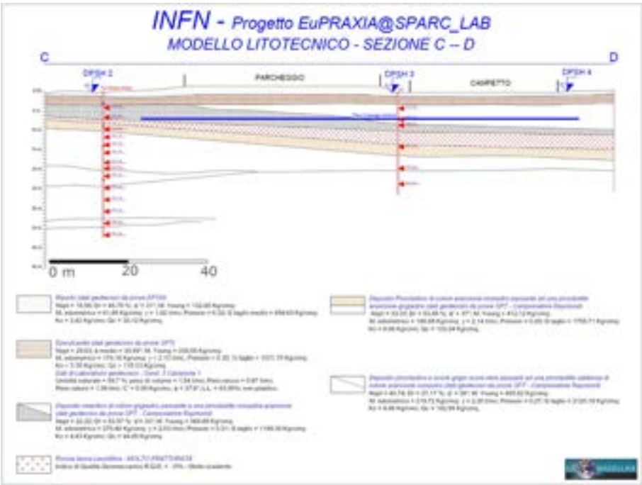
Figure 18.2: Excerpt from the geological report: stratigraphic section of the soil in longitudinal direction.
