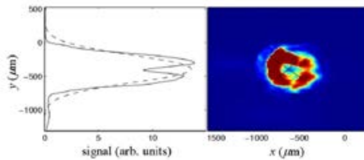
Figure 11.8: Example of a particle beam image in the presence of COTR [8].
