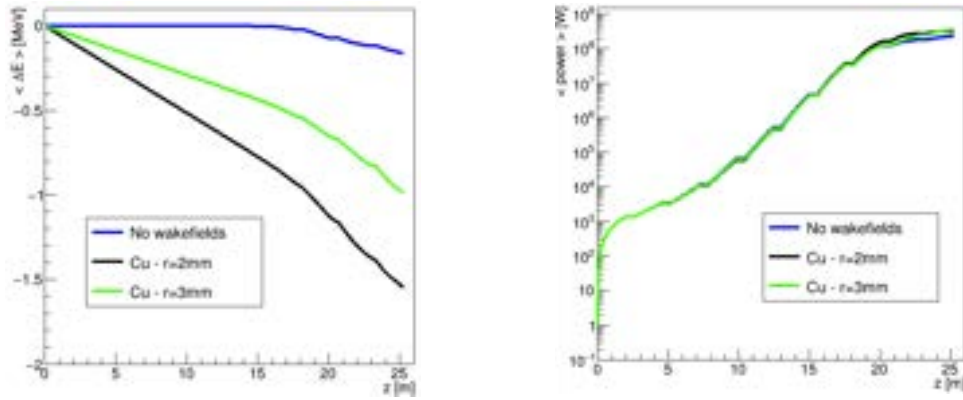
Figure 8.46: Electron bunch with 30 pC charge and 2 \mu\text{m} RMS length. Average energy loss (left) and average FEL output power (right) as a function of the propagation coordinate for VC inner radius of 2 mm (black) and 3 mm (green), compared with the no wakefield effects case (blue).
