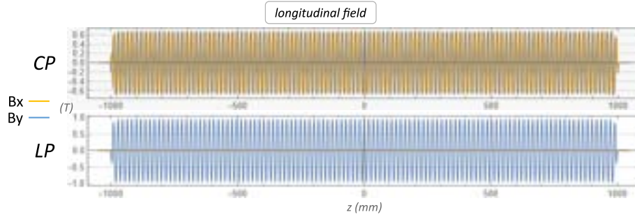
Figure 8.19: Longitudinal field profile of the AQUA undulator in Linear (LP) and Circular (CP) polarization.
