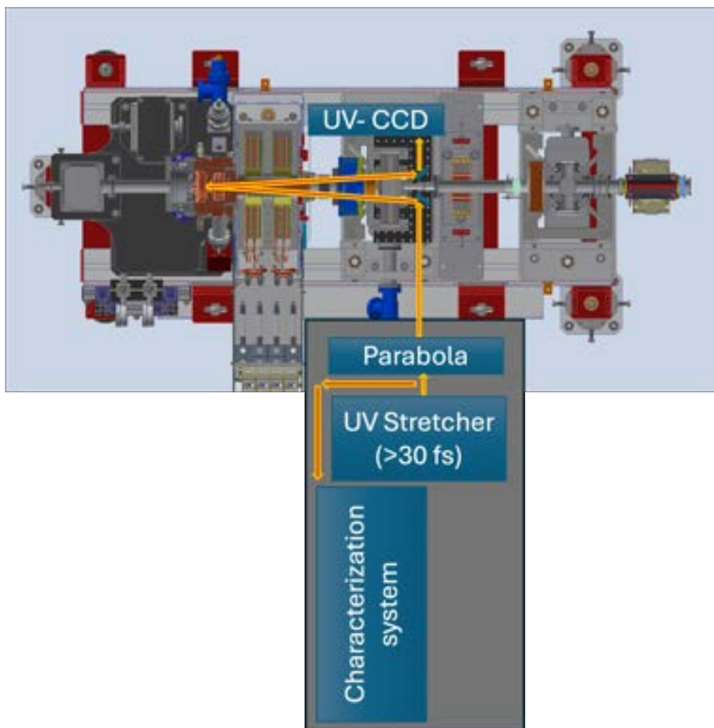
Figure 12.11: Top view of the gun and associated diagnostics.
