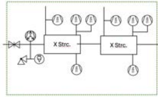
Figure 16.11: X-Band Linac Module: Vacuum Schematic Layout
