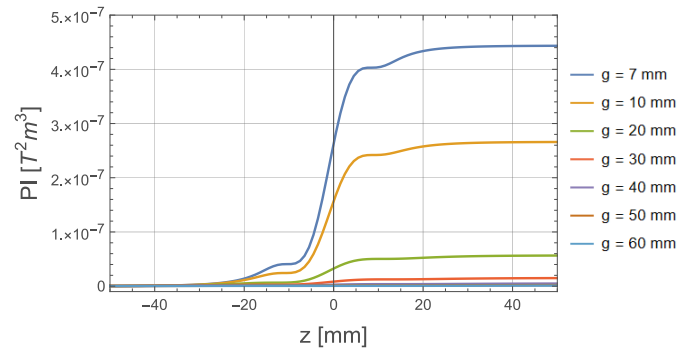
Figure 8.40: Phase Integral (PI) in the phase shifter for different values of the operational phase shifter gap.
