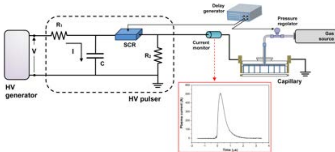
Figure 7.14: High-voltage source designed for plasma creation inside gas-discharge-filled capillaries. There are three different parts: the high-voltage generator that supplies power to a pulser consisting of an RC circuit that, in turn, is capable of producing high-repetition frequency current pulses (100-400 Hz) and a load represented by the plasma source.
