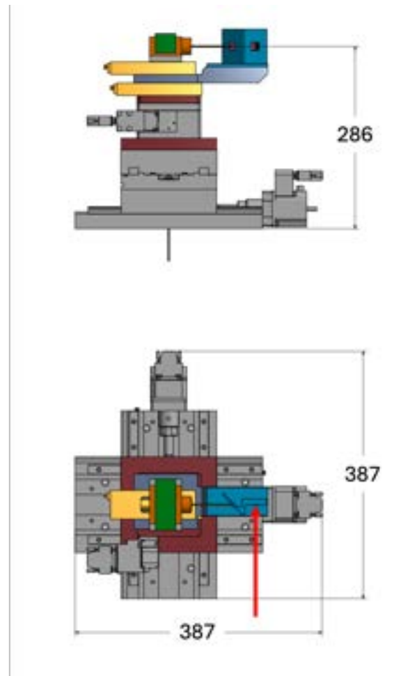
Figure 11.22: Design of the plasma entrance diagnostic device. Top: front view, with beam direction through the page. Bottom: top view, with beam direction indicated by the red arrow. Blue: holder containing the OTR screen (rotated at 45^\circ with respect to the beam) and the microwires. Grey: remotely controlled translation stages for in-out and longitudinal motion, and for fine adjustment of the vertical and horizontal positions for microwire scans. Orange: microscopic objective. Yellow: translation stage for precise objective positioning. Dimensions in mm.
