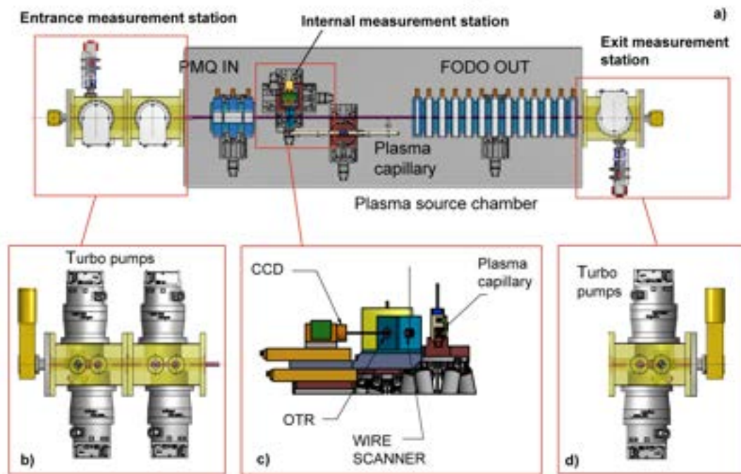
Figure 7.22: a) Top view of the layout of the beam diagnostics provided in the plasma source housing chamber area. b) Side view of the chamber housing the incoming beam diagnostics. c) Side view of the diagnostics of the beam entering the capillary. d) Side view of the chamber housing the outgoing beam diagnostics.
