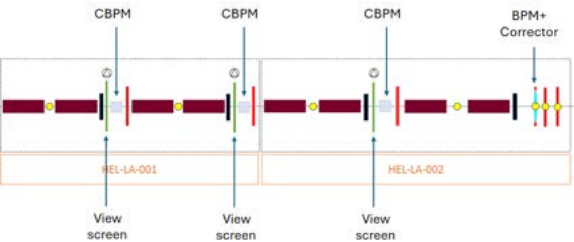
Figure 11.36: Diagnostics positions in the high energy linac.
