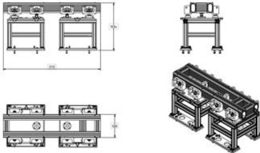
Figure 6.18: Girder of the X-band module supporting the two X-band structures and components.
