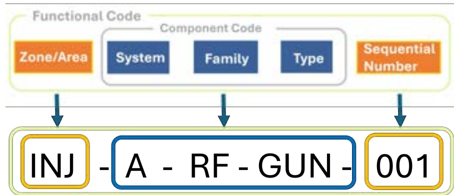
Figure 20.6: Identification code of the GUN on the beamline of EuPRAXIA@SPARC_LAB.
