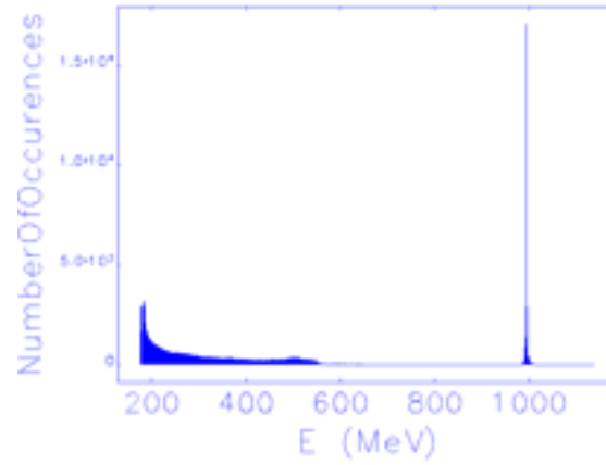
Figure 3.11: Energy distribution of the comb beam at the plasma exit: the witness bunch is located around the 1 GeV peak, while most of the driver particles are distributed between 200 and 500 MeV
