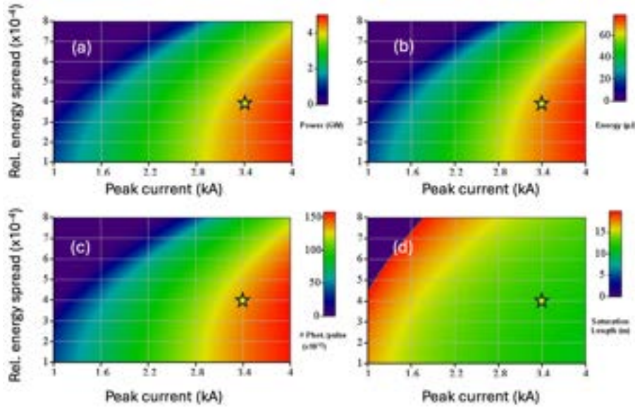
Figure 8.9: The four panels represent the dependence of the peak power (a), the pulse energy (b), the number of photons per pulse (c) and the saturation length (d) as functions of both the slice beam relative energy spread and the peak current. The undulator is in circular polarisation. The yellow star symbol indicate the working point simulated in the beam physics chapter, Tab. 3.1.
