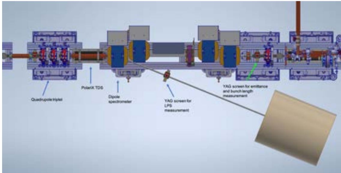
Figure 5.18: Layout of the high energy injector diagnostic.
