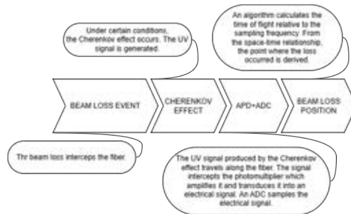
Figure 11.30: Description of the detection flow of Cherenkov BLM.
