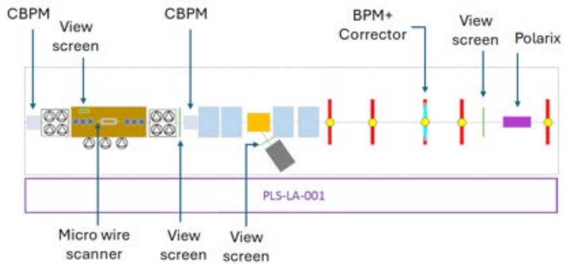
Figure 11.37: Diagnostics position in the plasma module. The view screen and the microwire scanner will be inserted in the beam line in alternation with permanent magnets and the plasma capillary, respectively.
