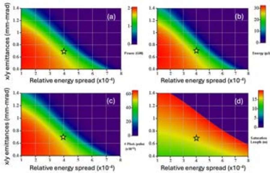
Figure 8.5: The four panels represent the dependence of the peak power (a), the pulse energy (b), the number of photons per pulse (c) and the saturation length (d) as functions of both the slice normalised beam emittances and the energy spread. The undulator is in circular polarisation. The yellow star symbol indicate energy spread and emittances of the working point simulated in the beam physics, Tab. 3.1. Note that the simulated working point presents a substantially higher peak current with respect to the conservative value used in this example (3.3-3.4 kA vs 1.5 kA).
