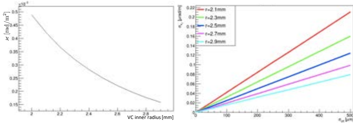
Figure 8.51: Left: kick parameter per unit length per transverse offset as a function of the vacuum chamber inner radius. Right: uncertainty in the kick angle per unit length as a function of the misalignment jitter value, for different vacuum chamber inner radii.
