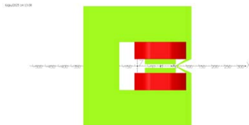
Figure 17.21: The section of the septum dipole.
