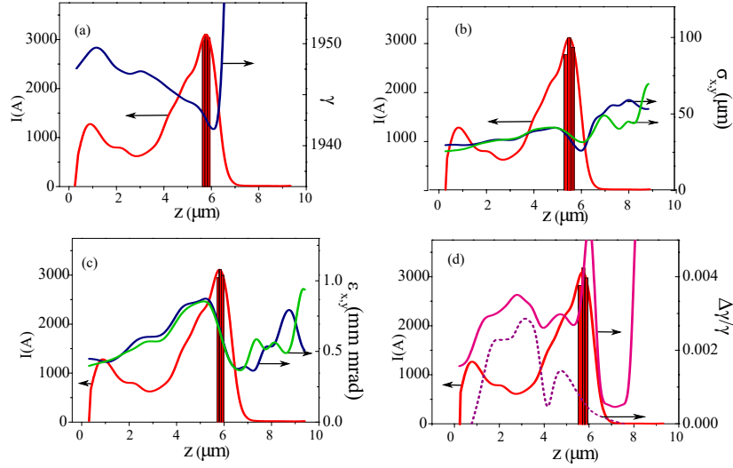
Figure 3.13: Slice analysis of the electron beam in the undulator: Beam current in red on the left axis in all the figures as function of the beam coordinate z(\mu\text{m}) . The red columns indicate the best slices in terms of radiation brilliance. On the right axes, (a) Lorentz factor \gamma (blue curve), (b) x and y rms dimensions \sigma_x and \sigma_y (green and blue curve respectively), (c) x and y normalized emittance \varepsilon_{nx} and \varepsilon_{ny} (green and blue curve respectively), and (d) the relative energy spread \Delta\gamma/\gamma for the whole beam (magenta solid line) and with a cut of 5% of charge (magenta dotted line).
