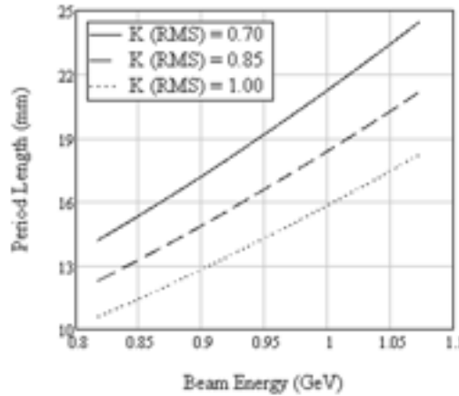
Figure 8.1: Relation between the beam energy and the undulator period ensuring the undulator resonance at the carbon K-edge (300 eV).
