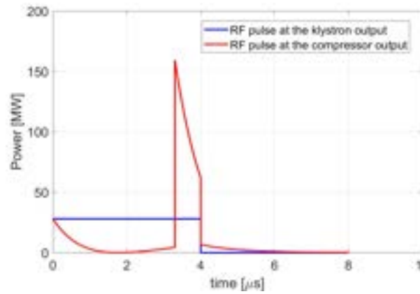
Figure 13.4: Computed RF pulses at the SLED input and output for the 1.5 m S-band structures.
