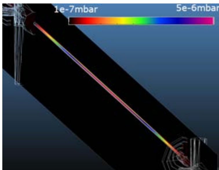
Figure 16.18: Undulators: Detail of pressure distribution inside one of the Undulator vacuum chamber
