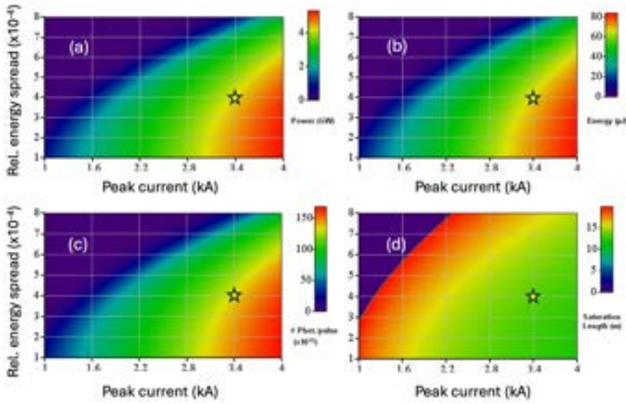
Figure 8.10: As in Fig. 8.9, the four panels represent the dependence of the peak power (a), the pulse energy (b), the number of photons per pulse (c) and the saturation length (d) as functions of both the slice beam relative energy spread and the peak current, but with the undulator in linear polarisation. The yellow star symbol indicate the working point simulated in the beam physics chapter, Tab. 3.1.
