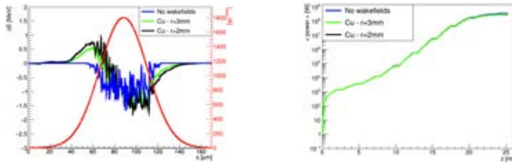
Figure 8.47: Electron bunch with 300 pC charge and 20 \mu\text{m} RMS length. Energy loss at undulator exit superimposed to the current profile (left frame) and average FEL output power along the propagation coordinate (right frame) for VC inner radius of 2 mm (black) and 3 mm (green), compared with the no wakefield effects case (blue).
