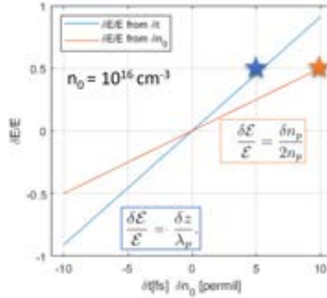
Figure 3.15: Analytical evaluation of the plasma vs the linac contribution to energy gain jitter at the plasma exit [7]. The stars represent the contribution to the energy spread due to the 5 fs jitter of the witness and driver temporal separation (blue) and the contribution due to the 1% plasma density variation (orange)
