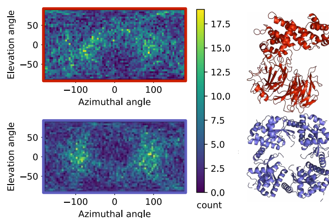
Figure 2.4: Simulated CEI footprints under AQUA beamline experimental conditions. Simulations were performed using the MOLDSTRUCT software [68] for two proteins of similar mass: one originating from the cell nucleus (Nucleoporin, PDB ID: 4mhc [69], shown in red) and one derived from a virus (avian influenza virus PA N Apo, PDB ID: 4e5e [70], shown in blue). Differences between the footprints enable clear differentiation of the two proteins upon explosion. Image adapted from [71].
