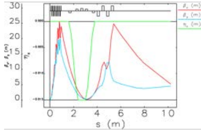
Figure 3.12: Twiss parameters of the witness along the capture/separation transfer line between the plasma capillary exit and the undulator entrance.
