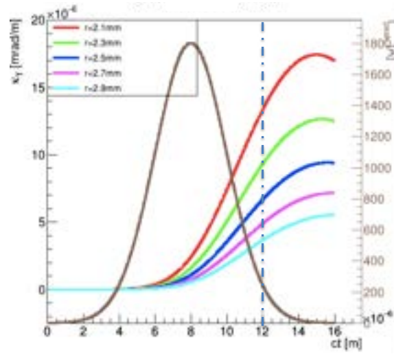
Figure 8.48: Kick angle per unit length for different vacuum chamber inner radii, and for a transverse offset of 50 \mu\text{m} , superimposed to the short bunch current profile (brown curve).
