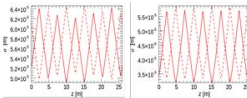
Figure 8.43: Electron beam RMS matched transverse size \sigma_{x,y} (m) along the AQUA undulator coordinate z (m) in circular polarization. Nominal case with \beta_T = 8 m (left) for quadrupole field gradients 5.6/-5.5 T/m, and case with \beta_T = 5 m (right) for quadrupole field gradients 12.5/-12 T/m. Solid lines \sigma_x , dashed lines \sigma_y .
