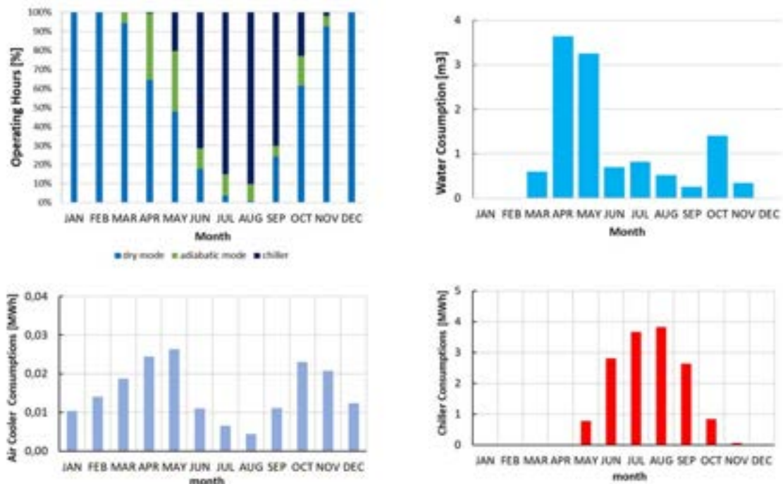
Figure 18.17: Top-left: Monthly operating hours of the chiller in free cooling dry mode, adiabatic mode, and chiller-only mode; Top-right: Monthly water consumption of the chiller in adiabatic mode; Bottom-left: Monthly electrical consumption of the chiller in free cooling mode; Bottom-right: Monthly electrical consumption in only chiller mode.
